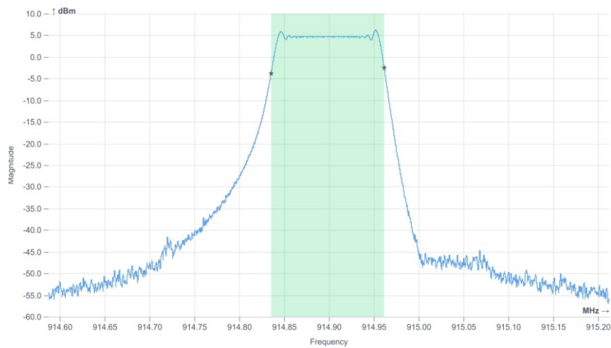
Plot 6: high channel, 99%OBW
