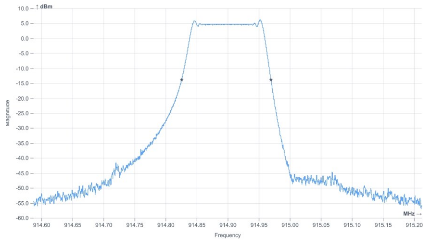
Plot 5: high channel, 20 dB-BW
