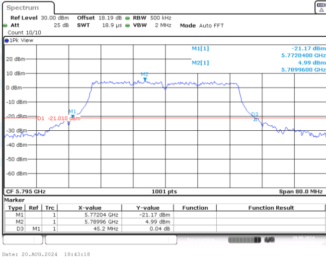
11N40SISO-Ant3-5795
