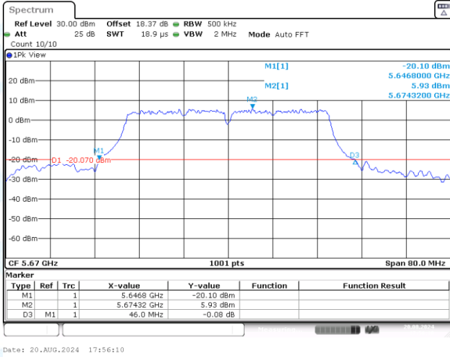
11N40SISO-Ant3-5670
