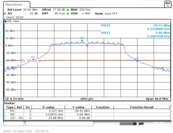
11AC20SISO-Ant3-5240
