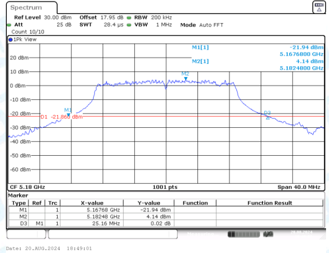
11AC20SISO-Ant3-5180
