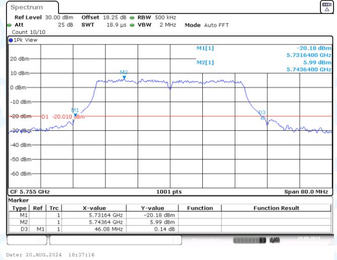
11N40SISO-Ant3-5755
