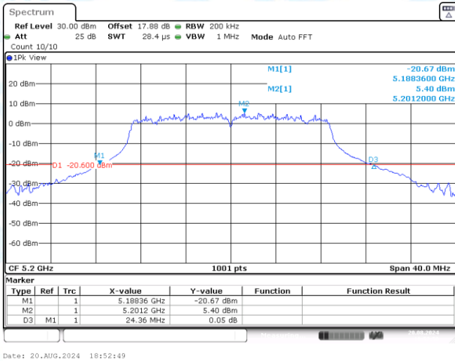
11AC20SISO-Ant3-5200
