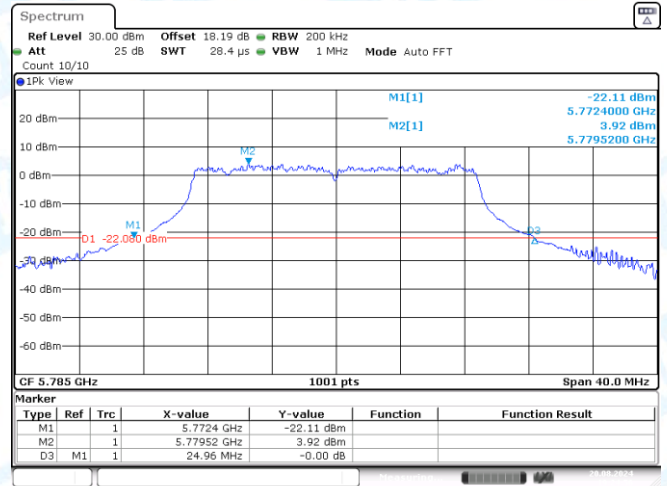
11AC20SISO-Ant3-5785
