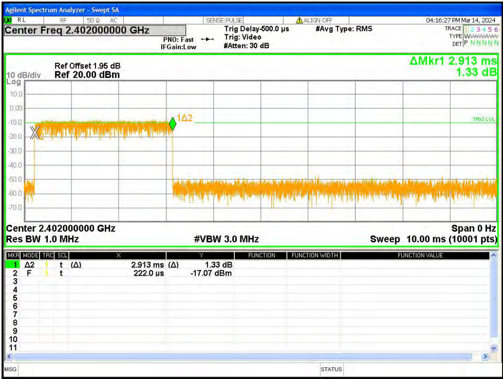
Dwell NVNT DH5 2402MHz Ant1 One Burst
