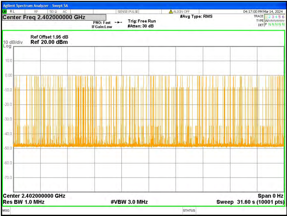
Dwell NVNT DH5 2402MHz Ant1 Accumulated
