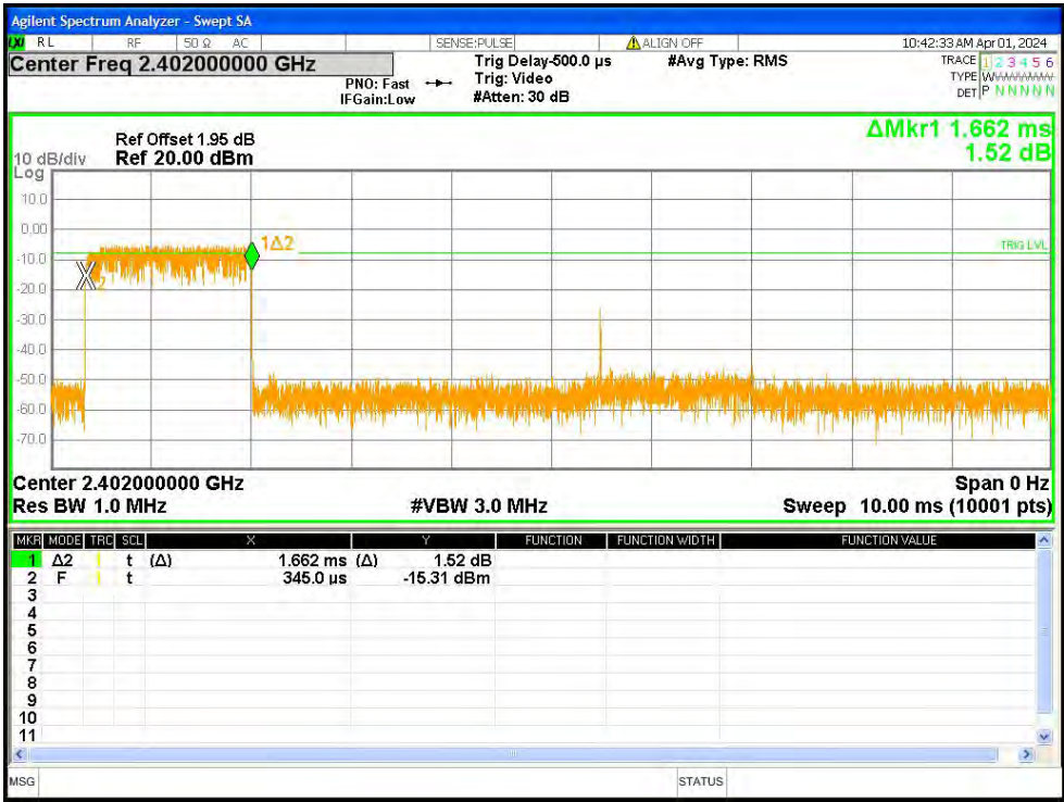
Dwell NVNT 3-DH3 2402MHz Ant1 One Burst
