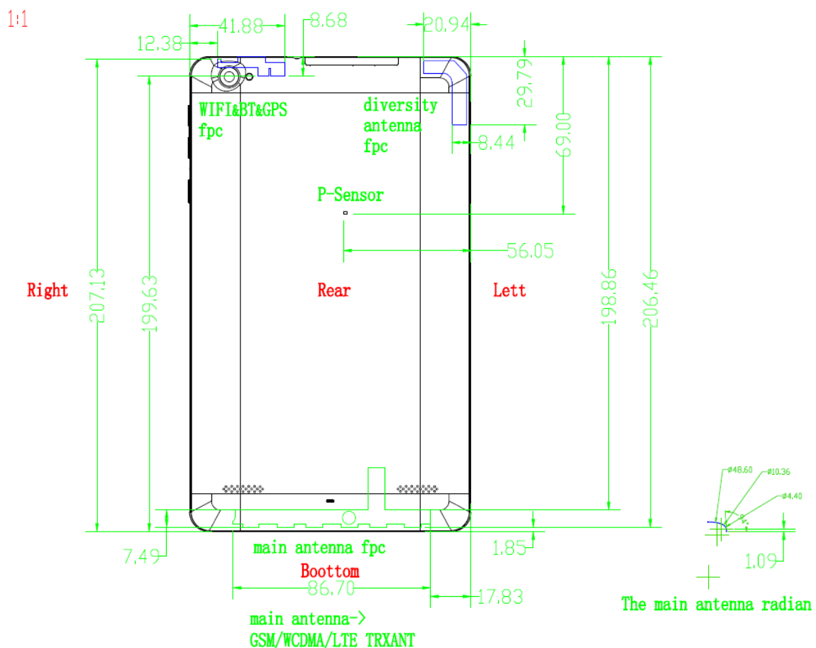
Fig.14.1 EUT Antenna Locations
