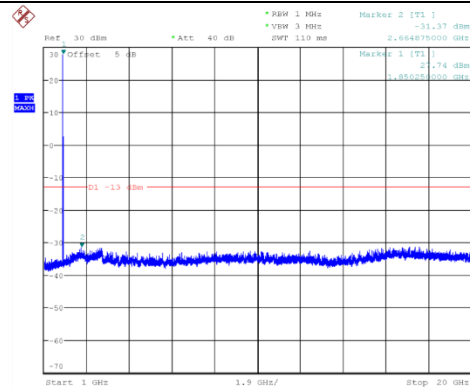
Channel 512: 1GHz~20GHz
