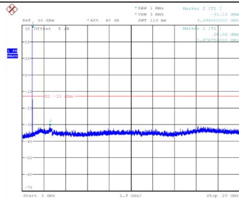
Channel 661: 1GHz~20GHz
