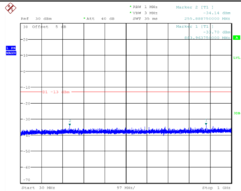
Channel 512: 30MHz~1GHz
