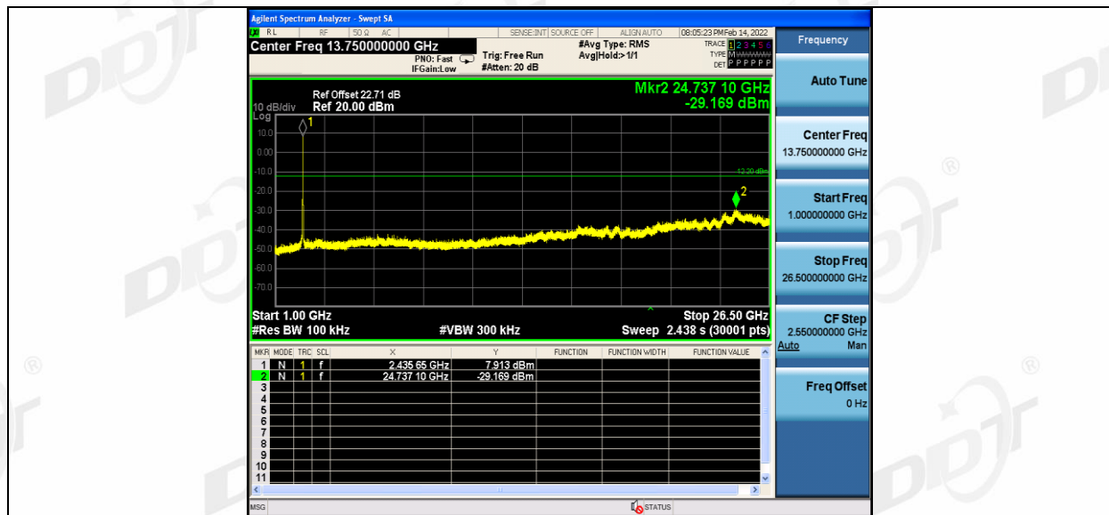
11AX20SU Ant2 2437 0-Reference
