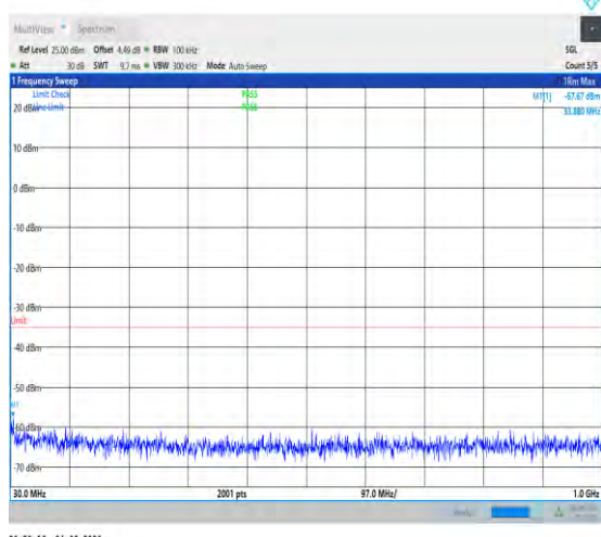
1-N7-PC3-15-40-H-1-DFT-PI2BPSK-Inner_1RB_Lef t-1@1-30-1000-Ant5-33.88--57.67--35-PASS
