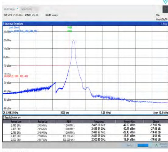
1-N7-PC3-15-5-L-4-CP-QPSK-Edge_1RB_Left-1@0-Ant5-1--PASS-see graph
