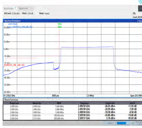
1-N7-PC3-15-10-L-6-CP-QPSK-Outer_Full-52@0-Ant5-1--PASS-see graph
