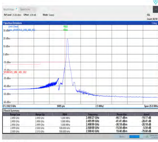
1-N7-PC3-15-10-L-4-CP-QPSK-Edge_1RB_Left-1@0-Ant5-1--PASS-see graph
