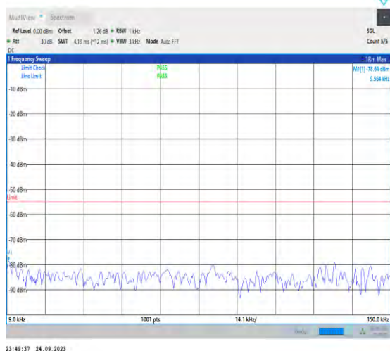
1-N7-PC3-15-40-L-1-DFT-PI2BPSK-Inner_1RB_Left -1@1-0.009-0.15-Ant5-0.01--78.64--55-PASS
