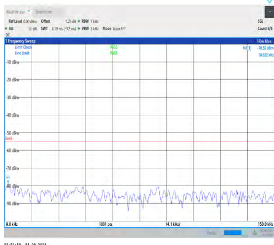
1-N7-PC3-15-40-H-1-DFT-PI2BPSK-Inner_1RB_Lef t-1@1-0.009-0.15-Ant5-0.01--78.55--55-PASS
