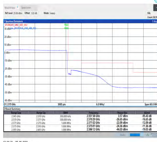
1-N7-PC3-15-25-H-6-CP-QPSK-Outer_Full-133@0-Ant5-1--PASS-see graph
