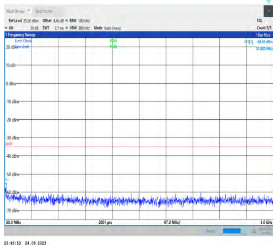
1-N7-PC3-15-40-L-1-DFT-PI2BPSK-Inner_1RB_Left -1@1-30-1000-Ant5-34.85--56.45--35-PASS
