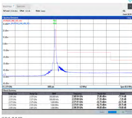
1-N7-PC3-15-25-H-5-CP-QPSK-Edge_1RB_Right-1@132-Ant5-1--PASS-see graph
