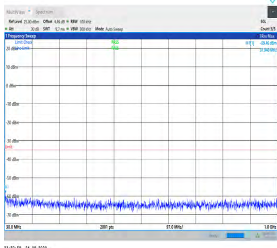
1-N7-PC3-15-40-M-1-DFT-PI2BPSK-Inner_1RB_Lef t-1@1-30-1000-Ant5-31.94--58.46--35-PASS
