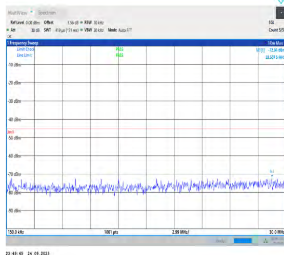
1-N7-PC3-15-40-L-1-DFT-PI2BPSK-Inner_1RB_Left- 1@1-0.15-30-Ant5-28.51--72.04--45-PASS
