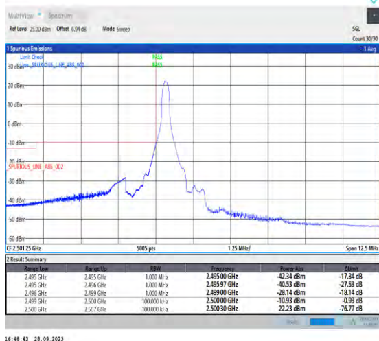
1-N7-PC3-15-5-L-1-DFT-PI2BPSK-Edge_1RB_Left-1@0-Ant5-1--PASS-see graph
