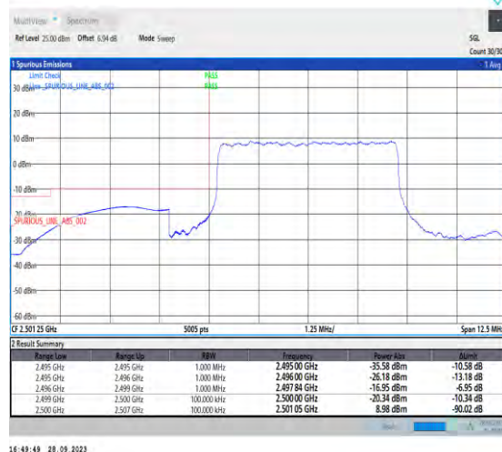
1-N7-PC3-15-5-L-3-DFT-PI2BPSK-Outer_Full-25@0-Ant5-1--PASS-see graph
