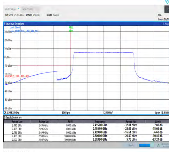
1-N7-PC3-15-5-L-6-CP-QPSK-Outer_Full-25@0-Ant5-1--PASS-see graph
