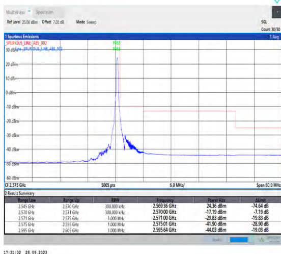
1-N7-PC3-15-25-H-2-DFT-PI2BPSK-Edge_1RB_Right-1@132-Ant5-1--PASS-see graph
