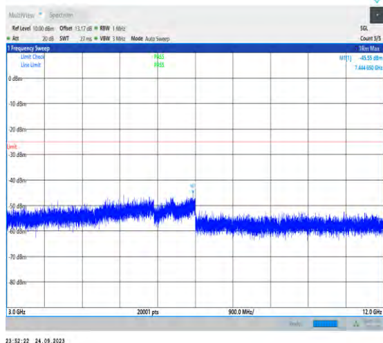
1-N7-PC3-15-40-H-1-DFT-PI2BPSK-Inner_1RB_Lef t-1@1-3000-12000-Ant5-7444.65--45.55--25-PASS
