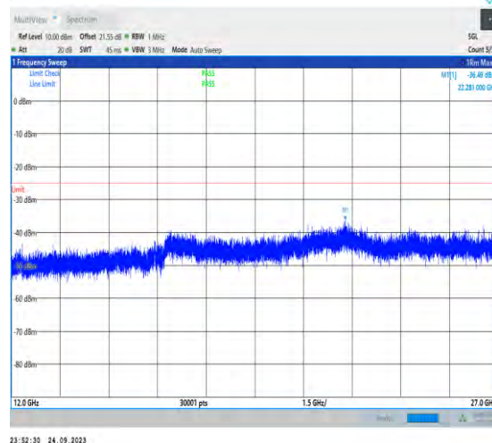
1-N7-PC3-15-40-H-1-DFT-PI2BPSK-Inner_1RB_Left- 1@1-12000-27000-Ant5-22281.00--36.49--25-PASS
