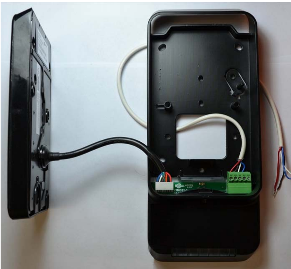
T21 Mifare Reader Assembly
