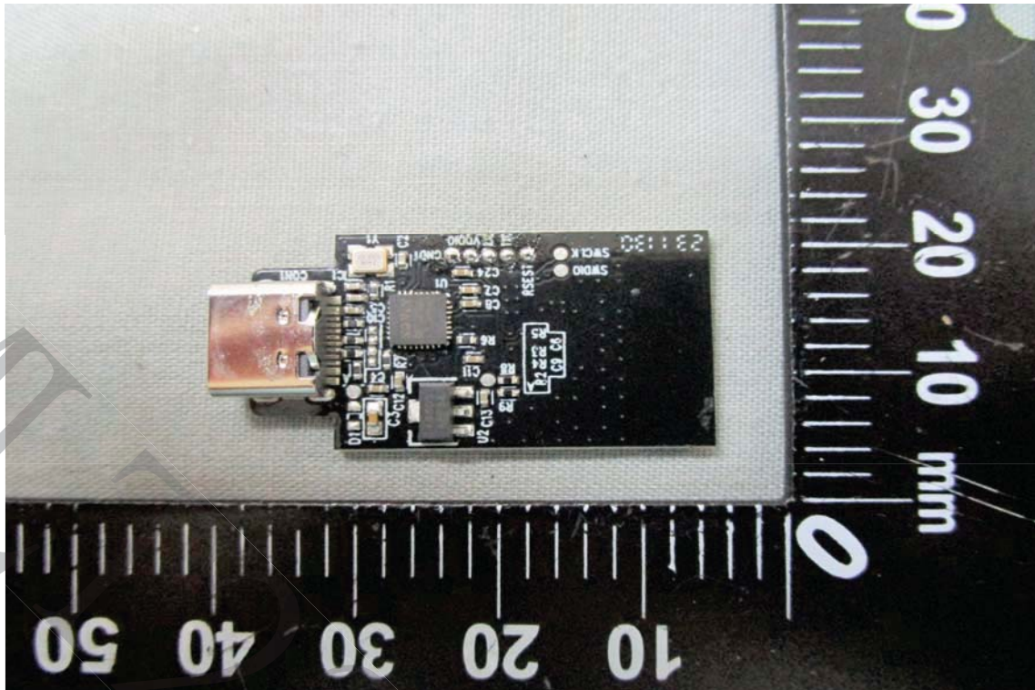
< PCB-R >
