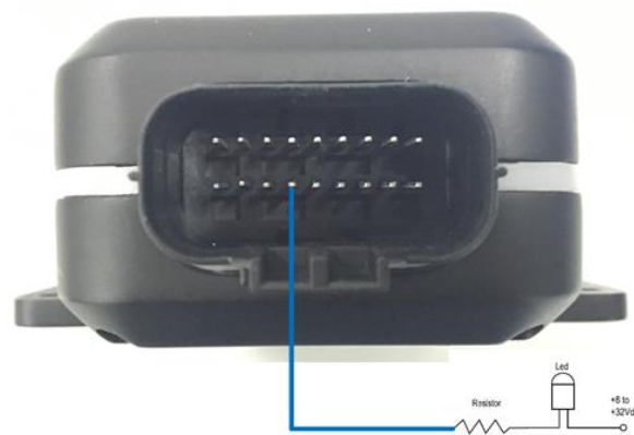
Figure 10. Typical Connection with a LED
