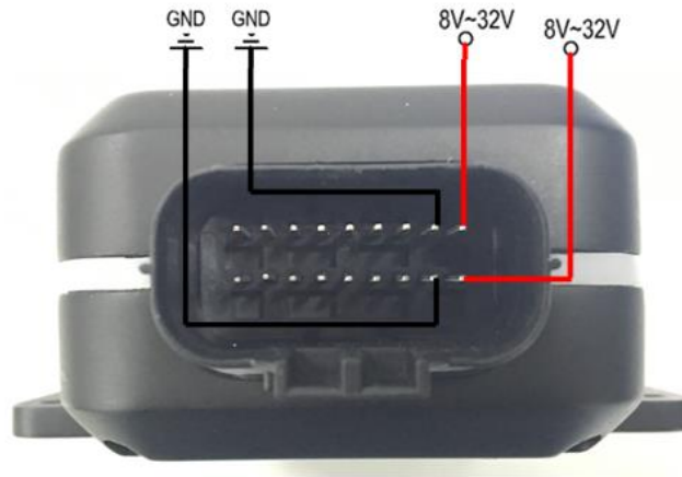
Figure 4. External Power Supply Connection
