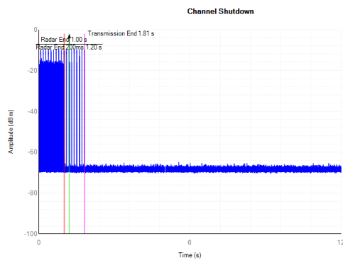
5530MHz Shutdown
