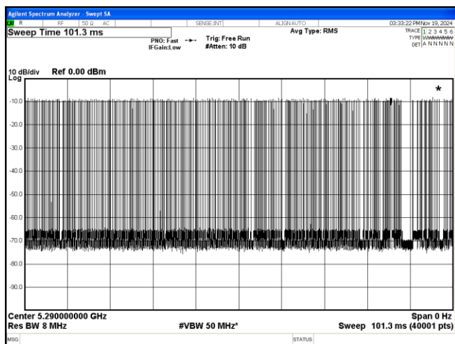
Bandwidth 80MHz
