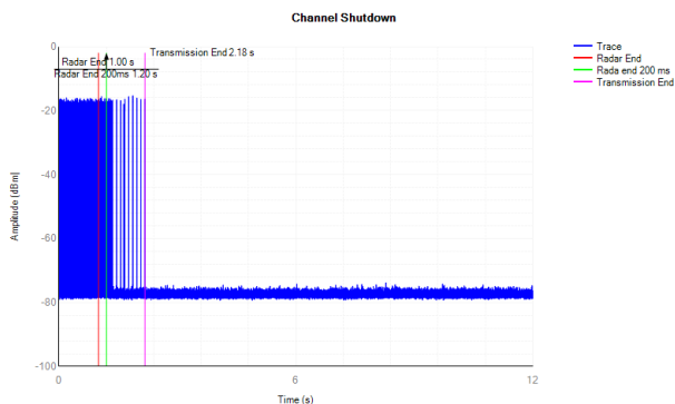
5290MHz Shutdown
