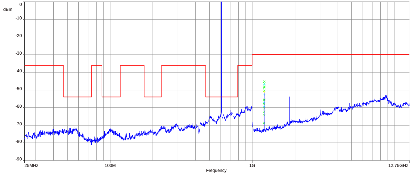
Plot 3: 607.9 MHz, spurious emissions, 25 MHz – 12.75 GHz
