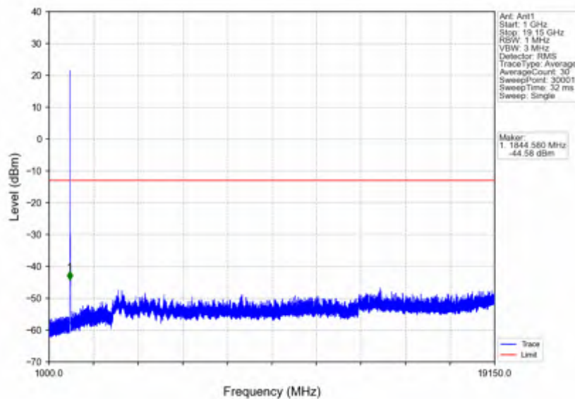
n25_15kHz_SISO_NTV_15MHz_CP-OFDM QPSK_1882.5MHz_Edge_1RB_Left
