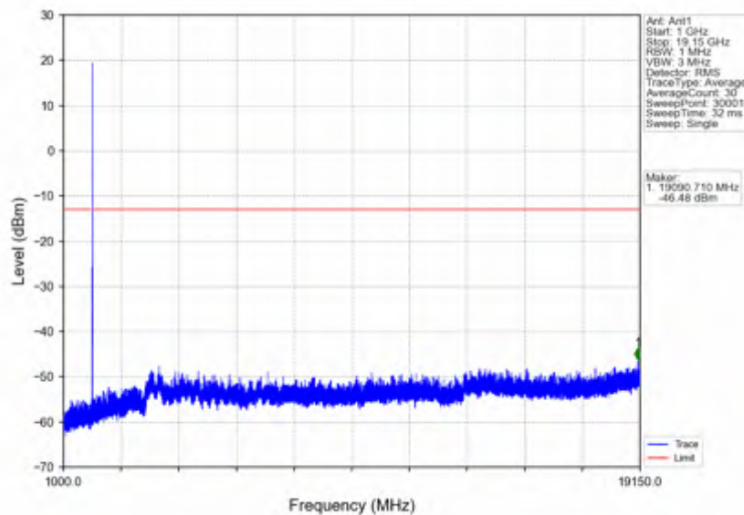
n25_15kHz_SISO_NTNV_10MHz_CP-OFDM QPSK_1910MHz_Outer_Full
