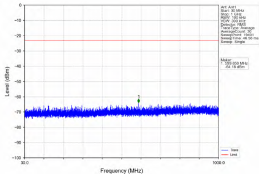
n25_15kHz_SISO_NTNV_15MHz_DFT-s-OFDM QPSK_1907.5MHz_Inner_1RB_Right
