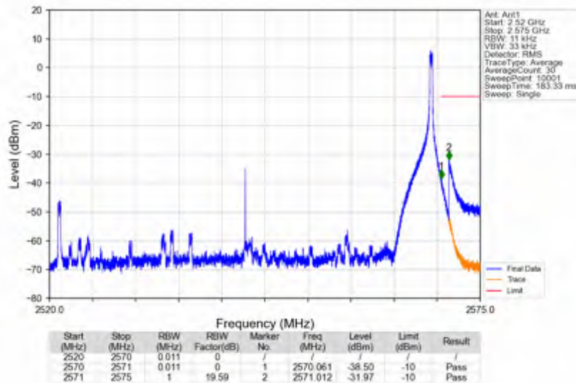
n7_30kHz_SISO_NTNV_50MHz_DFT-s-OFDM_PI/2_BPSK_2545MHz_Edge_1RB_Right
