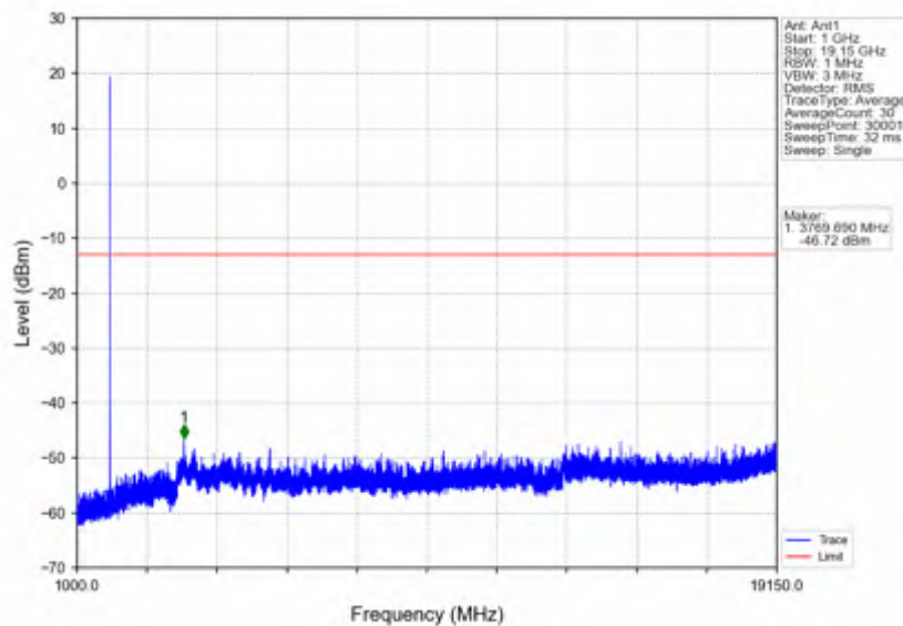
n25_15kHz_SISO_NTNV_5MHz_CP-OFDM QPSK_1852.5MHz_Outer_Full
