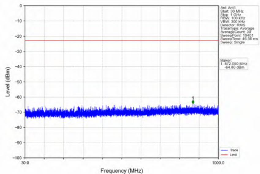
n25_15kHz_SISO_NTNV_10MHz_DFT-s-OFDM QPSK_1855MHz_Outer_Full
