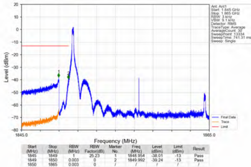
n25_15kHz_SISO_NTNV_15MHz_CP-OFDM_QPSK_1857.5MHz_Edge_1RB_Left
