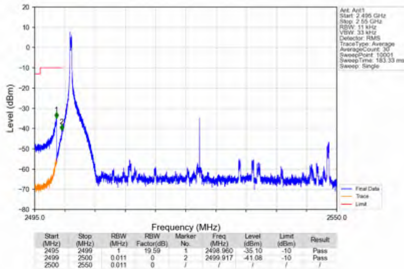
n7_30kHz_SISO_NTNV_50MHz_DFT-s-OFDM QPSK_2525MHz_Inner_1RB_Left
