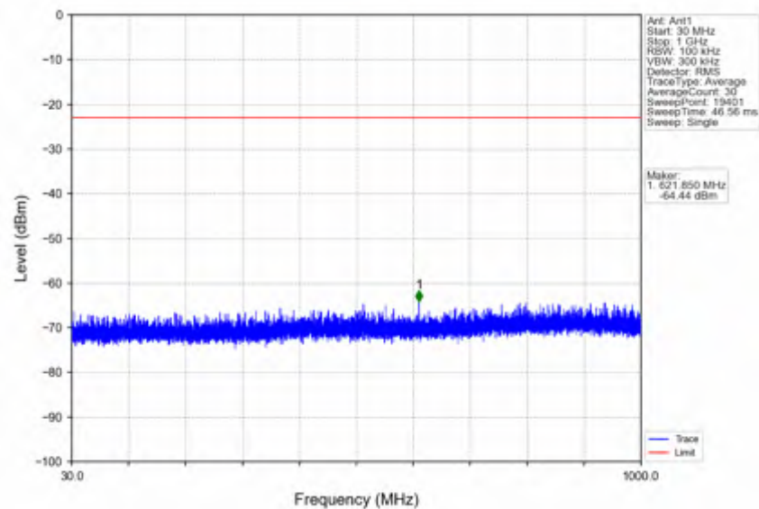
n25_15kHz_SISO_NTNV_15MHz_CP-OFDM QPSK_1857.5MHz_Outer_Full
