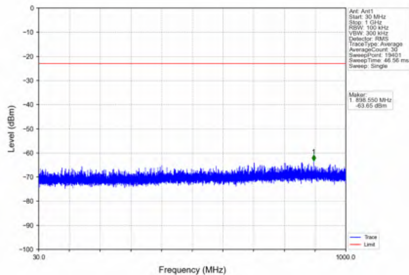
n25_15kHz_SISO_NTNV_5MHz_CP-OFDM QPSK_1852.5MHz_Inner_1RB_Left
