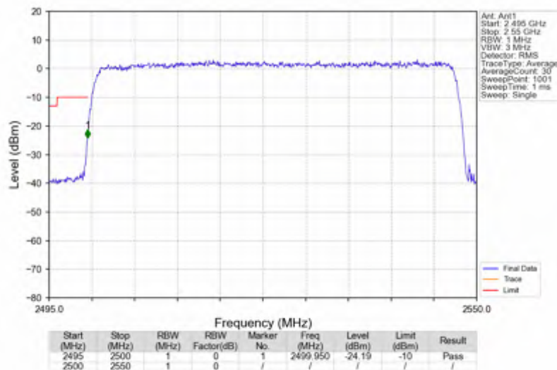
n7_30kHz_SISO_NTNV_50MHz_DFT-s-OFDM QPSK_2525MHz_Outer_Full
