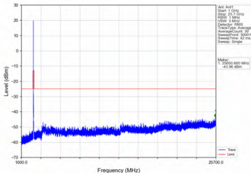
n7_30kHz_SISO_NTNV_40MHz_CP-OFDM QPSK_2550MHz_Edge_1RB_Right
