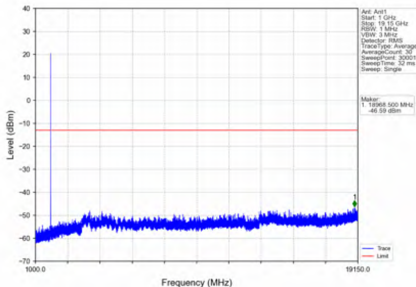
n25_15kHz_SISO_NTNV_5MHz_CP-OFDM QPSK_1882.5MHz_Edge_1RB_Left
