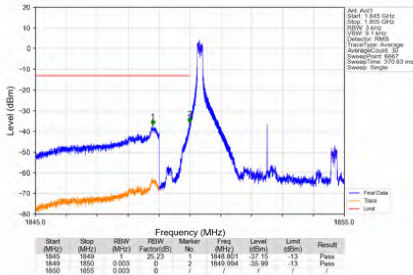
n25_15kHz_SISO_NTNV_5MHz_DFT-s-OFDM QPSK_1852.5MHz_Edge_1RB_Left
