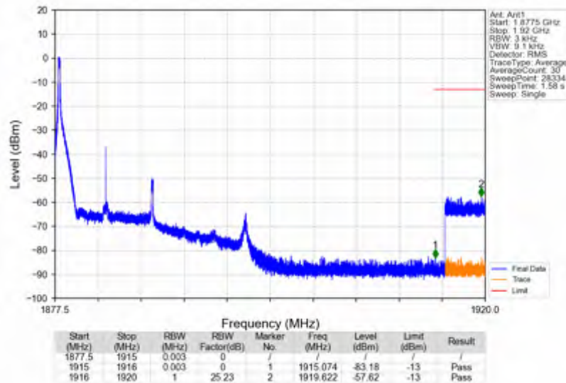
n25_15kHz_SISO_NTNV_10MHz_CP-OFDM QPSK_1882.5MHz_Edge_1RB_Left
