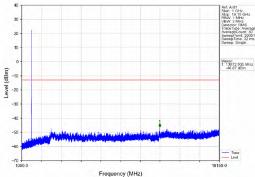
n25_15kHz_SISO_NTNV_5MHz_DFT-s-OFDM QPSK_1852.5MHz_Edge_1RB_Left
