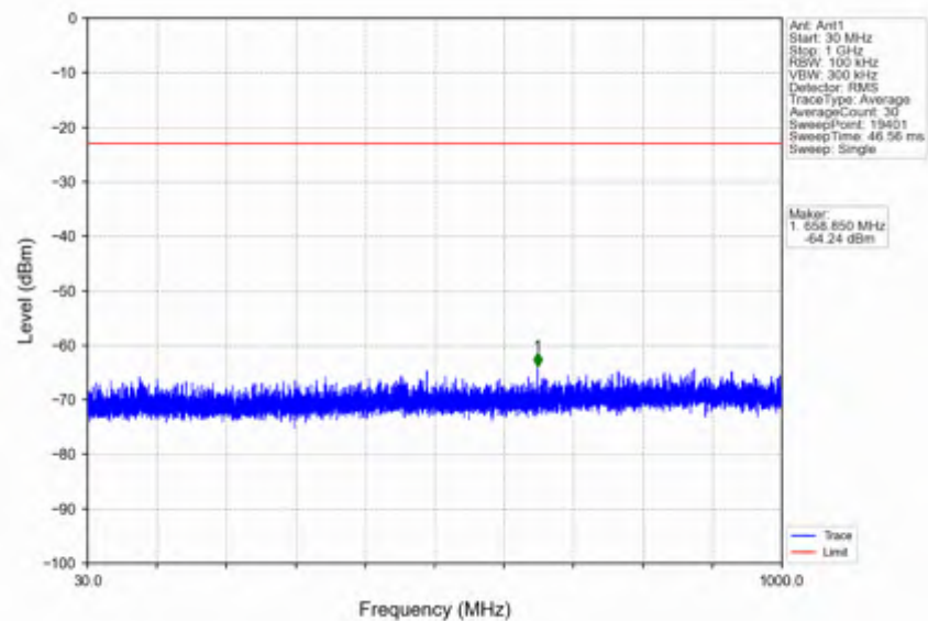
n25_15kHz_SISO_NTNV_10MHz_CP-OFDM QPSK_1855MHz_Edge_1RB_Left
