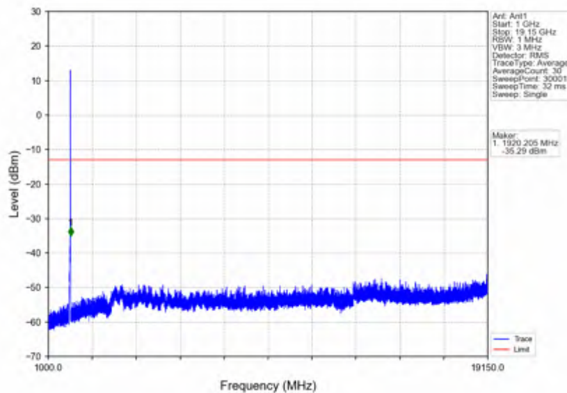
n25_15kHz_SISO_NTNV_15MHz_DFT-s-OFDM QPSK_1907.5MHz_Inner_1RB_Right
