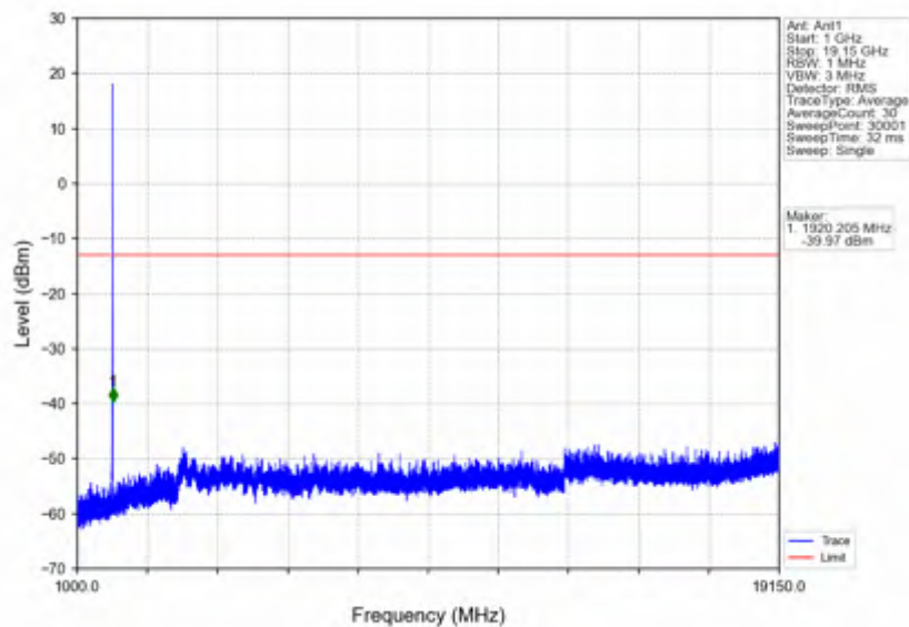
n25_15kHz_SISO_NTNV_5MHz_DFT-s-OFDM QPSK_1912.5MHz_Inner_1RB_Right
