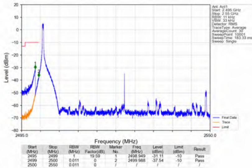
n7_30kHz_SISO_NTNV_50MHz_DFT-s-OFDM_PI/2_BPSK_2525MHz_Edge_1RB_Left
