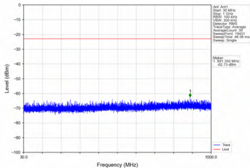
n7_30kHz_SISO_NTNV_50MHz_DFT-s-OFDM QPSK_2525MHz_Edge_1RB_Left
