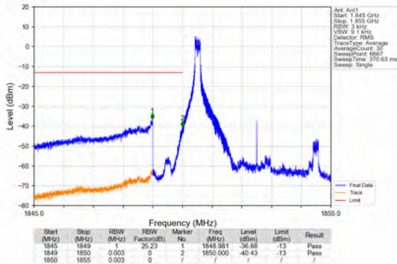
n25_15kHz_SISO_NTNV_5MHz_DFT-s-OFDM QPSK_1852.5MHz_Inner_1RB_Left
