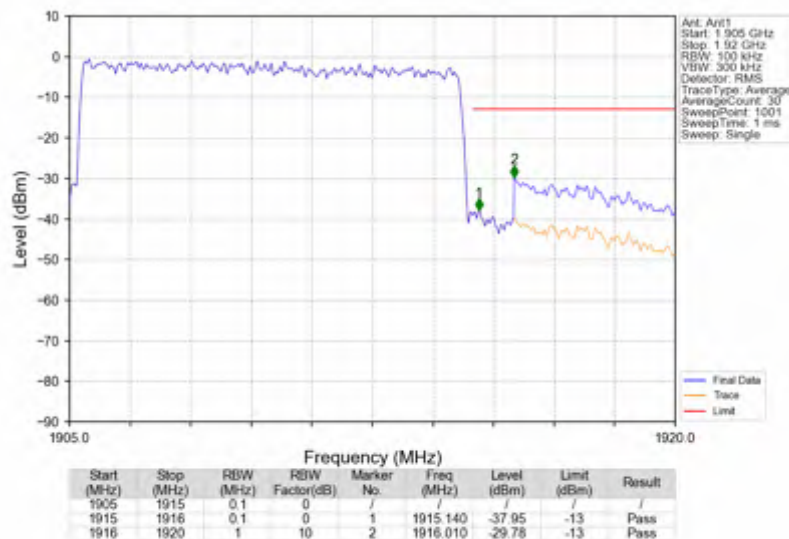
n25_15kHz_SISO_NTNV_10MHz_CP-OFDM QPSK_1910MHz_Outer_Full
