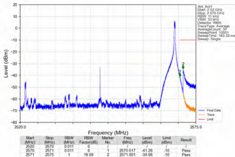
n7_30kHz_SISO_NTNV_50MHz_DFT-s-OFDM QPSK_2545MHz_Inner_1RB_Right
