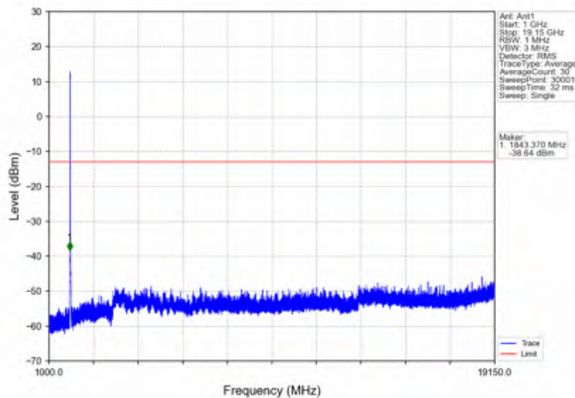
n25_15kHz_SISO_NTNV_15MHz_DFT-s-OFDM_QPSK_1857.5MHz_Inner_1RB_Left
