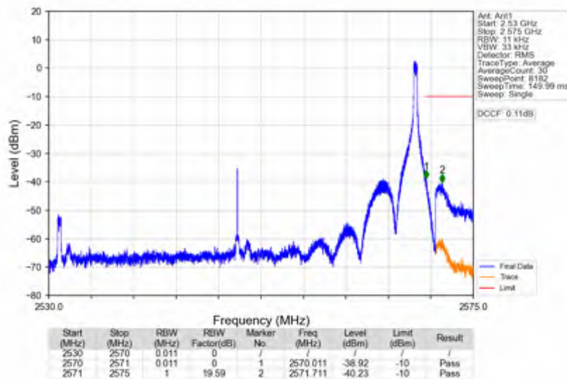
n7_30kHz_SISO_NTNV_40MHz_CP-OFDM QPSK_2550MHz_Edge_1RB_Right
