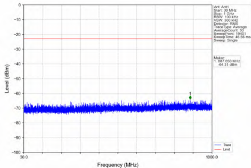
n25_15kHz_SISO_NTNV_5MHz_DFT-s-OFDM_PI/2_BPSK_1912.5MHz_Outer_Full
