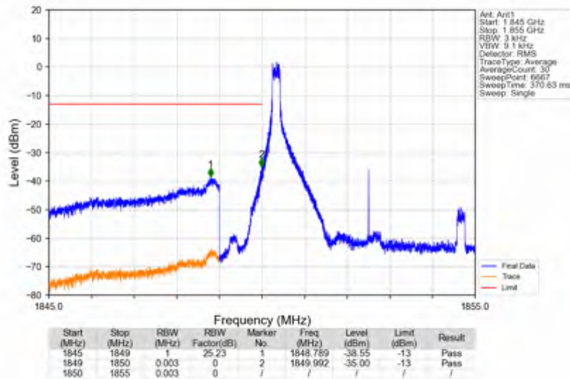
n25_15kHz_SISO_NTNV_5MHz_CP-OFDM QPSK_1852.5MHz_Edge_1RB_Left
