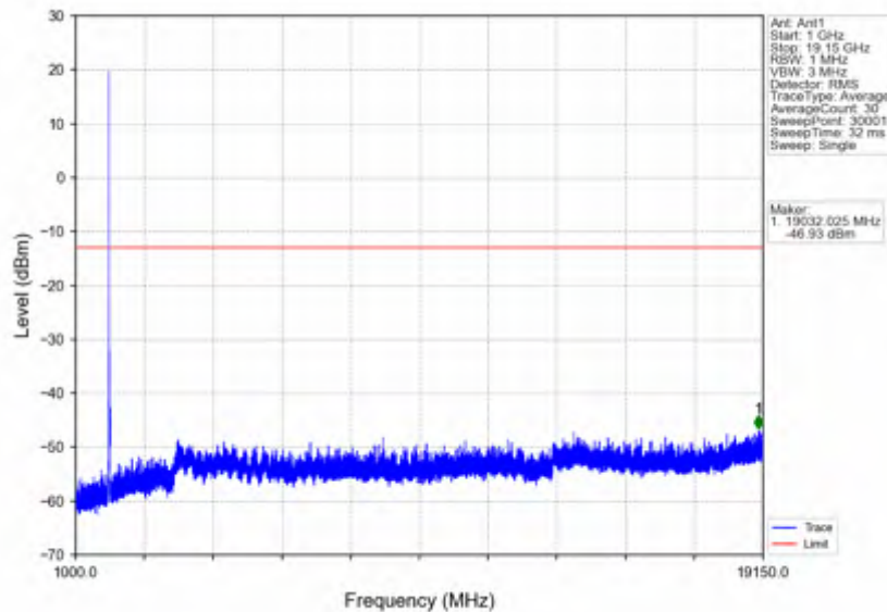
n25_15kHz_SISO_NTNV_15MHz_CP-OFDM_QPSK_1882.5MHz_Edge_1RB_Left
