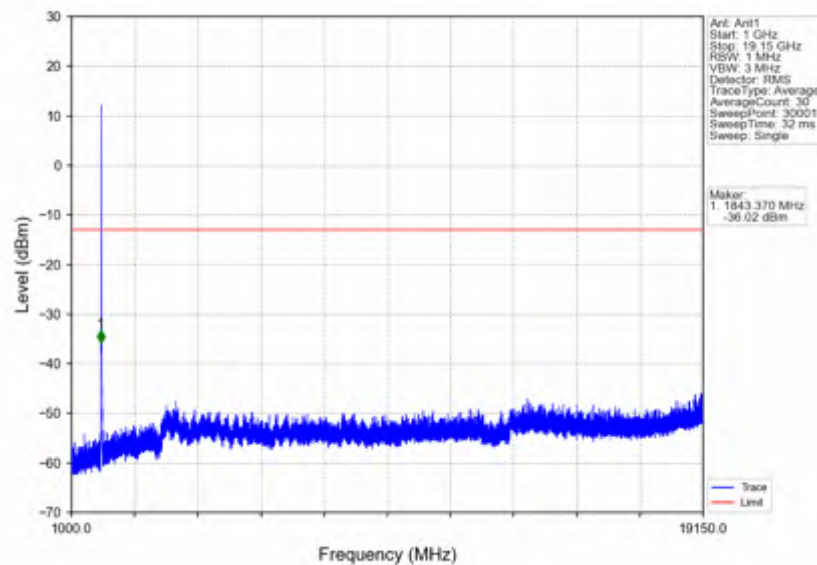
n25_15kHz_SISO_NTNV_10MHz_CP-OFDM_QPSK_1855MHz_Outer_Full
