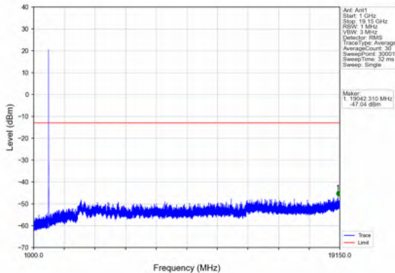
n25_15kHz_SISO_NTNV_10MHz_CP-OFDM QPSK_1882.5MHz_Edge_1RB_Left
