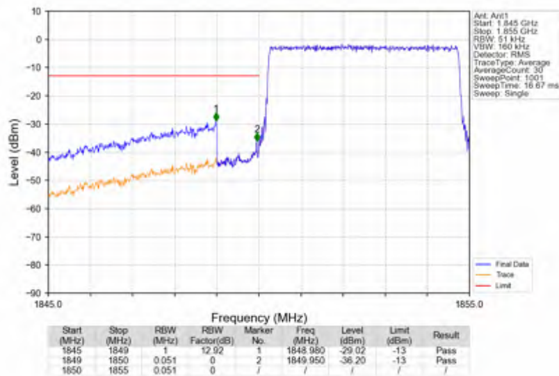
n25_15kHz_SISO_NTNV_5MHz_CP-OFDM QPSK_1852.5MHz_Outer_Full
