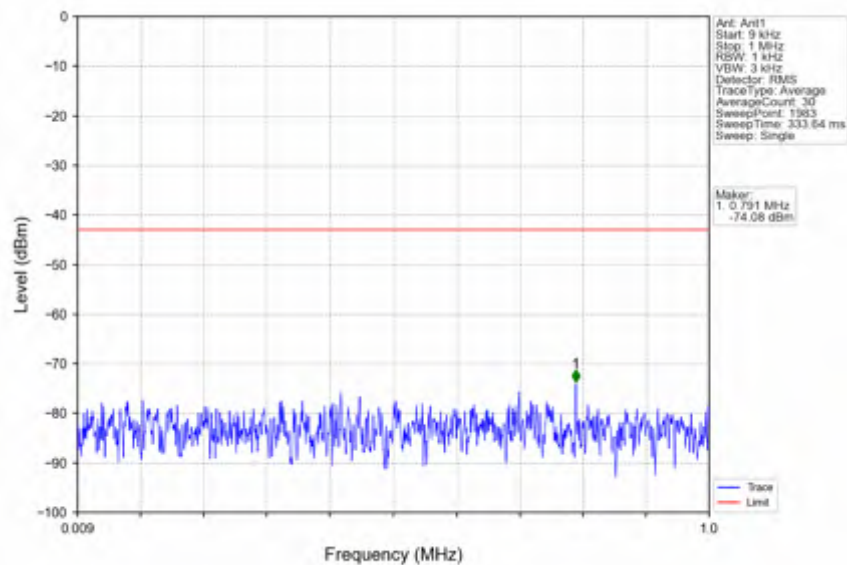
n25_15kHz_SISO_NTNV_10MHz_CP-OFDM QPSK_1855MHz_Outer_Full
