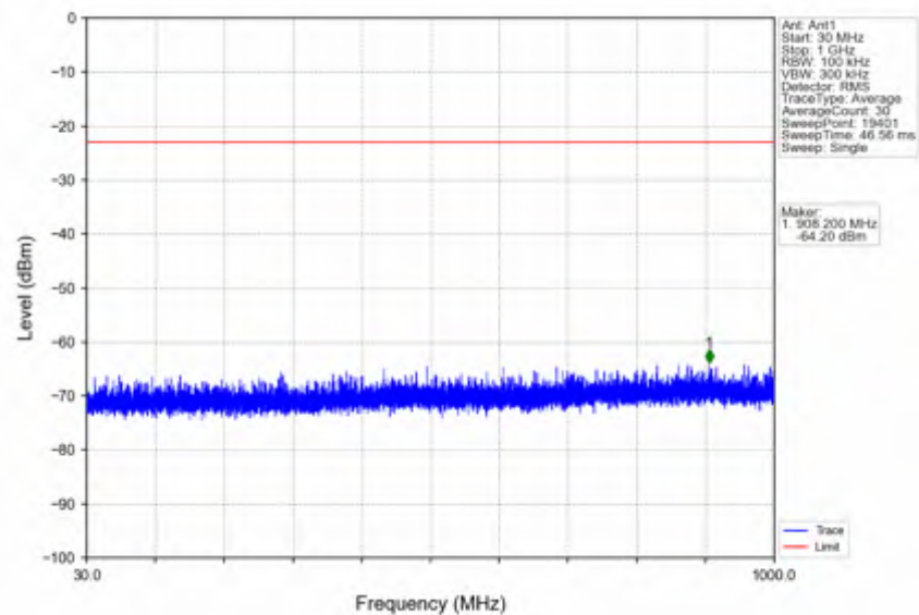
n25_15kHz_SISO_NTNV_5MHz_CP-OFDM QPSK_1912.5MHz_Edge_1RB_Right
