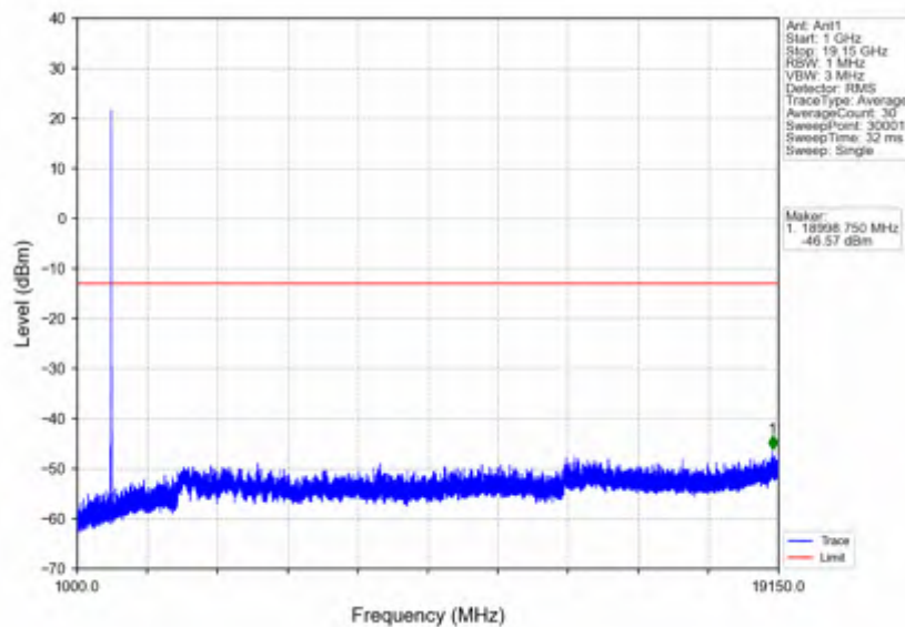
n25_15kHz_SISO_NTNV_10MHz_DFT-s-OFDM QPSK_1910MHz_Edge_1RB_Right
