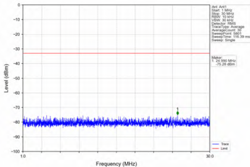
n25_15kHz_SISO_NTNV_5MHz_CP-OFDM QPSK_1912.5MHz_Outer_Full
