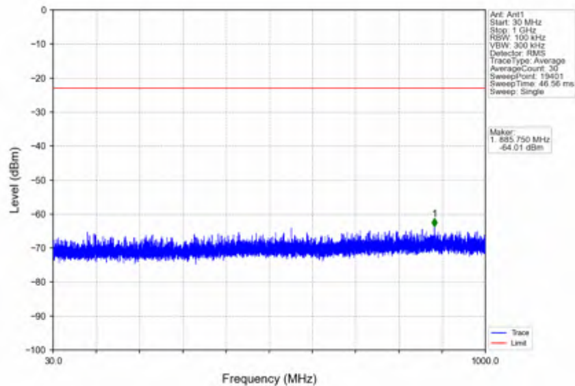
n25_15kHz_SISO_NTNV_10MHz_CP-OFDM_QPSK_1910MHz_Outer_Full
