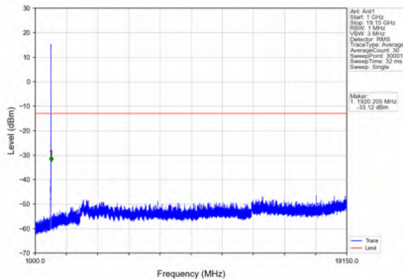
n25_15kHz_SISO_NTNV_10MHz_DFT-s-OFDM QPSK_1910MHz_Inner_1RB_Right
