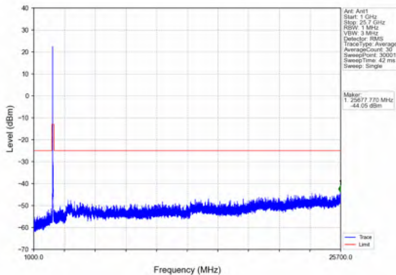
n7_30kHz_SISO_NTNV_50MHz_DFT-s-OFDM_PI/2_BPSK_2545MHz_Edge_1RB_Right
