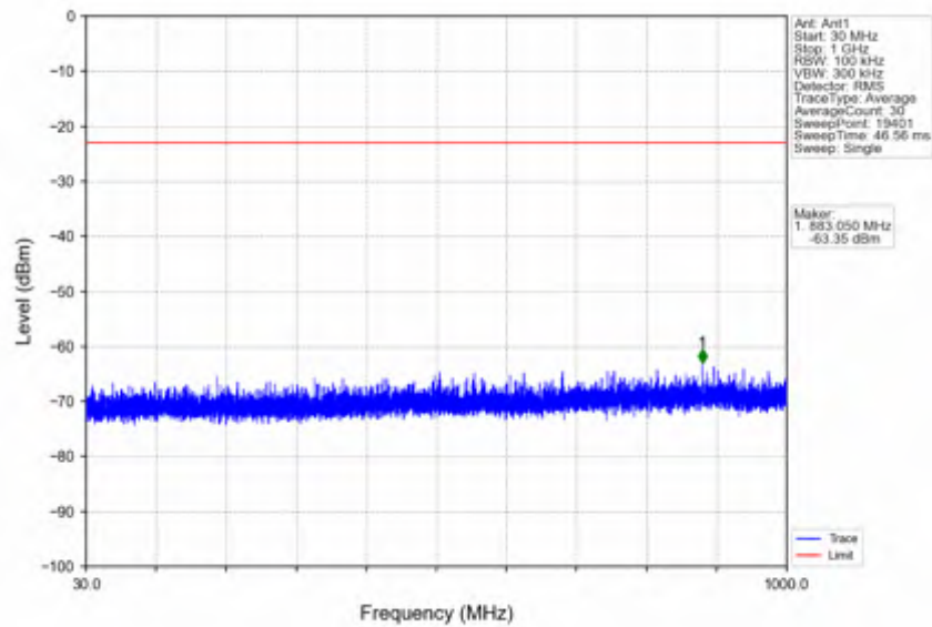
n25_15kHz_SISO_NTNV_5MHz_CP-OFDM QPSK_1852.5MHz_Outer_Full
