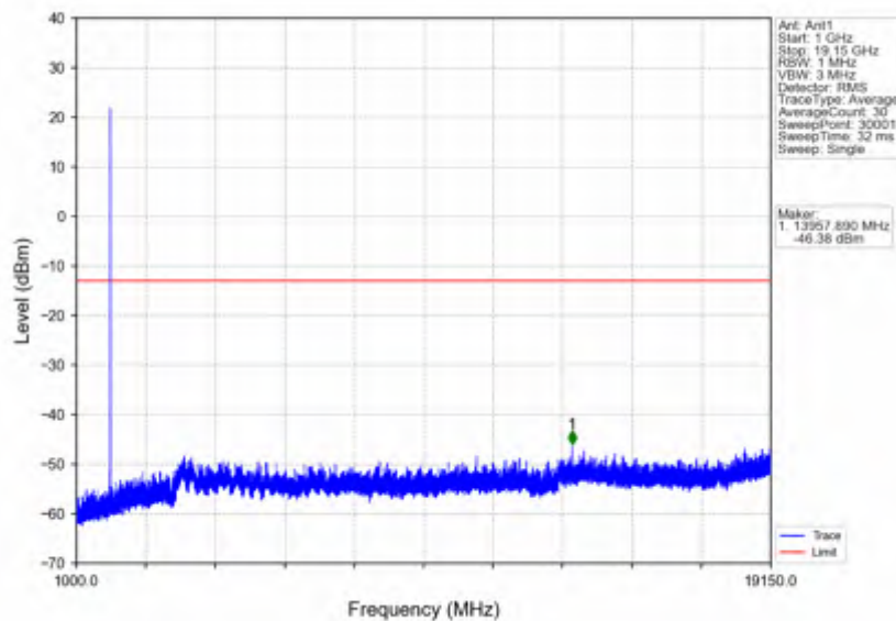
n25_15kHz_SISO_NTNV_5MHz_DFT-s-OFDM QPSK_1912.5MHz_Edge_1RB_Right
