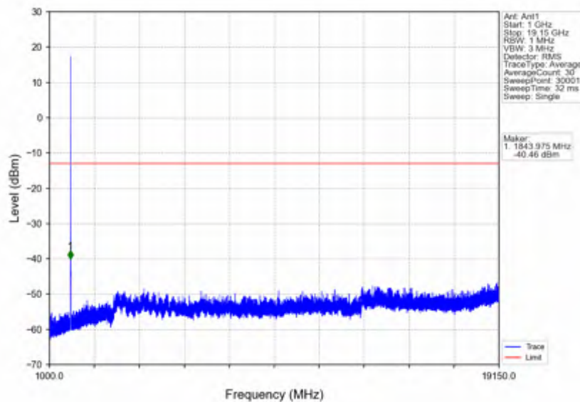
n25_15kHz_SISO_NTNV_5MHz_DFT-s-OFDM QPSK_1852.5MHz_Inner_1RB_Left
