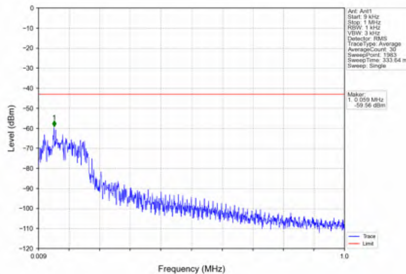
n25_15kHz_SISO_NTNV_5MHz_DFT-s-OFDM QPSK_1882.5MHz_Edge_1RB_Left
