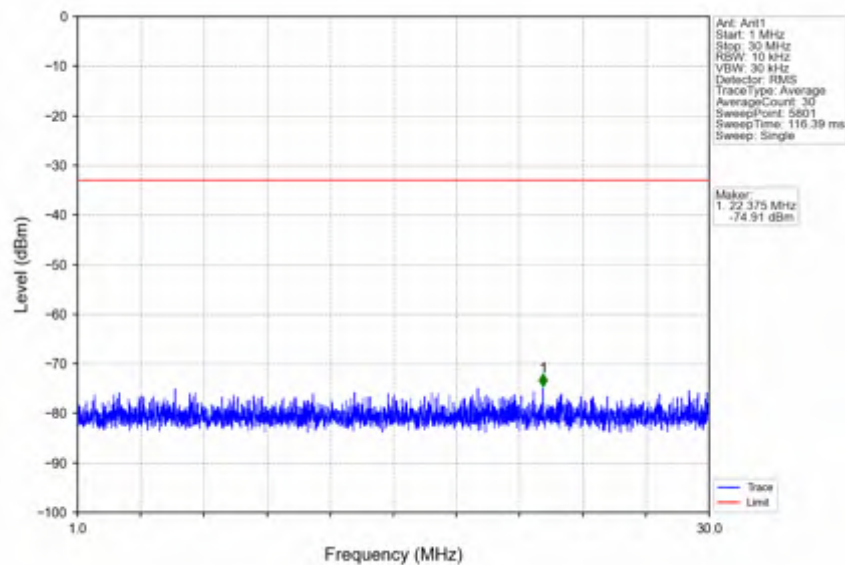
n25_15kHz_SISO_NTNV_10MHz_CP-OFDM QPSK_1910MHz_Outer_Full
