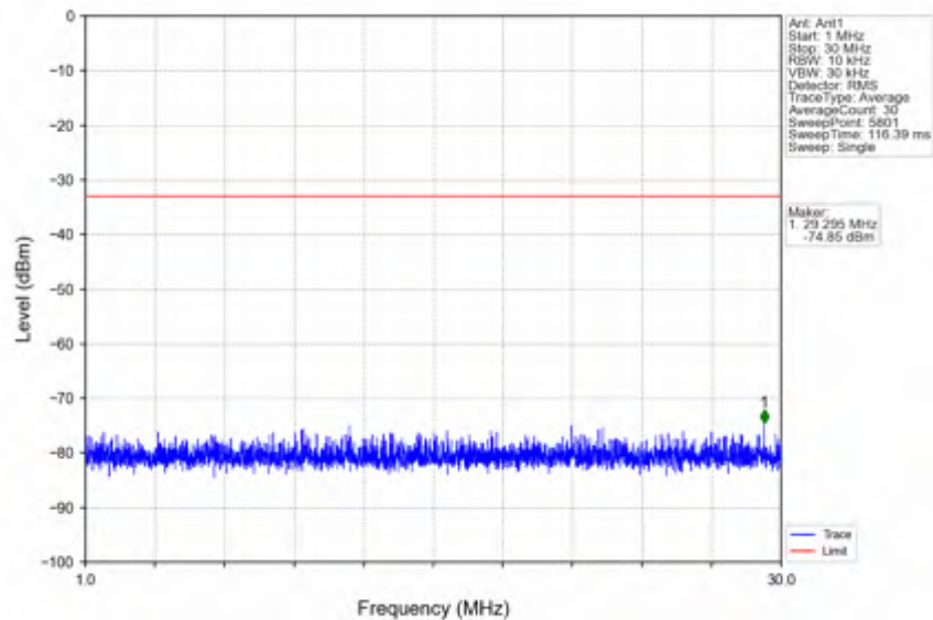
n25_15kHz_SISO_NTNV_15MHz_CP-OFDM_QPSK_1882.5MHz_Edge_1RB_Left
