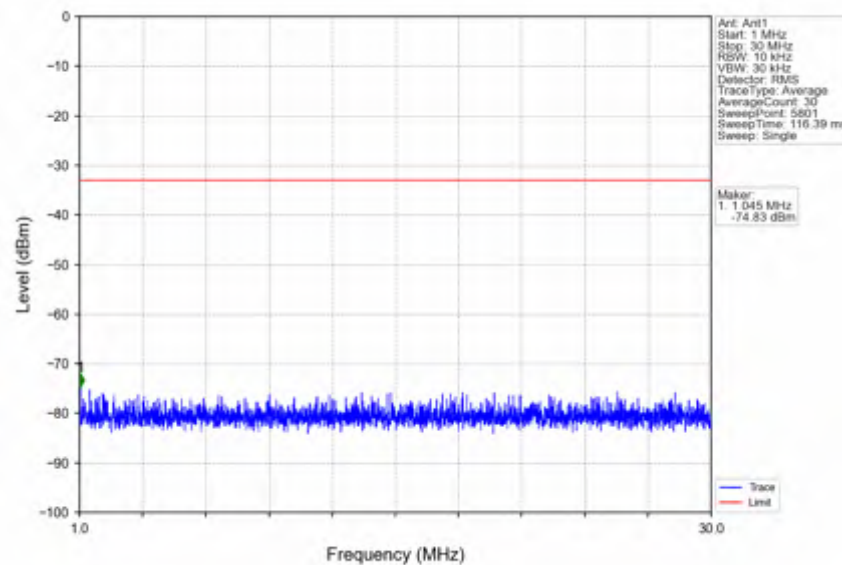
n25_15kHz_SISO_NTNV_10MHz_CP-OFDM QPSK_1910MHz_Edge_1RB_Right
