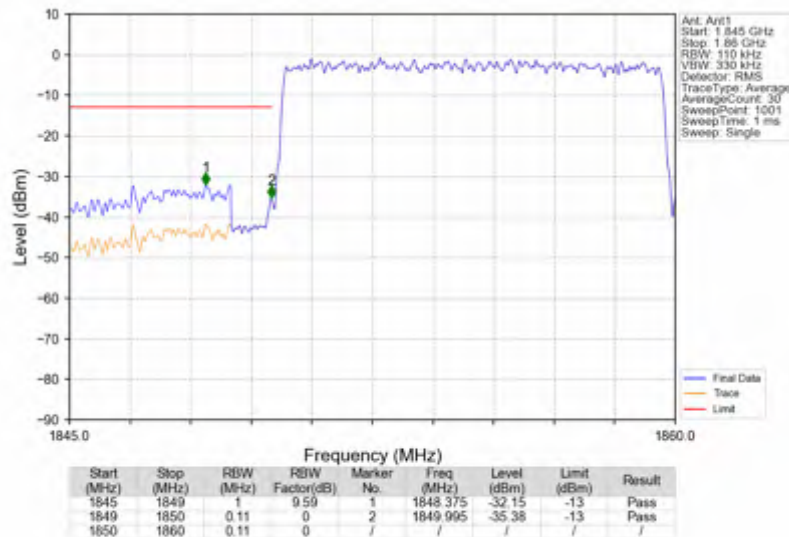
n25_15kHz_SISO_NTNV_10MHz_CP-OFDM QPSK_1855MHz_Outer_Full
