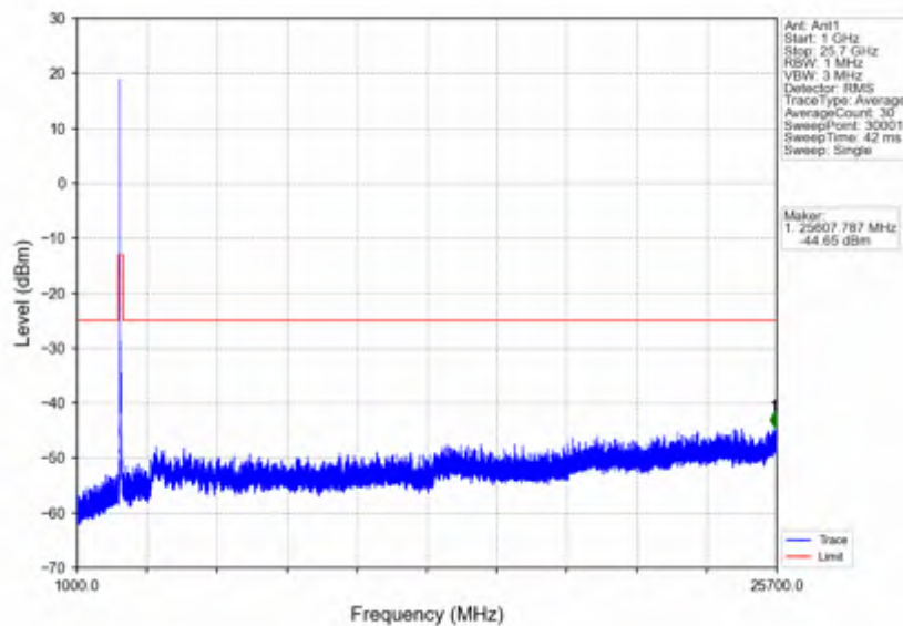
n7_30kHz_SISO_NTNV_50MHz_CP-OFDM QPSK_2525MHz_Outer_Full
