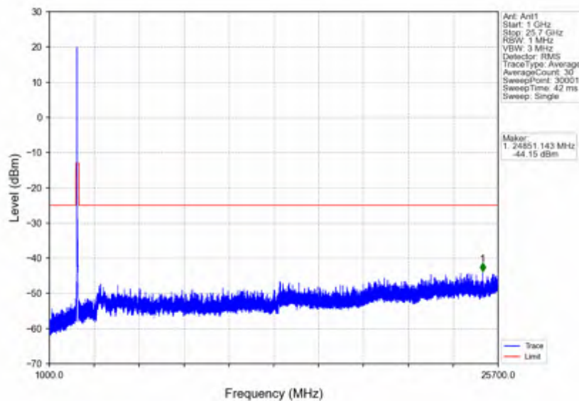
n7_30kHz_SISO_NTNV_50MHz_CP-OFDM QPSK_2545MHz_Edge_1RB_Right
