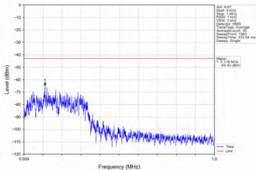
n7_30kHz_SISO_NTNV_50MHz_DFT-s-OFDM QPSK_2545MHz_Edge_1RB_Right
