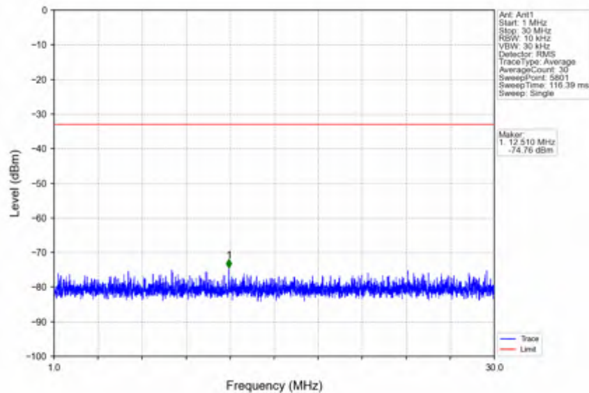
n25_15kHz_SISO_NTV_15MHz_CP-OFDM QPSK_1857.5MHz_Inner_1RB_Left
