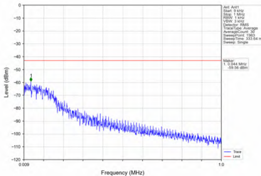
n25_15kHz_SISO_NTNV_5MHz_CP-OFDM_QPSK_1852.5MHz_Inner_1RB_Left
