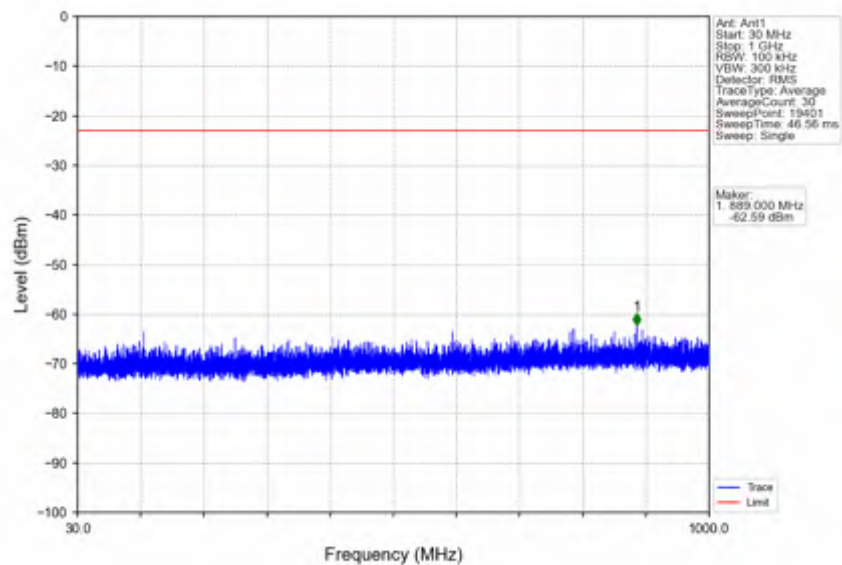
n7_30kHz_SISO_NTNV_50MHz_CP-OFDM QPSK_2525MHz_Edge_1RB_Left
