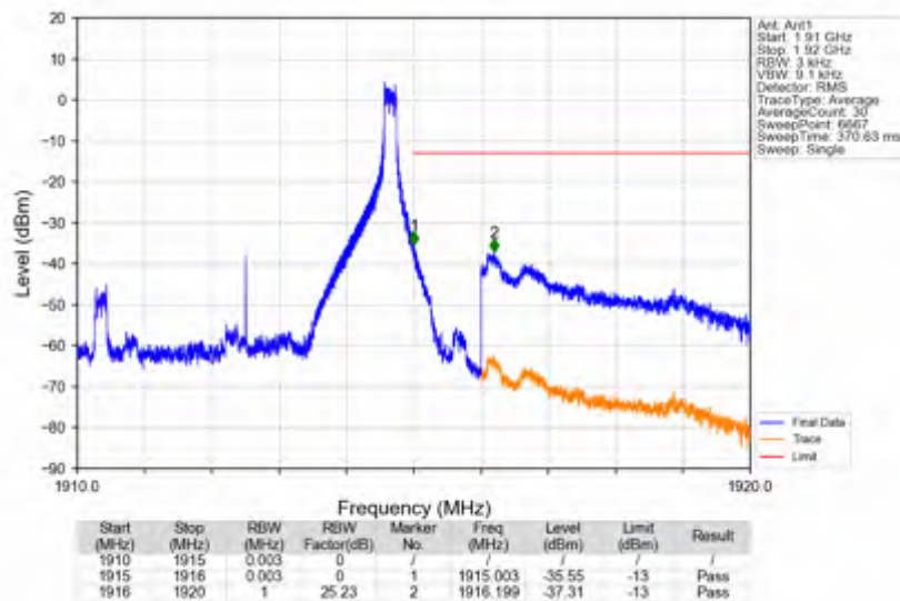
n25_15kHz_SISO_NTNV_5MHz_DFT-s-OFDM QPSK_1912.5MHz_Edge_1RB_Right
