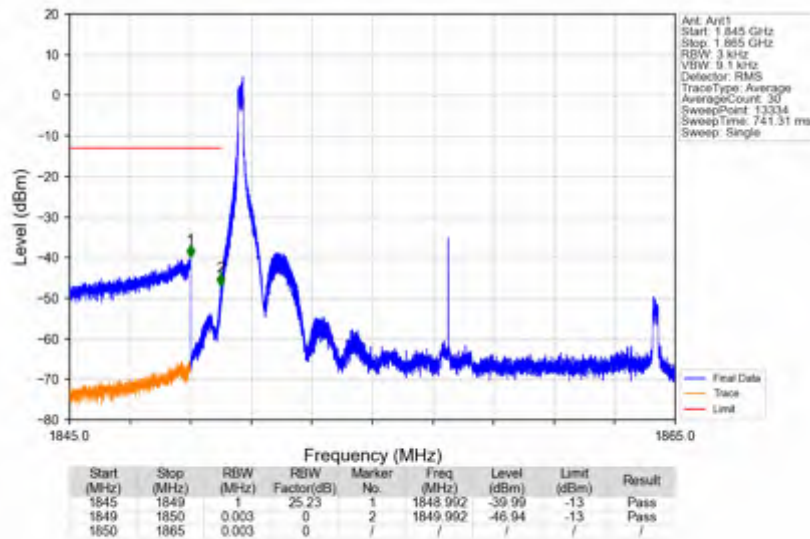
n25_15kHz_SISO_NTV_15MHz_CP-OFDM_QPSK_1857.5MHz_Inner_1RB_Left
