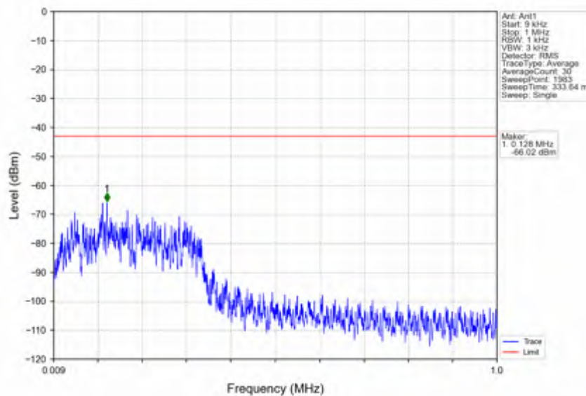
n7_30kHz_SISO_NTNV_50MHz_DFT-s-OFDM QPSK_2525MHz_Edge_1RB_Left
