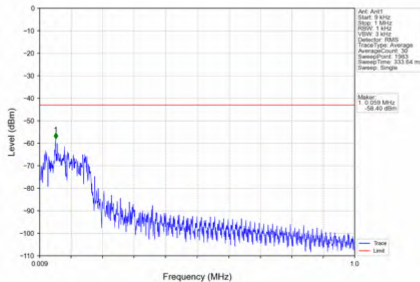
n25_15kHz_SISO_NTNV_10MHz_DFT-s-OFDM QPSK_1910MHz_Edge_1RB_Right
