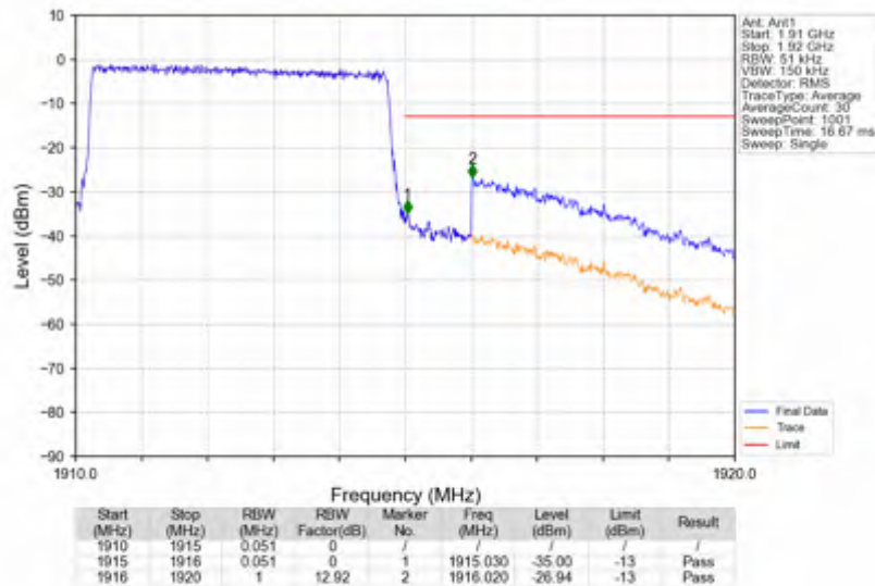
n25_15kHz_SISO_NTNV_5MHz_CP-OFDM QPSK_1912.5MHz_Outer_Full
