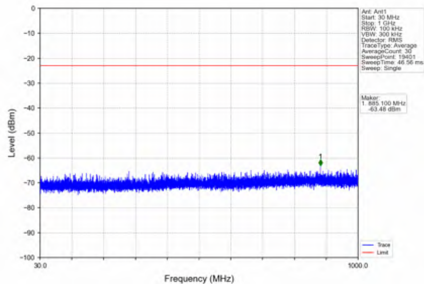
n25_15kHz_SISO_NTNV_10MHz_DFT-s-OFDM_QPSK_1910MHz_Inner_1RB_Right
