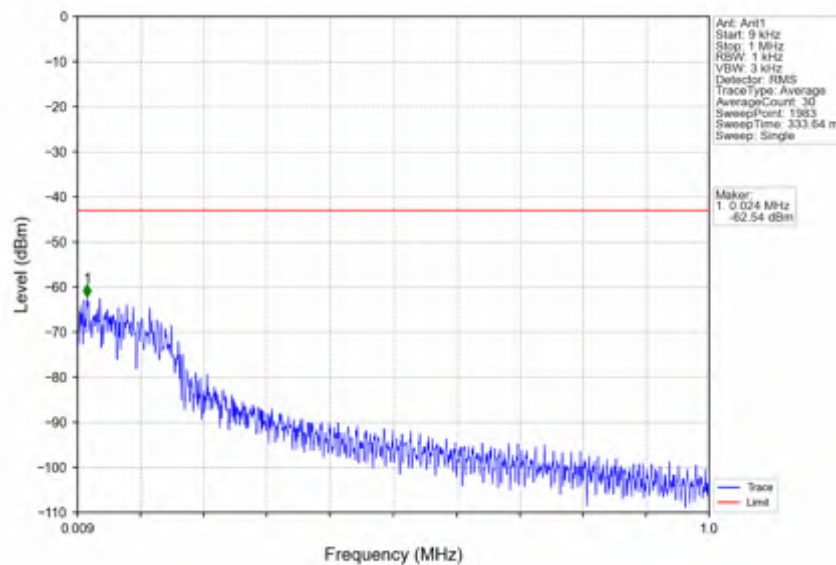
n25_15kHz_SISO_NTNV_10MHz_CP-OFDM_QPSK_1910MHz_Edge_1RB_Right
