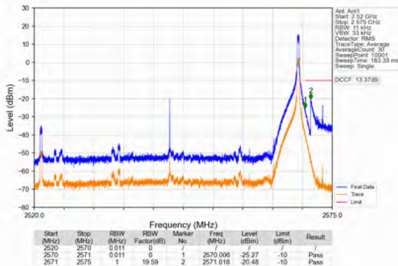
n7_30kHz_SISO_NTNV_50MHz_CP-OFDM QPSK_2545MHz_Edge_1RB_Right
