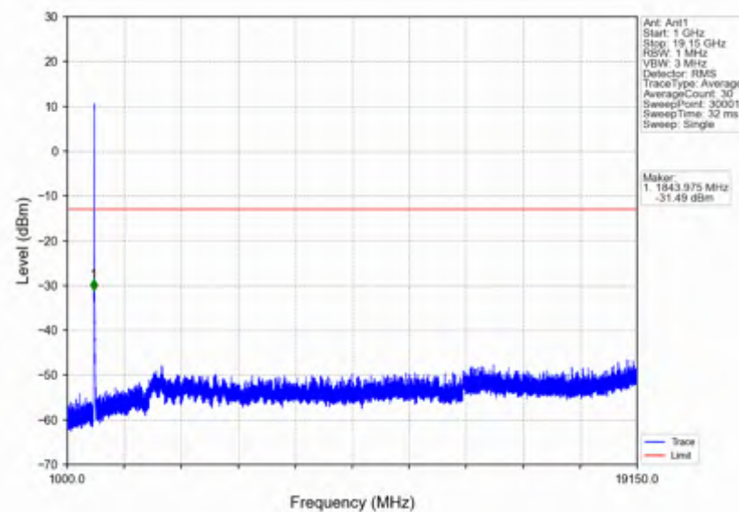
n25_15kHz_SISO_NTNV_15MHz_CP-OFDM QPSK_1857.5MHz_Outer_Full
