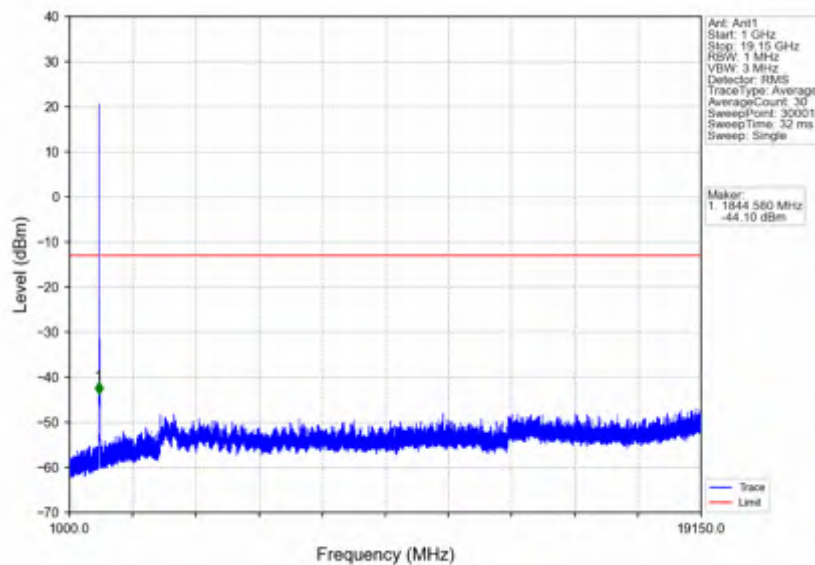
n25_15kHz_SISO_NTNV_15MHz_CP-OFDM QPSK_1857.5MHz_Outer_Full
