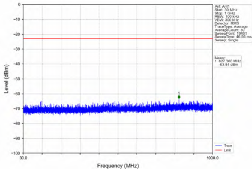
n25_15kHz_SISO_NTNV_5MHz_CP-OFDM QPSK_1912.5MHz_Outer_Full
