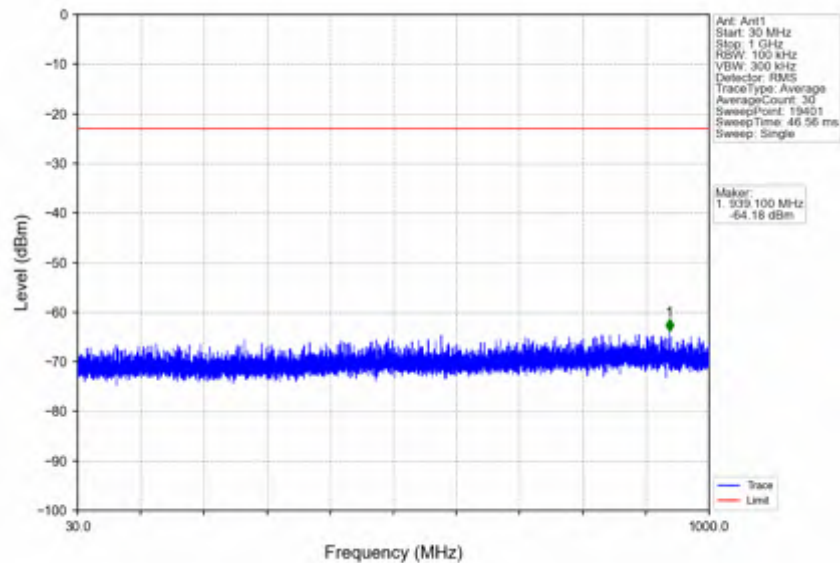
n25_15kHz_SISO_NTNV_10MHz_CP-OFDM QPSK_1882.5MHz_Edge_1RB_Left
