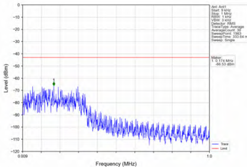
n7_30kHz_SISO_NTNV_50MHz_DFT-s-OFDM QPSK_2535MHz_Edge_1RB_Left
