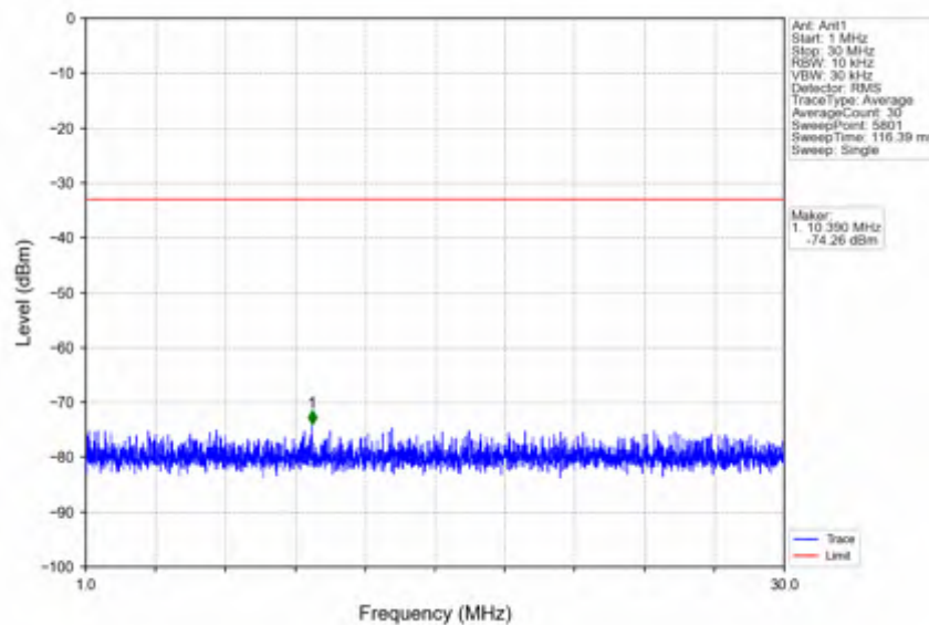
n7_30kHz_SISO_NTNV_50MHz_DFT-s-OFDM QPSK_2535MHz_Edge_1RB_Left
