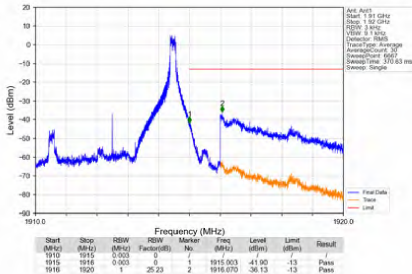
n25_15kHz_SISO_NTNV_5MHz_DFT-s-OFDM QPSK_1912.5MHz_Inner_1RB_Right
