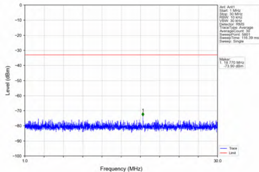
n25_15kHz_SISO_NTNV_10MHz_DFT-s-OFDM QPSK_1855MHz_Outer_Full
