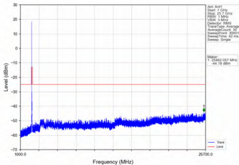
n7_30kHz_SISO_NTNV_40MHz_CP-OFDM QPSK_2520MHz_Outer_Full
