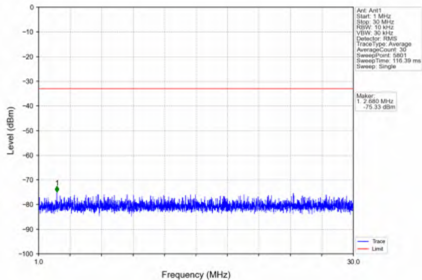
n25_15kHz_SISO_NTNV_10MHz_DFT-s-OFDM QPSK_1855MHz_Edge_1RB_Left
