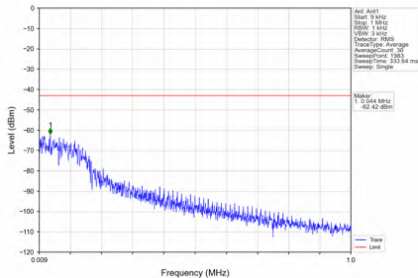
n25_15kHz_SISO_NTNV_5MHz_CP-OFDM QPSK_1882.5MHz_Edge_1RB_Left
