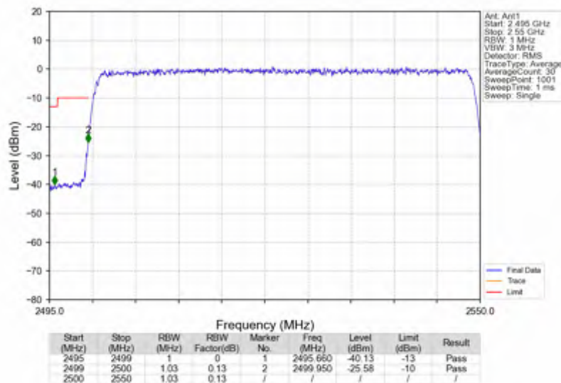
n7_30kHz_SISO_NTNV_50MHz_CP-OFDM QPSK_2525MHz_Outer_Full
