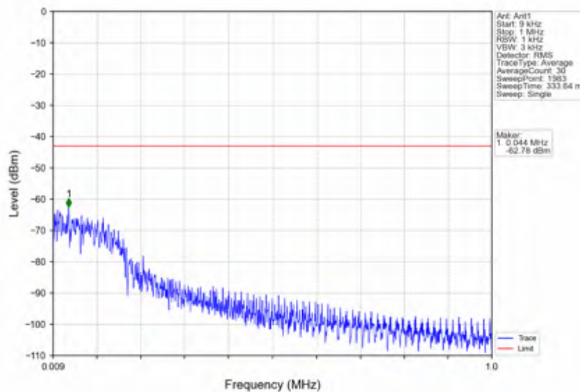
n25_15kHz_SISO_NTNV_15MHz_CP-OFDM_QPSK_1857.5MHz_Edge_1RB_Left
