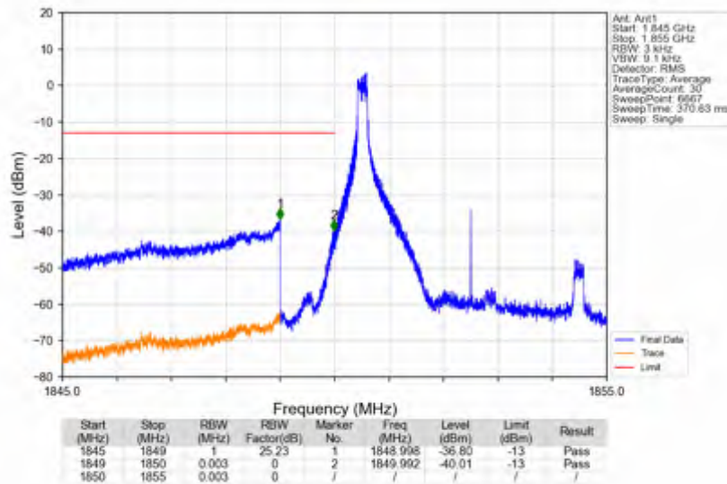
n25_15kHz_SISO_NTNV_5MHz_CP-OFDM_QPSK_1852.5MHz_Inner_1RB_Left
