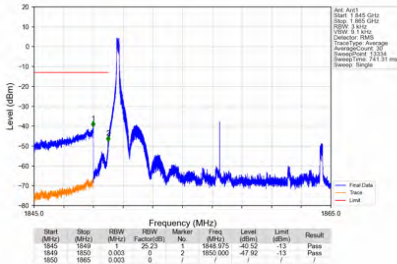
n25_15kHz_SISO_NTNV_15MHz_DFT-s-OFDM_QPSK_1857.5MHz_Inner_1RB_Left
