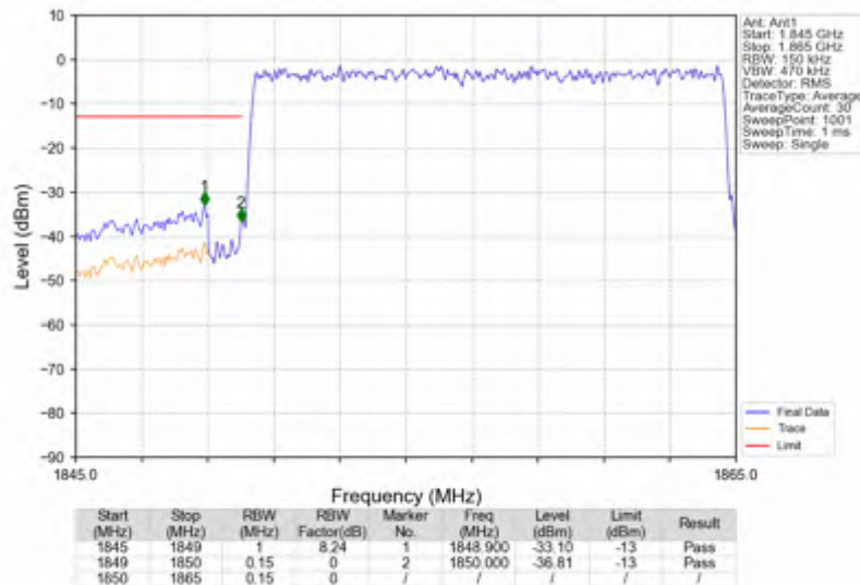
n25_15kHz_SISO_NTNV_15MHz_CP-OFDM QPSK_1857.5MHz_Outer_Full
