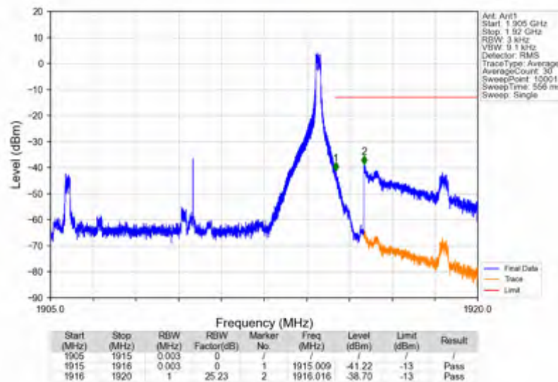
n25_15kHz_SISO_NTNV_10MHz_DFT-s-OFDM QPSK_1910MHz_Inner_1RB_Right
