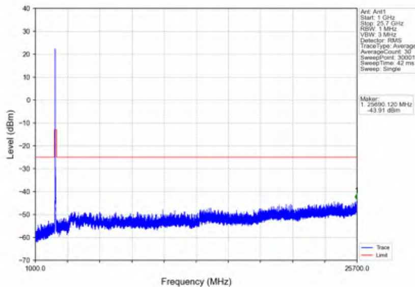
n7_30kHz_SISO_NTNV_50MHz_DFT-s-OFDM_QPSK_2545MHz_Edge_1RB_Right
