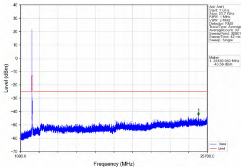
n7_30kHz_SISO_NTNV_50MHz_DFT-s-OFDM QPSK_2525MHz_Outer_Full
