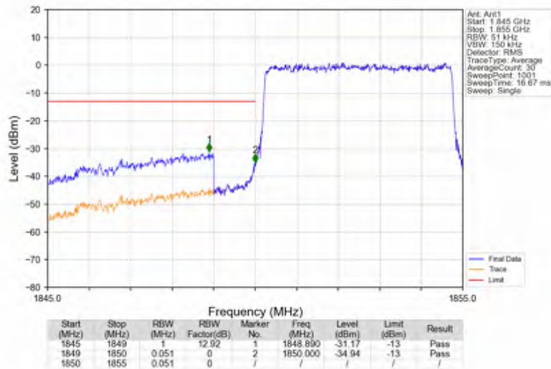
n25_15kHz_SISO_NTNV_5MHz_DFT-s-OFDM QPSK_1852.5MHz_Outer_Full
