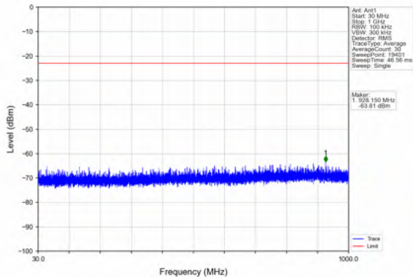
n25_15kHz_SISO_NTNV_15MHz_DFT-s-OFDM_PI/2_BPSK_1882.5MHz_Edge_1RB_Left
