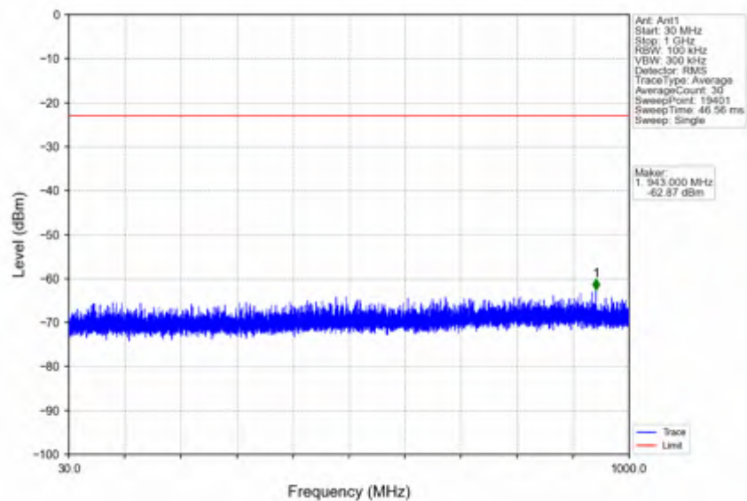
n7_30kHz_SISO_NTNV_50MHz_CP-OFDM QPSK_2535MHz_Edge_1RB_Left
