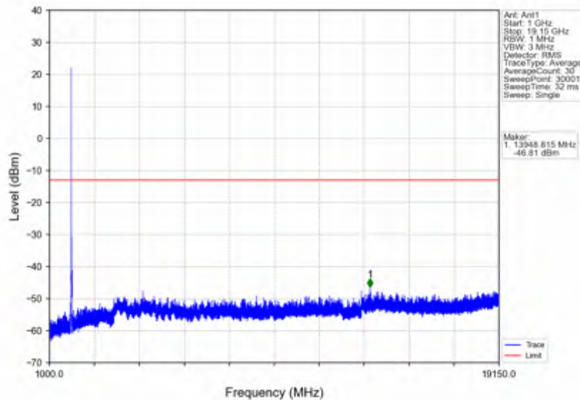
n25_15kHz_SISO_NTNV_15MHz_DFT-s-OFDM_PI/2_BPSK_1882.5MHz_Edge_1RB_Left
