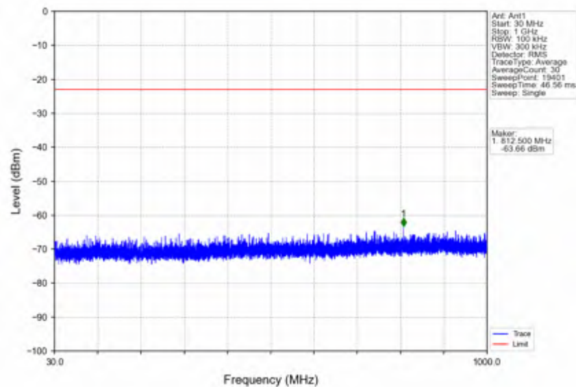
n25_15kHz_SISO_NTNV_15MHz_DFT-s-OFDM_QPSK_1857.5MHz_Outer_Full
