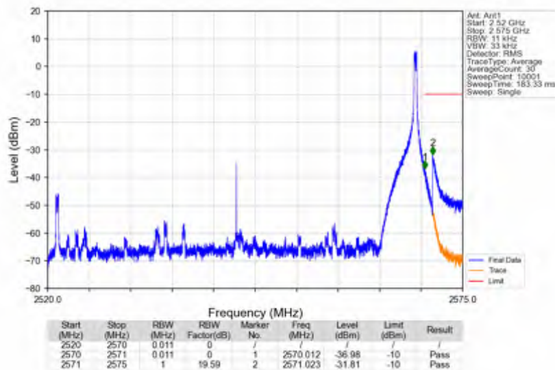
n7_30kHz_SISO_NTNV_50MHz_DFT-s-OFDM_QPSK_2545MHz_Edge_1RB_Right
