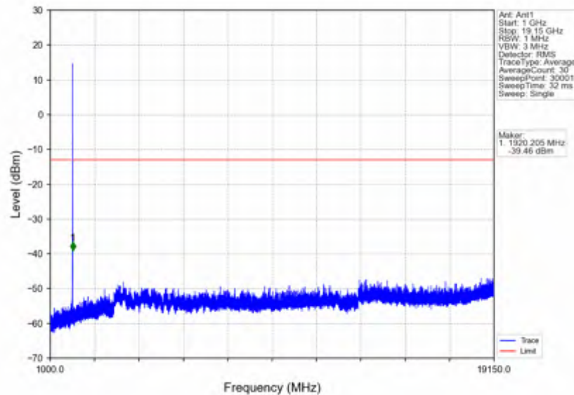
n25_15kHz_SISO_NTNV_5MHz_CP-OFDM QPSK_1912.5MHz_Outer_Full
