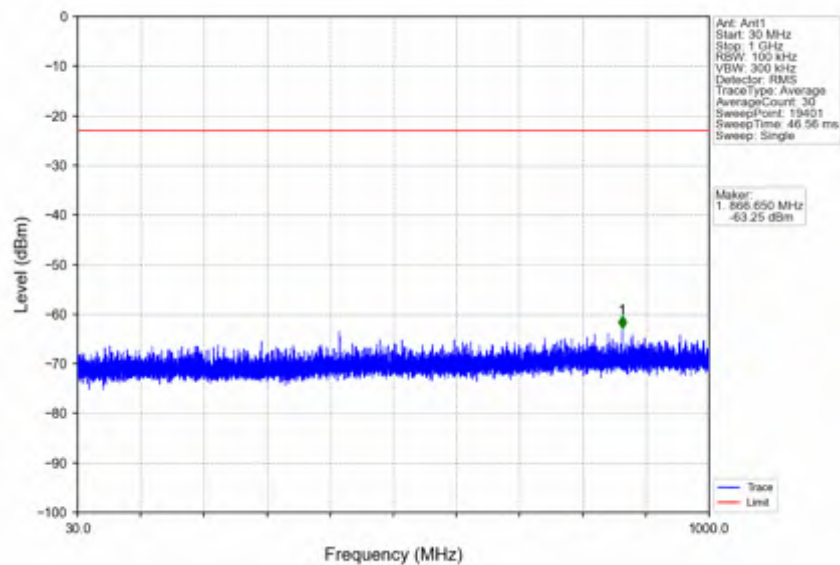
n25_15kHz_SISO_NTNV_15MHz_CP-OFDM QPSK_1857.5MHz_Edge_1RB_Left
