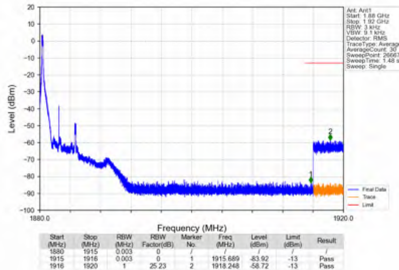
n25_15kHz_SISO_NTNV_5MHz_DFT-s-OFDM QPSK_1882.5MHz_Edge_1RB_Left
