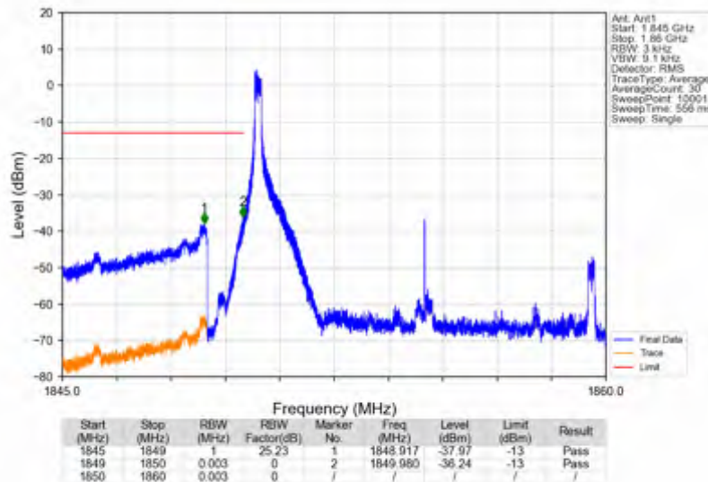
n25_15kHz_SISO_NTNV_10MHz_DFT-s-OFDM QPSK_1855MHz_Edge_1RB_Left
