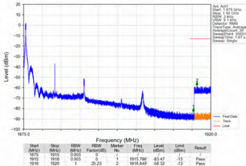
n25_15kHz_SISO_NTV_15MHz_CP-OFDM QPSK_1882.5MHz_Edge_1RB_Left
