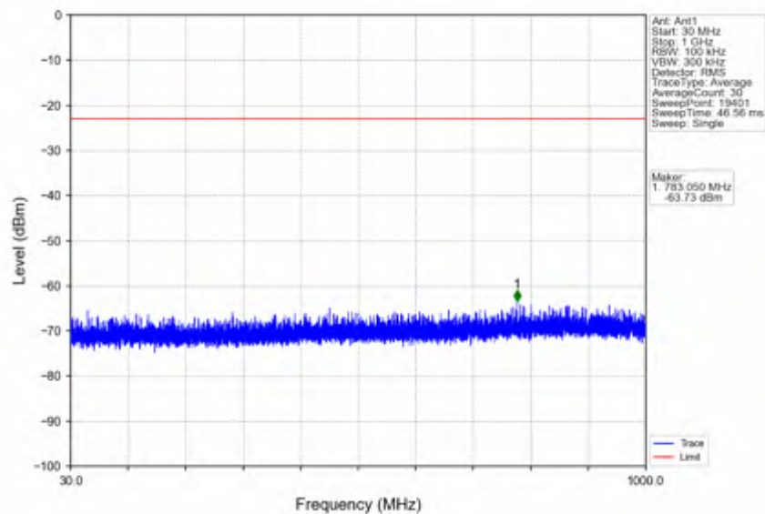
n25_15kHz_SISO_NTNV_10MHz_CP-OFDM QPSK_1910MHz_Inner_1RB_Right
