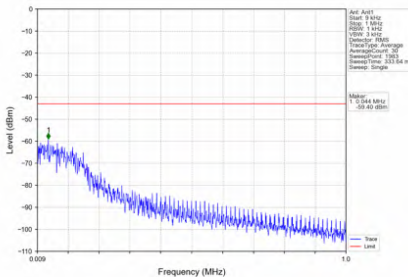
n25_15kHz_SISO_NTV_15MHz_CP-OFDM_QPSK_1857.5MHz_Inner_1RB_Left
