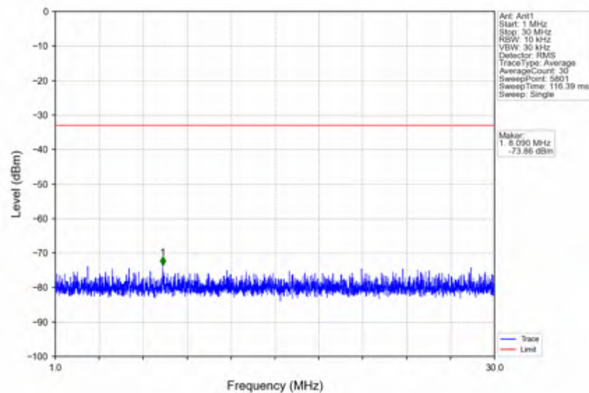
n7_30kHz_SISO_NTNV_50MHz_DFT-s-OFDM QPSK_2525MHz_Edge_1RB_Left
