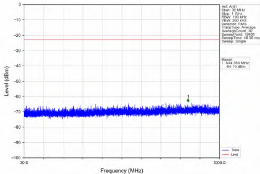
n25_15kHz_SISO_NTNV_10MHz_DFT-s-OFDM_PI/2_BPSK_1855MHz_Outer_Full
