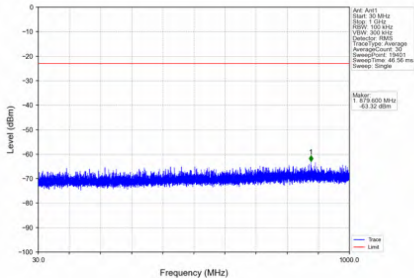
n25_15kHz_SISO_NTNV_15MHz_CP-OFDM_QPSK_1882.5MHz_Edge_1RB_Left
