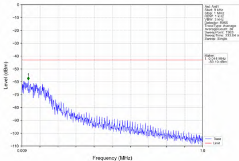
n25_15kHz_SISO_NTNV_5MHz_CP-OFDM_QPSK_1912.5MHz_Inner_1RB_Right
