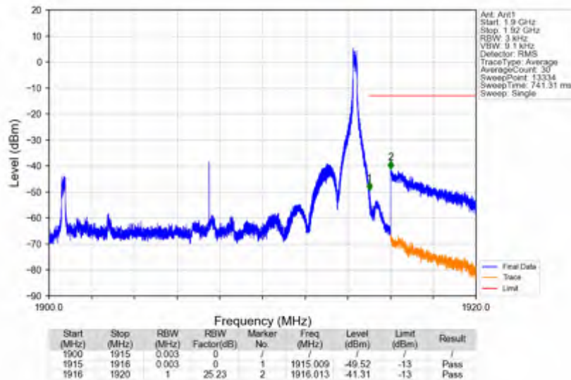
n25_15kHz_SISO_NTNV_15MHz_DFT-s-OFDM QPSK_1907.5MHz_Inner_1RB_Right
