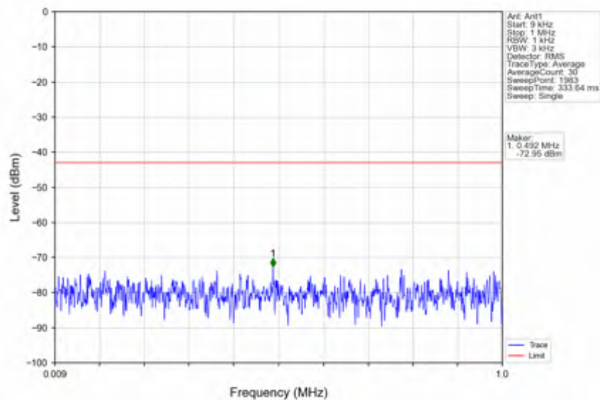
n25_15kHz_SISO_NTNV_5MHz_CP-OFDM QPSK_1852.5MHz_Outer_Full
