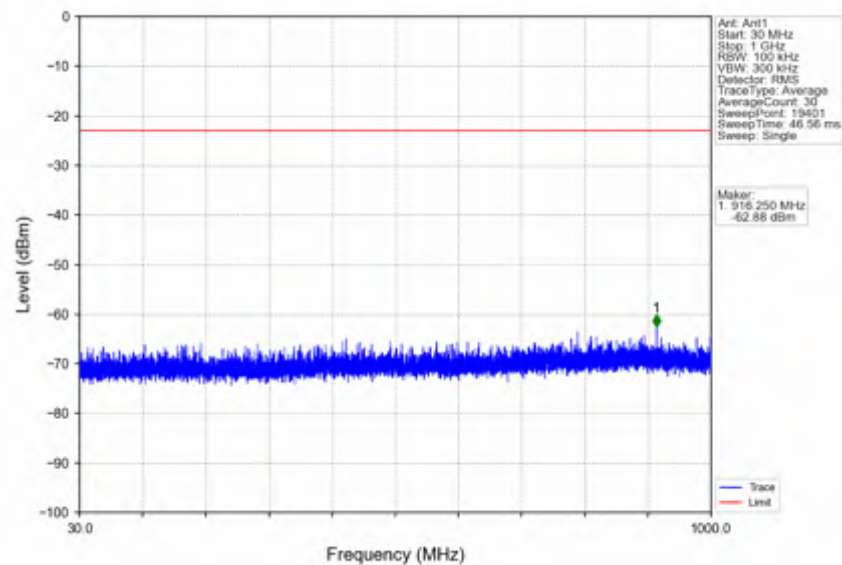
n25_15kHz_SISO_NTNV_10MHz_CP-OFDM_QPSK_1855MHz_Outer_Full
