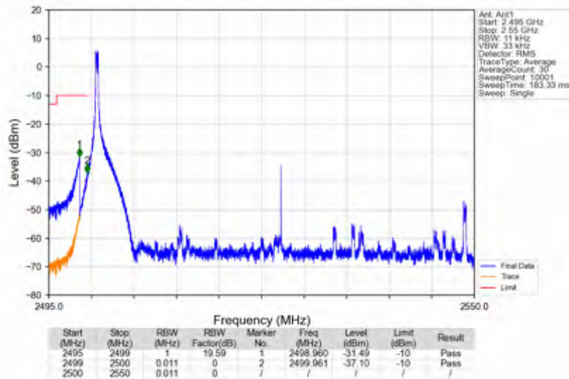
n7_30kHz_SISO_NTNV_50MHz_DFT-s-OFDM QPSK_2525MHz_Edge_1RB_Left
