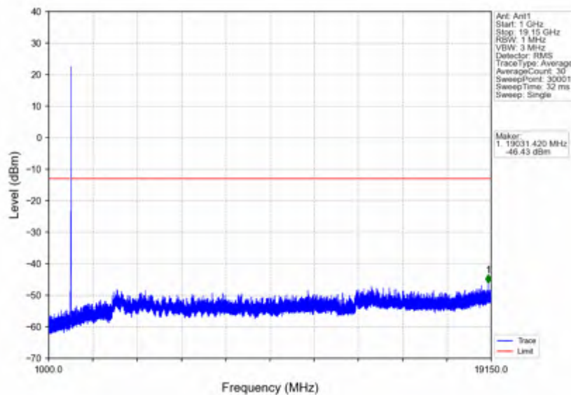
n25_15kHz_SISO_NTNV_10MHz_DFT-s-OFDM QPSK_1855MHz_Edge_1RB_Left
