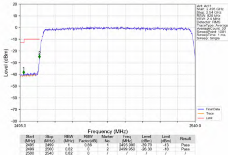
n7_30kHz_SISO_NTNV_40MHz_CP-OFDM QPSK_2520MHz_Outer_Full
