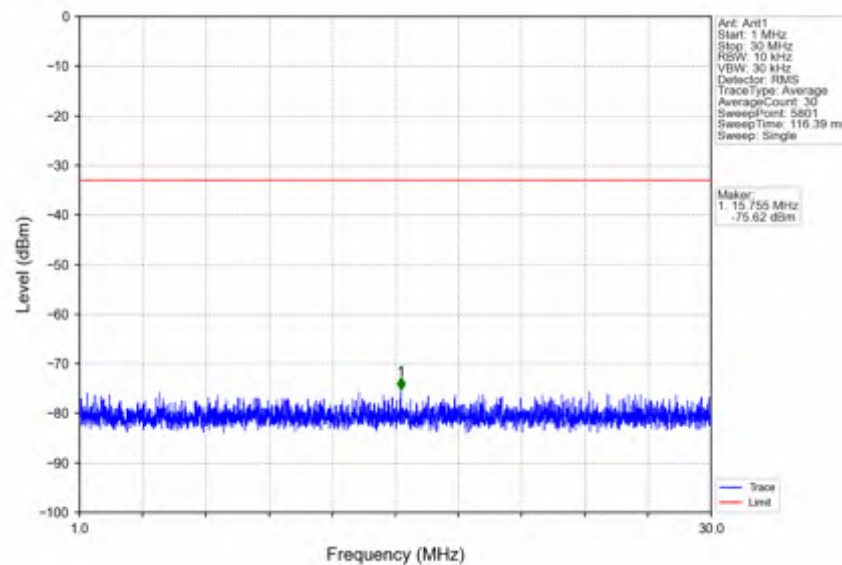
n25_15kHz_SISO_NTNV_5MHz_CP-OFDM QPSK_1912.5MHz_Inner_1RB_Right
