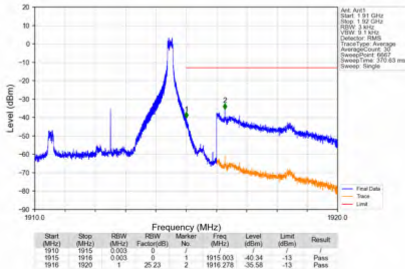
n25_15kHz_SISO_NTNV_5MHz_CP-OFDM_QPSK_1912.5MHz_Inner_1RB_Right
