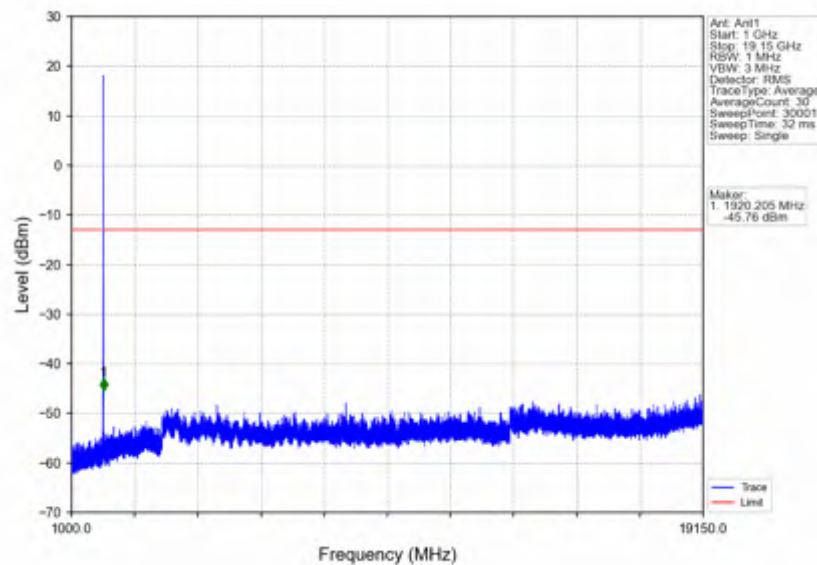
n25_15kHz_SISO_NTNV_5MHz_DFT-s-OFDM_PI/2_BPSK_1912.5MHz_Outer_Full
