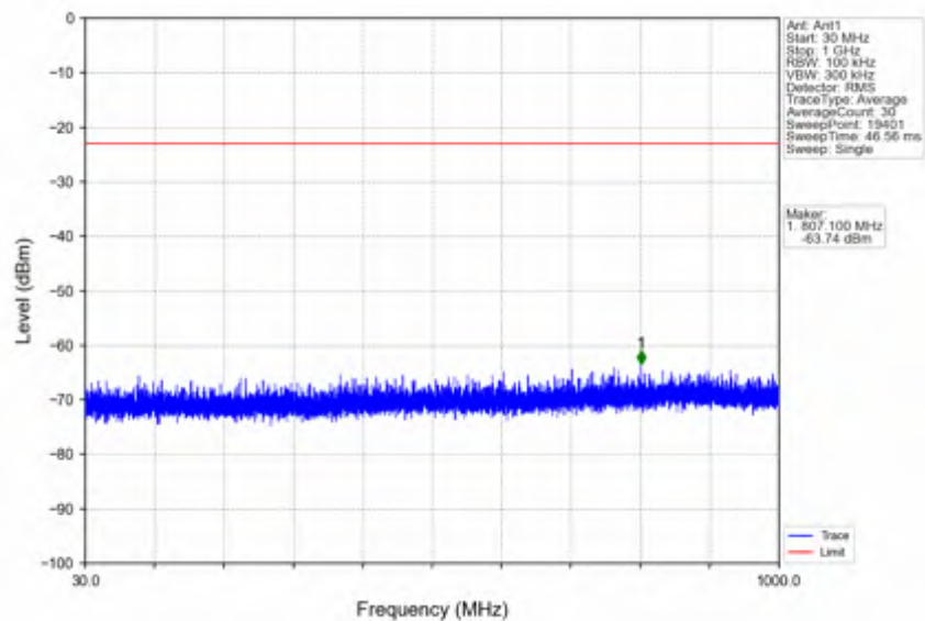
n25_15kHz_SISO_NTNV_5MHz_CP-OFDM QPSK_1852.5MHz_Edge_1RB_Left
