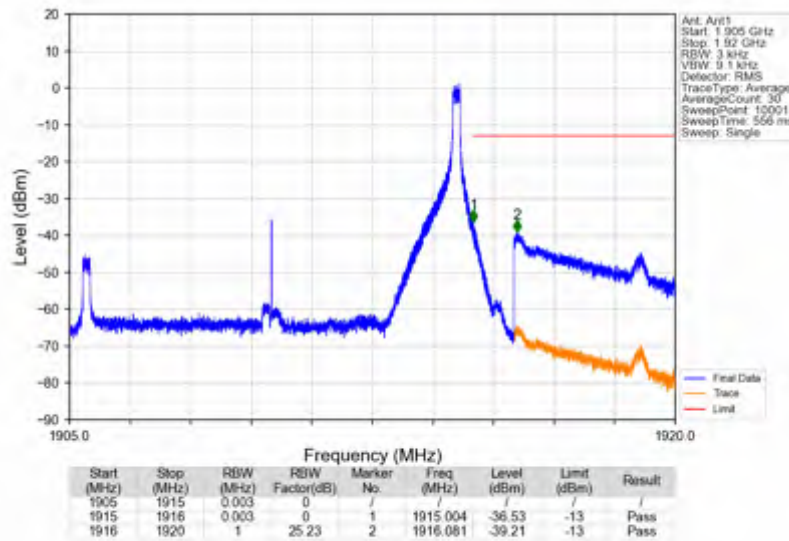
n25_15kHz_SISO_NTNV_10MHz_CP-OFDM_QPSK_1910MHz_Edge_1RB_Right
