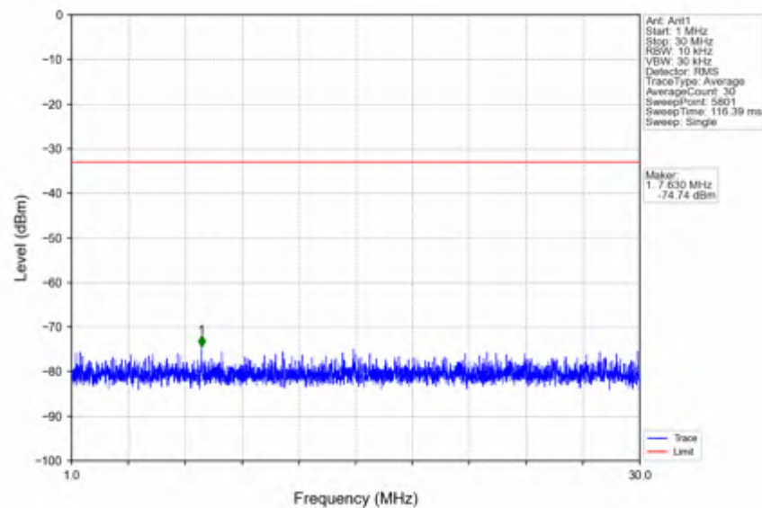
n25_15kHz_SISO_NTNV_10MHz_DFT-s-OFDM_PI/2_BPSK_1910MHz_Outer_Full
