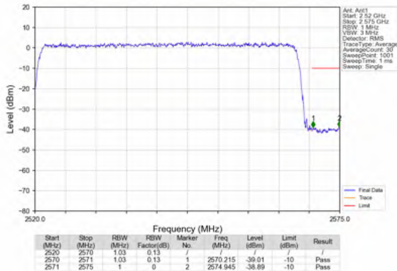
n7_30kHz_SISO_NTNV_50MHz_DFT-s-OFDM QPSK_2545MHz_Outer_Full
