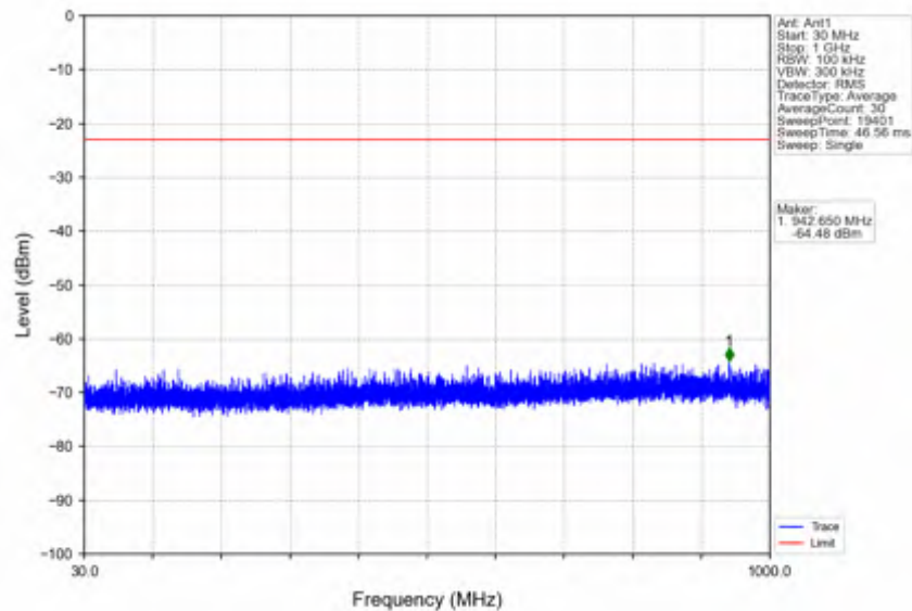
n25_15kHz_SISO_NTNV_5MHz_CP-OFDM_QPSK_1882.5MHz_Edge_1RB_Left
