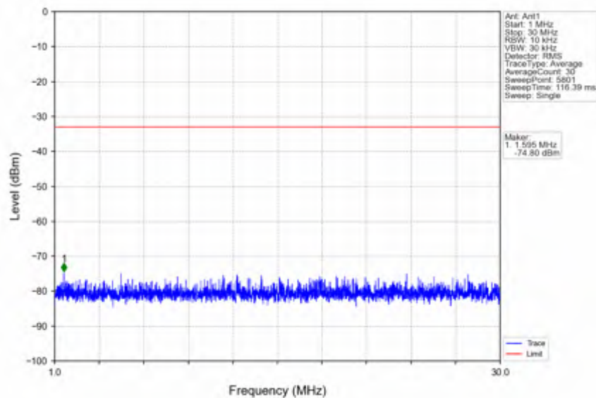
n25_15kHz_SISO_NTNV_15MHz_CP-OFDM QPSK_1857.5MHz_Edge_1RB_Left
