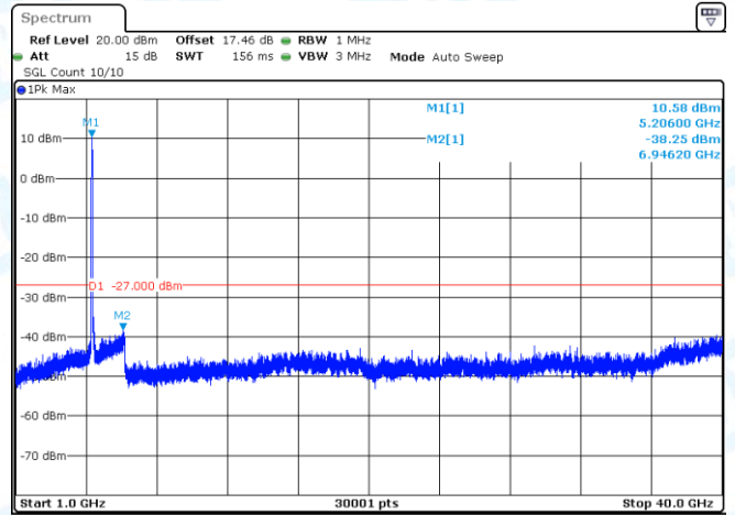
11AX80-CDD-Ant2-5210-1000~40000-PASS
