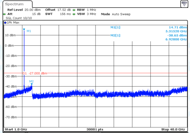
11AX20-CDD-Ant2-5320-1000~40000-PASS
