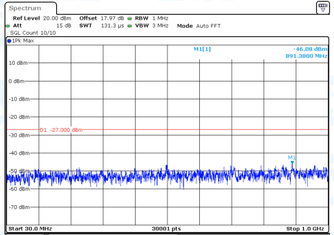
11AX40-CDD-Ant2-5670-30~1000-PASS
