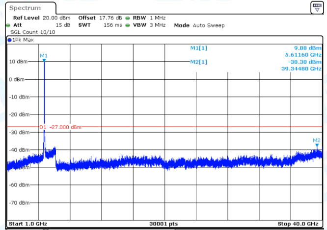
11AX80-CDD-Ant2-5610-1000~40000-PASS
