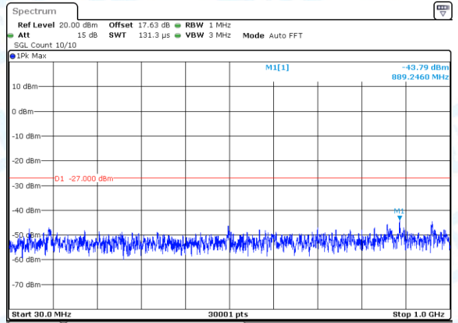
11AX20-CDD-Ant2-5580-30~1000-PASS
