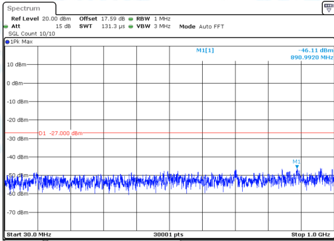
11AX20-CDD-Ant1-5580-30~1000-PASS
