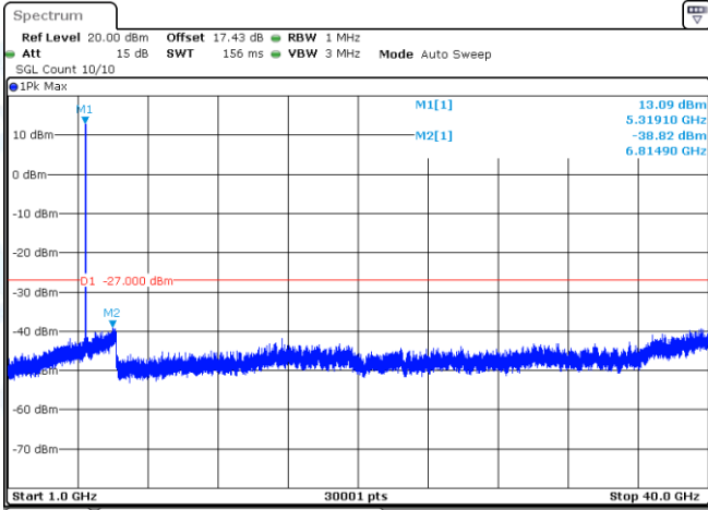
11AX20-CDD-Ant1-5320-1000~40000-PASS
