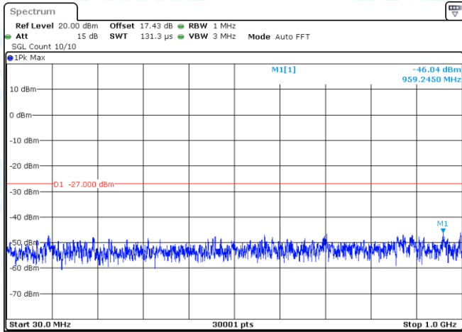
11AX40-CDD-Ant1-5310-30~1000-PASS
