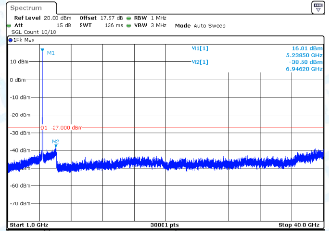
11AX20-CDD-Ant2-5240-1000~40000-PASS
