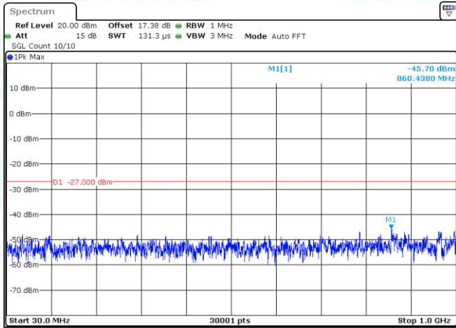
11AX20-CDD-Ant1-5200-30~1000-PASS
