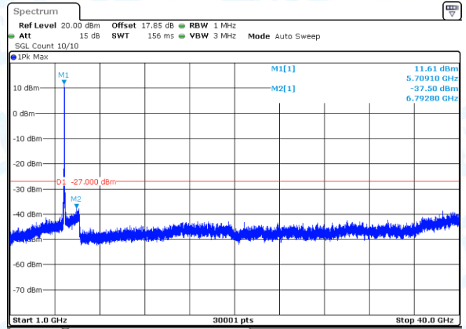
11AX40-CDD-Ant2-5710-1000~40000-PASS
