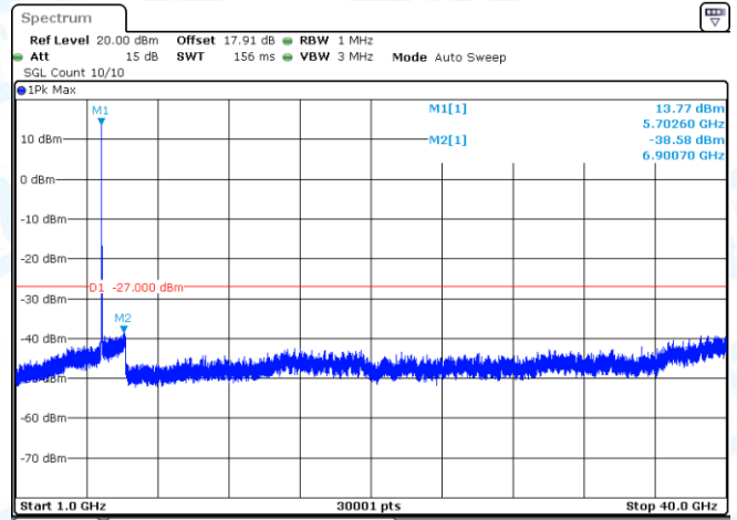
11AX20-CDD-Ant2-5700-1000~40000-PASS
