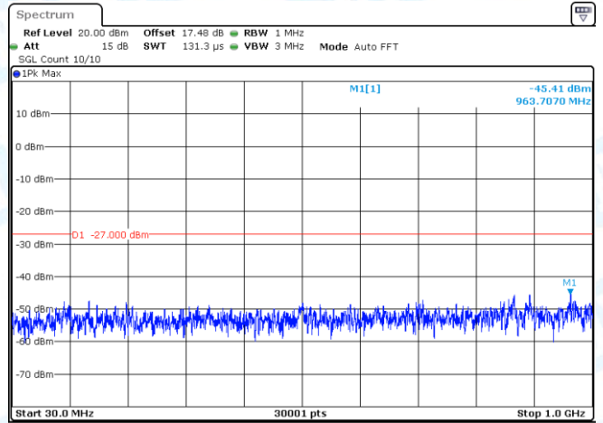
11AX20-CDD-Ant2-5200-30~1000-PASS
