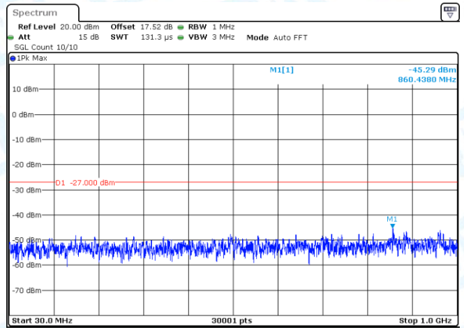
11AX20-CDD-Ant2-5280-30~1000-PASS
