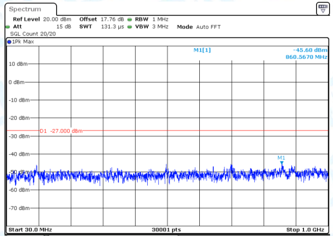
11AX40-CDD-Ant2-5795-30~1000-PASS
