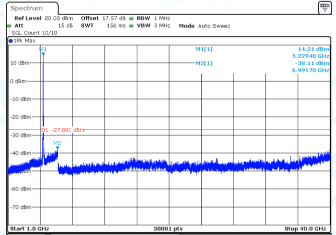
11AX40-CDD-Ant2-5230-1000~40000-PASS
