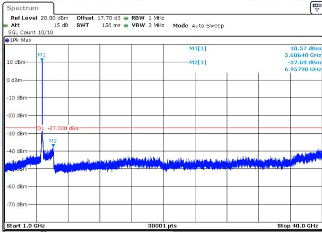
11AX80-CDD-Ant1-5610-1000~40000-PASS
