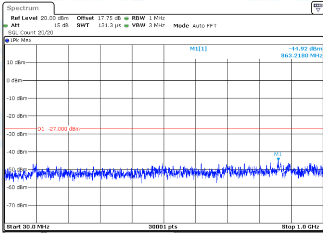
11AX20-CDD-Ant1-5745-30~1000-PASS
