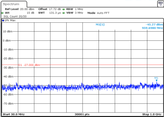
11AX80-CDD-Ant1-5775-30~1000-PASS
