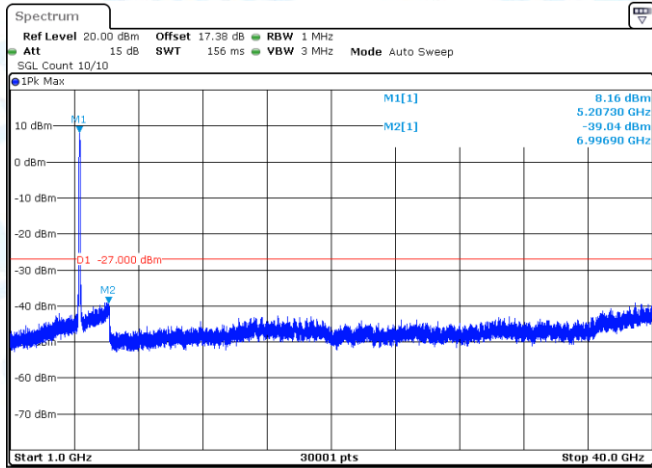
11AX80-CDD-Ant1-5210-1000~40000-PASS
