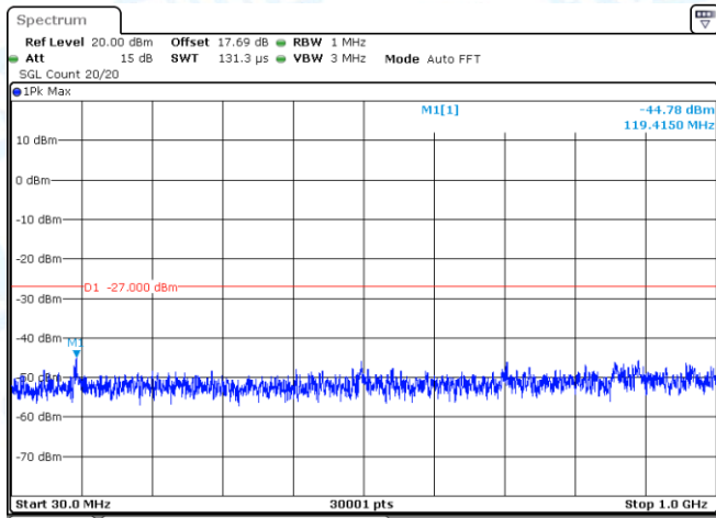
11AX40-CDD-Ant1-5795-30~1000-PASS
