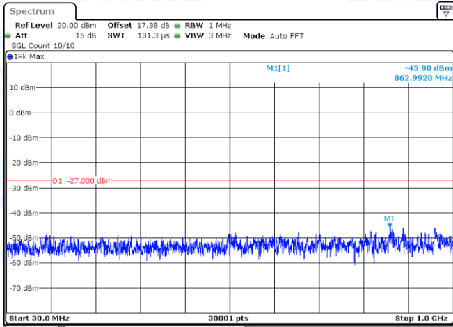
11AX40-CDD-Ant1-5190-30~1000-PASS
