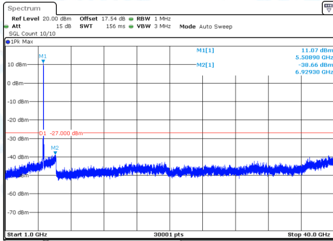
11AX40-CDD-Ant1-5510-1000~40000-PASS
