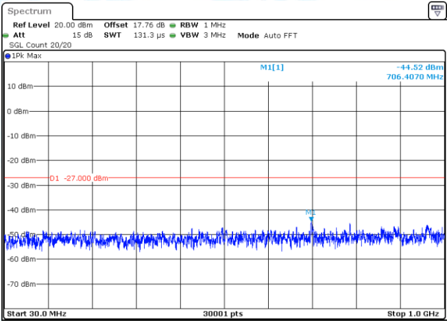
11AX80-CDD-Ant2-5775-30~1000-PASS
