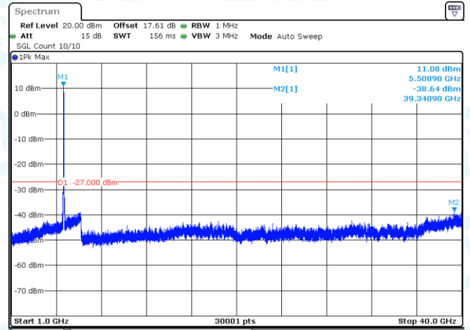
11AX40-CDD-Ant2-5510-1000~40000-PASS
