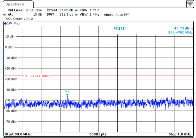
11AX80-CDD-Ant2-5530-30~1000-PASS
