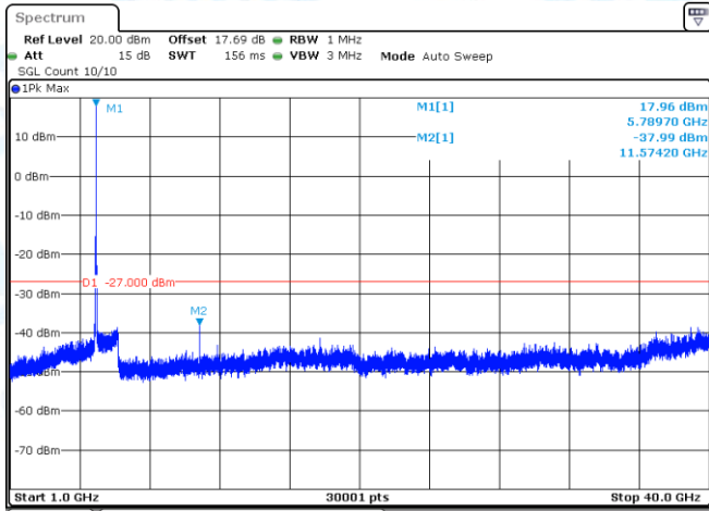
11AX20-CDD-Ant1-5785-1000~40000-PASS
