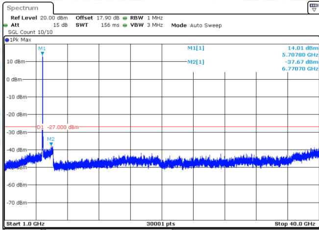
11AX40-CDD-Ant1-5710-1000~40000-PASS
