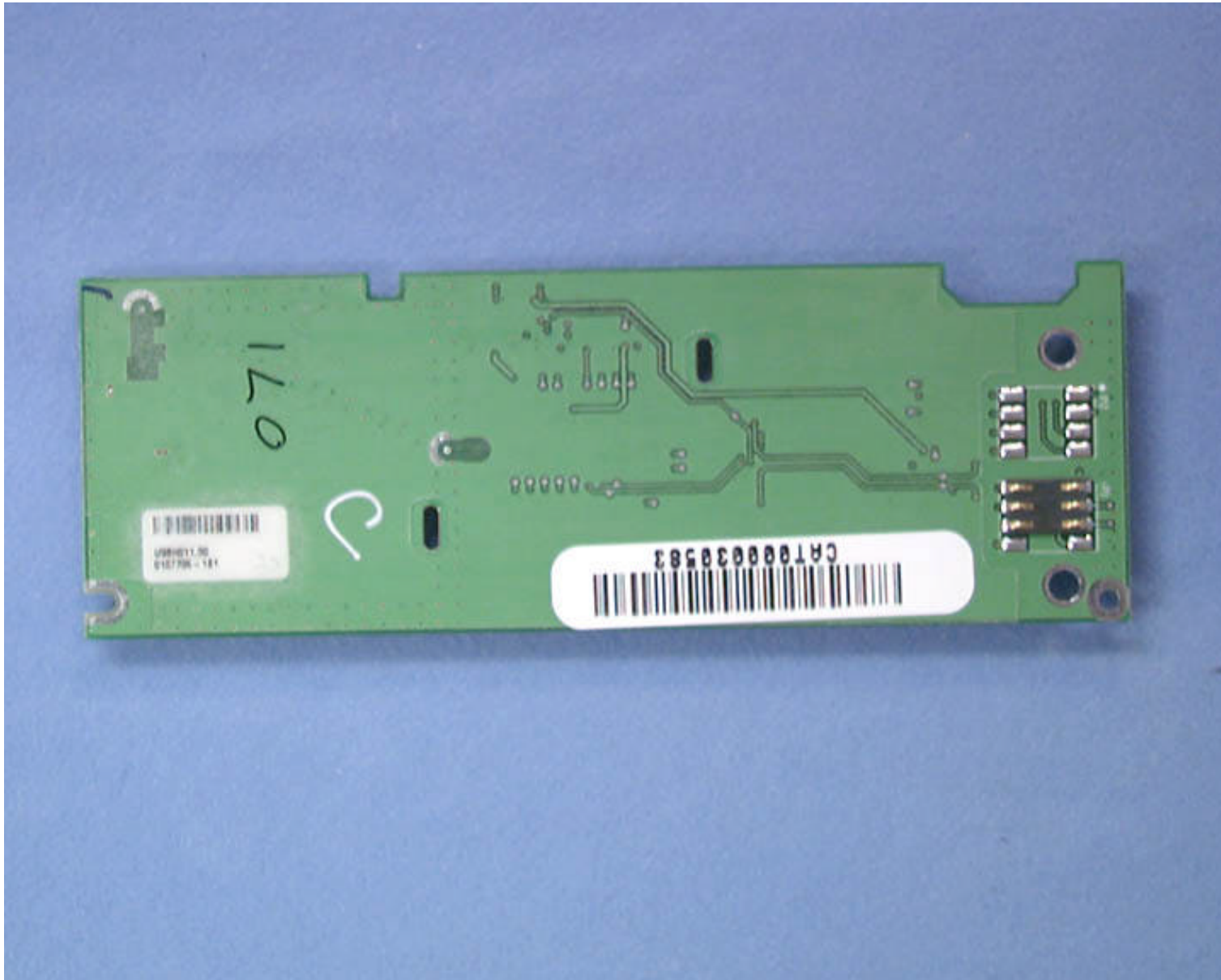
PCB – Back
