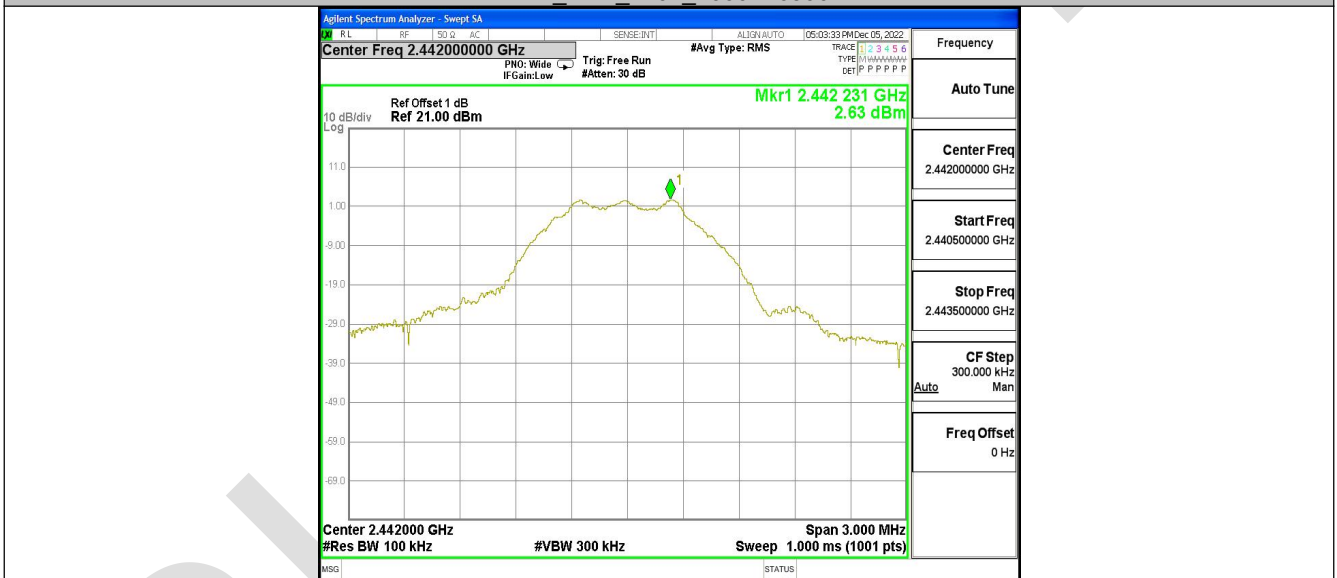
BLE_Ant1_2442_0~Reference
