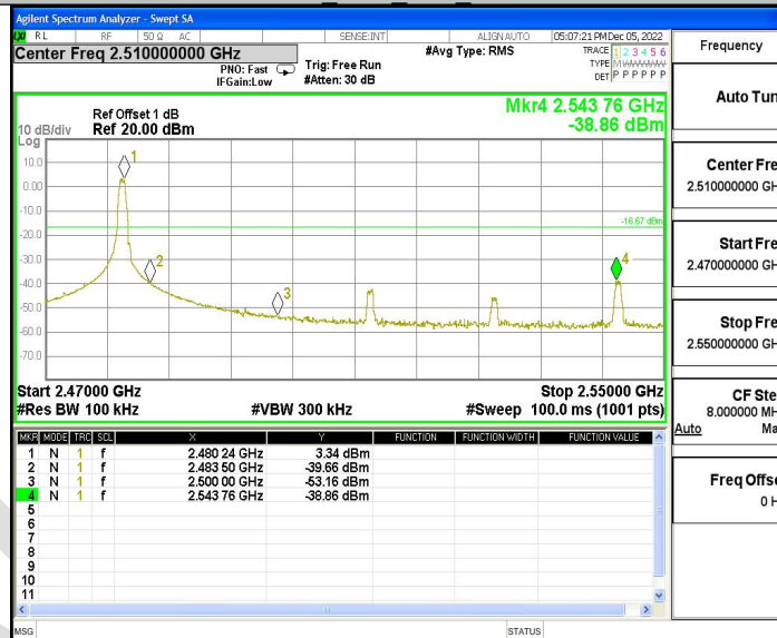
BLE_Ant1_High_2480
