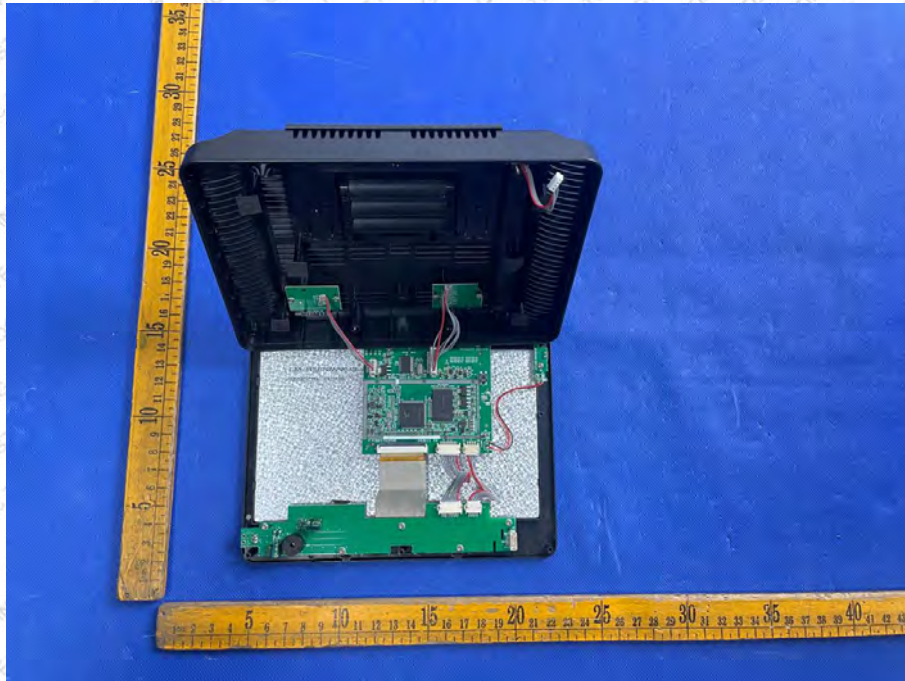
915MHz Antenna
