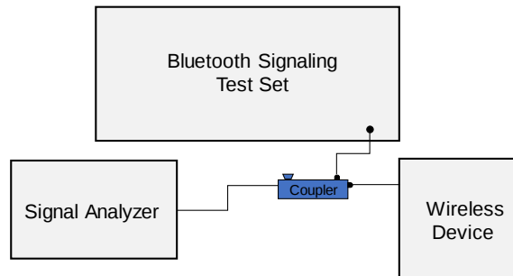
Figure 8-8 Power Measurement Setup
