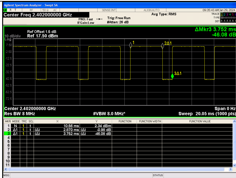
GFSK(DH5)_Channel 0
