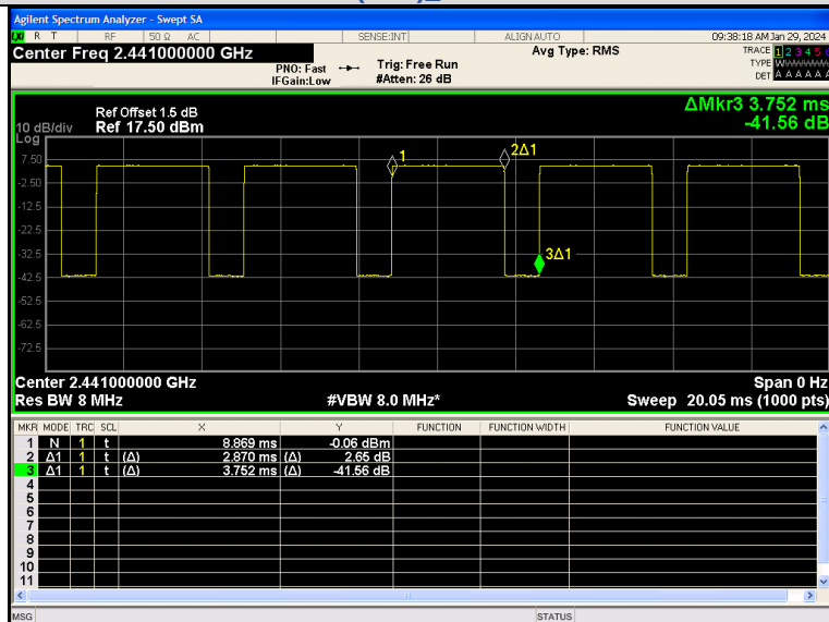
GFSK(DH5)_Channel 39
