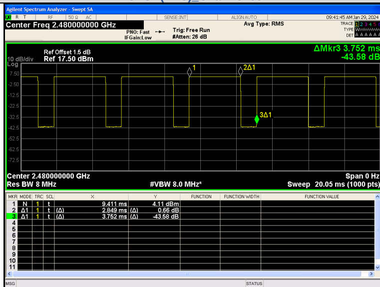
GFSK(DH5)_Channel 78
