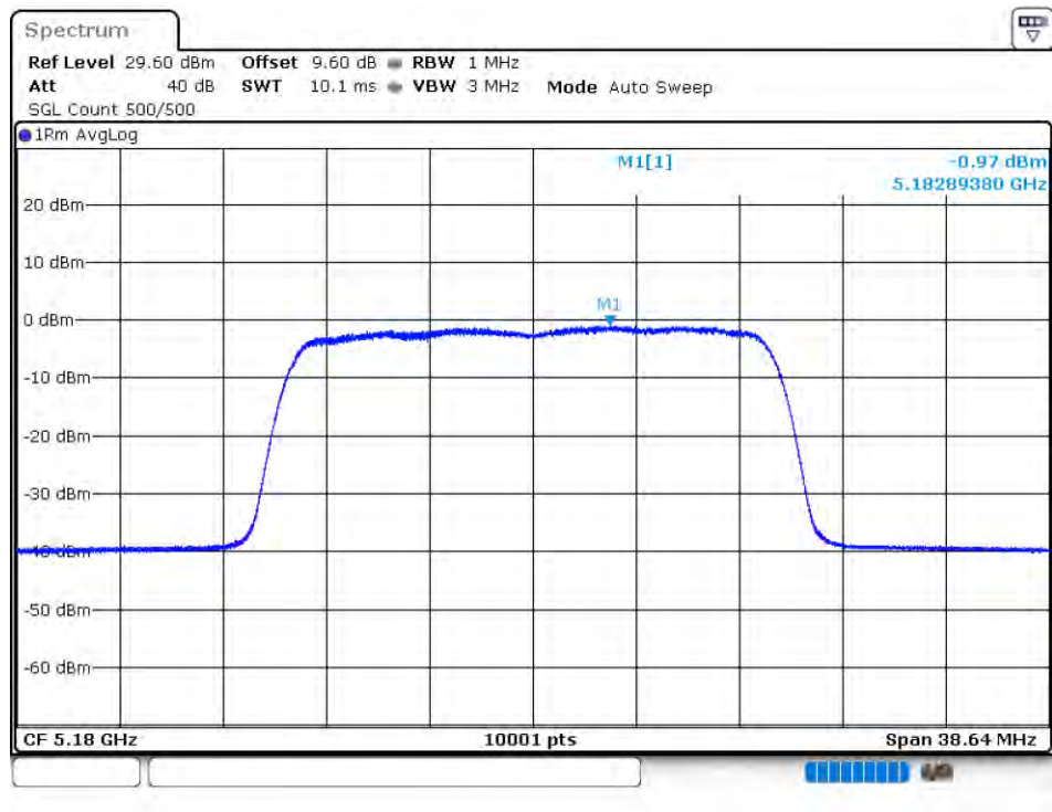
PSD NVNT 802.11ac20 5180MHz Ant2
