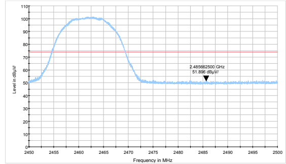
802.11b-Channel 11: Average
