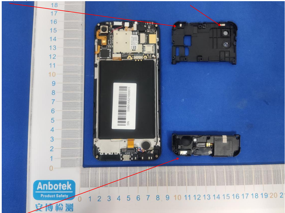
2G,3G,4G Main ANT
