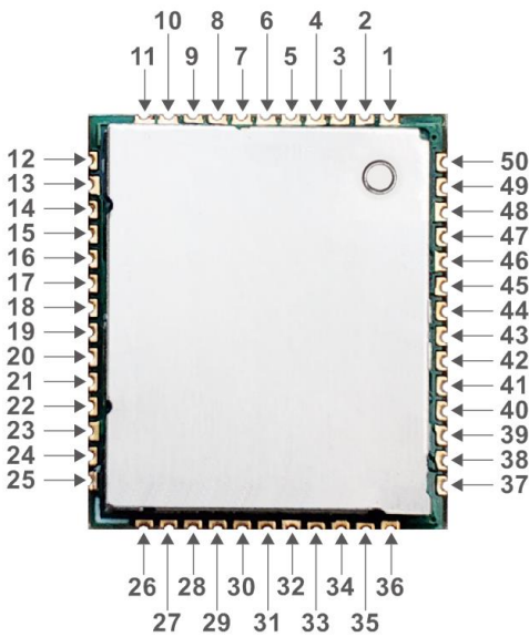
Figure 4-Top view
