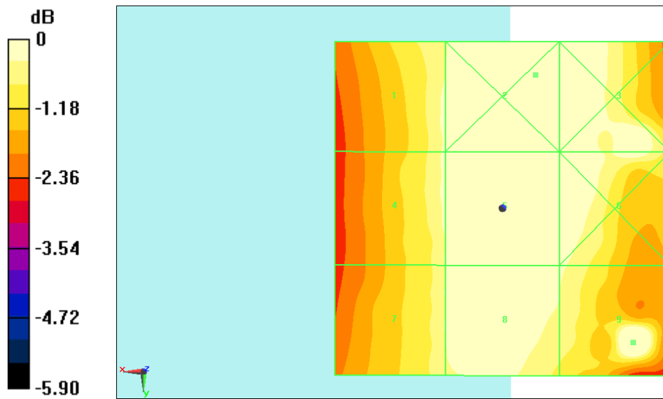
Fig B.3 HAC RF E-Field CDMA BC0 Middle
