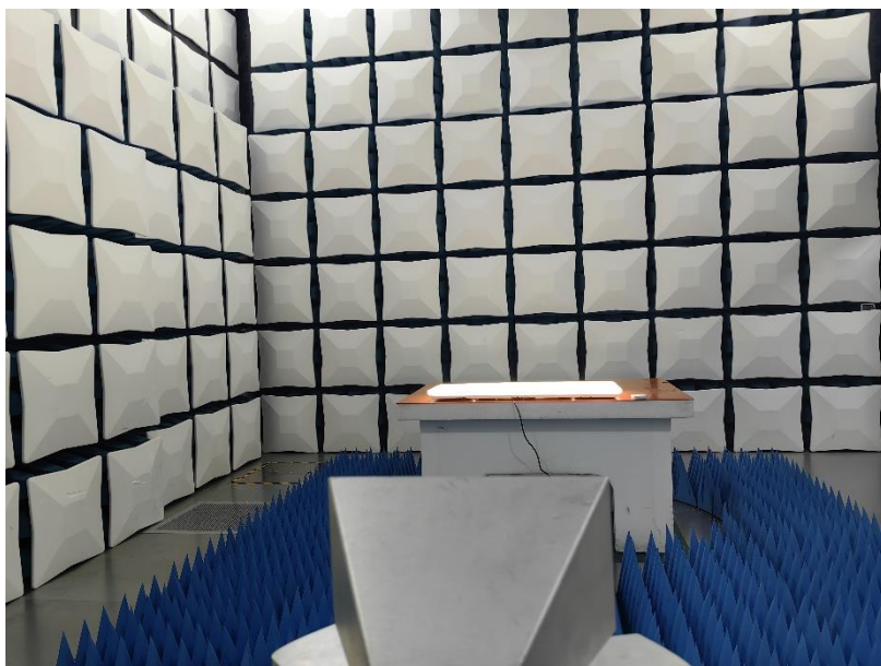
Photograph 3: Set-up for measurement of radiated emission, Above 1G
