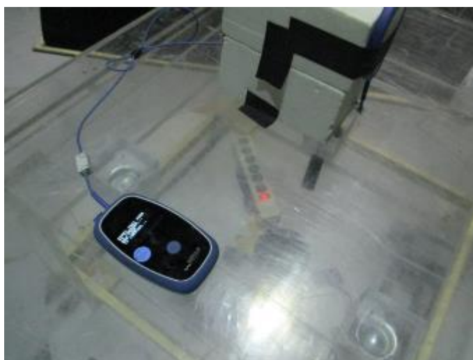
Radiated Emissions / Bandwidth / Field Strength Setup
