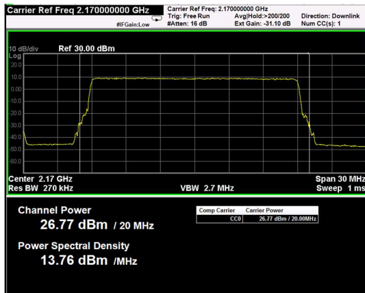
Channel: TOP, Modulation: QPSK, BW=20MHz, Channel Power
