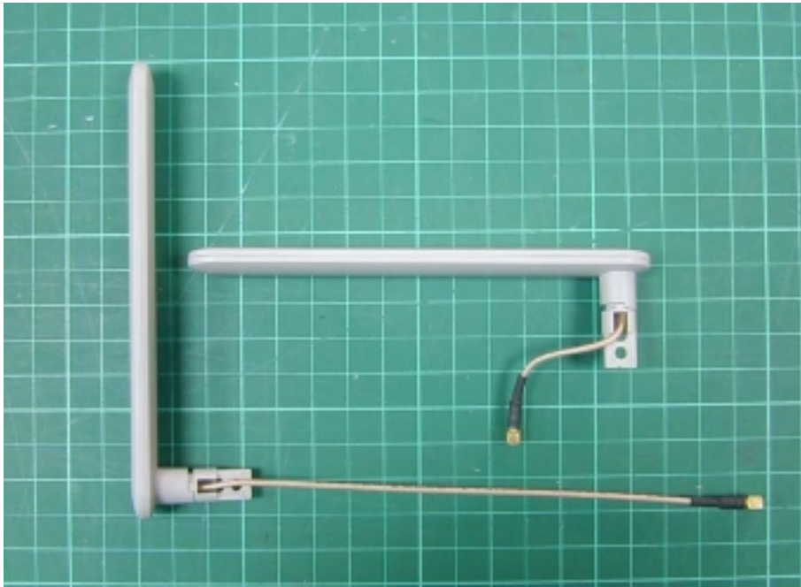
Photo 1: Antenna photo
