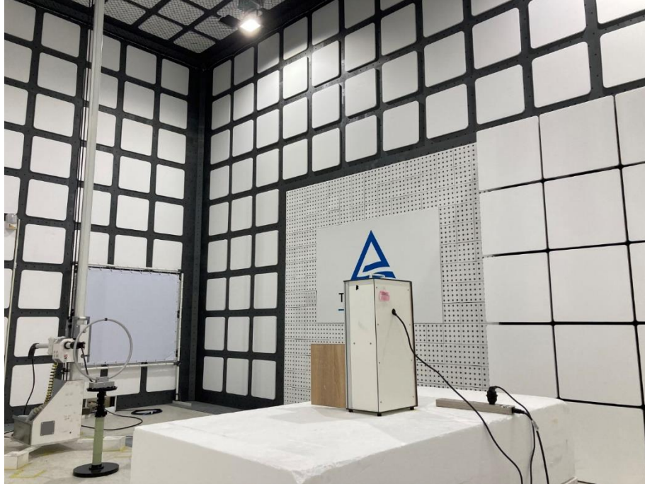
Photograph 7: Test Setup for Spurious Emissions (Back View 1)
