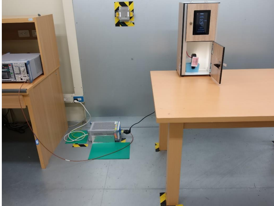
Photograph 9: Test Setup for Mains Conducted Emissions (Front View)
