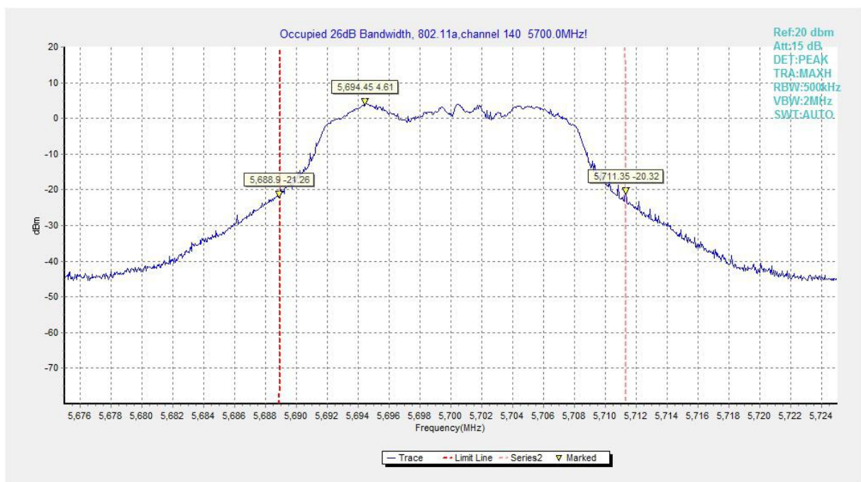
Fig.58 Occupied 26dB Bandwidth (802.11a, 5700MHz)
