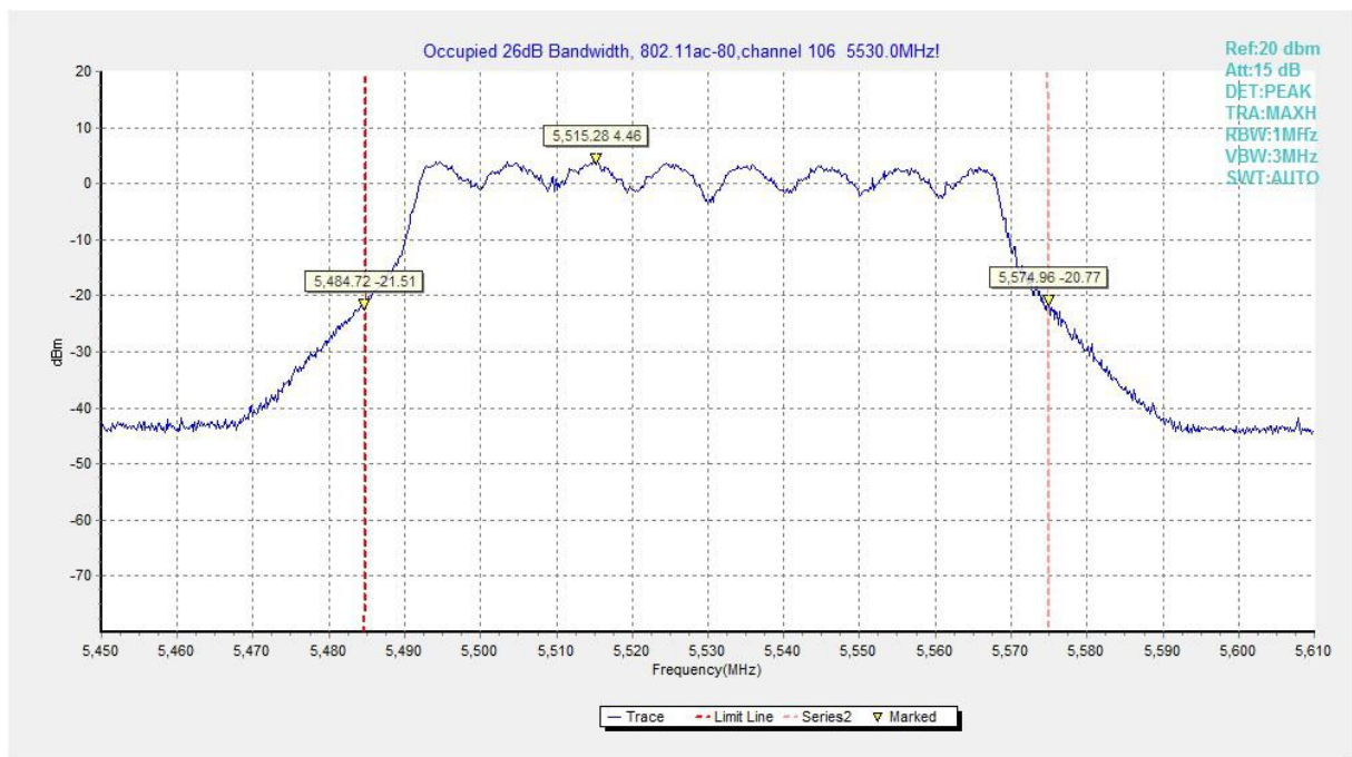
Fig.77 Occupied 26dB Bandwidth (802. 11ac-HT80, 5530MHz)
