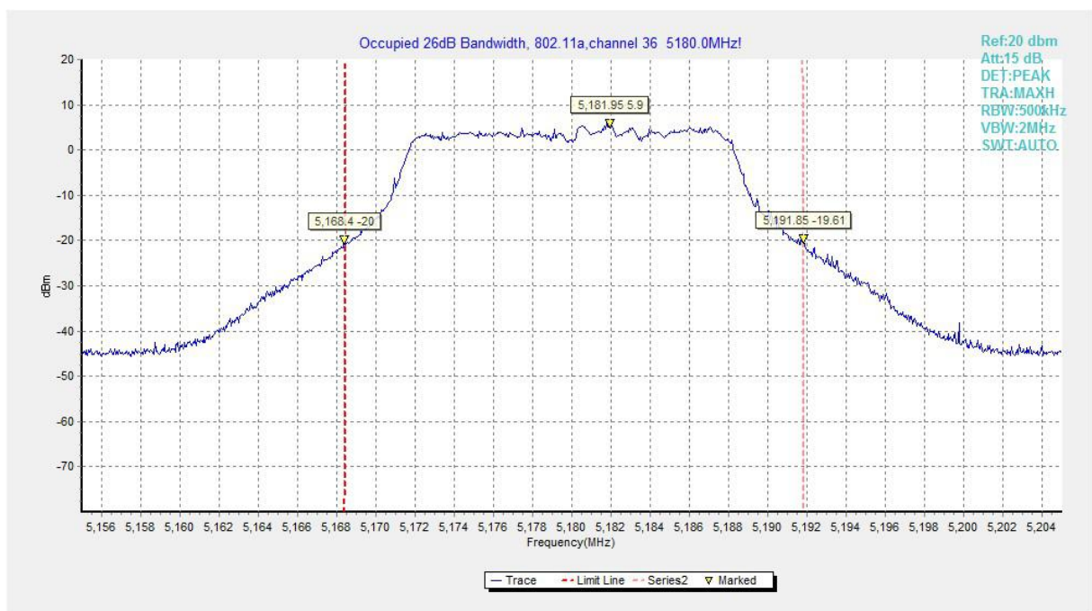
Fig.50 Occupied 26dB Bandwidth (802.11a, 5180MHz)
