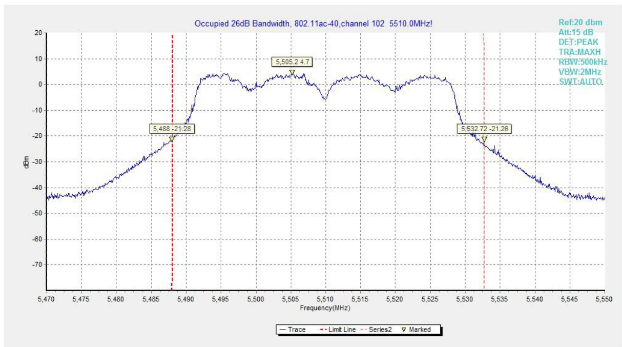
Fig.72 Occupied 26dB Bandwidth (802.11ac-HT40, 5510MHz)
