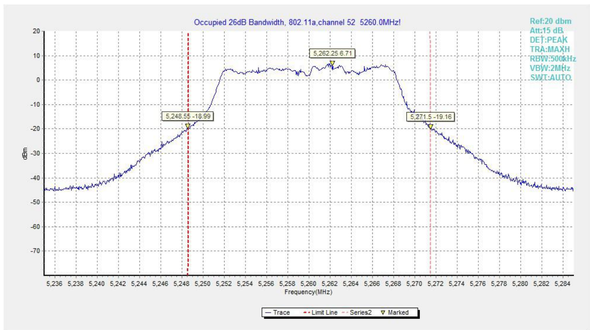
Fig.53 Occupied 26dB Bandwidth (802.11a, 5260MHz)
