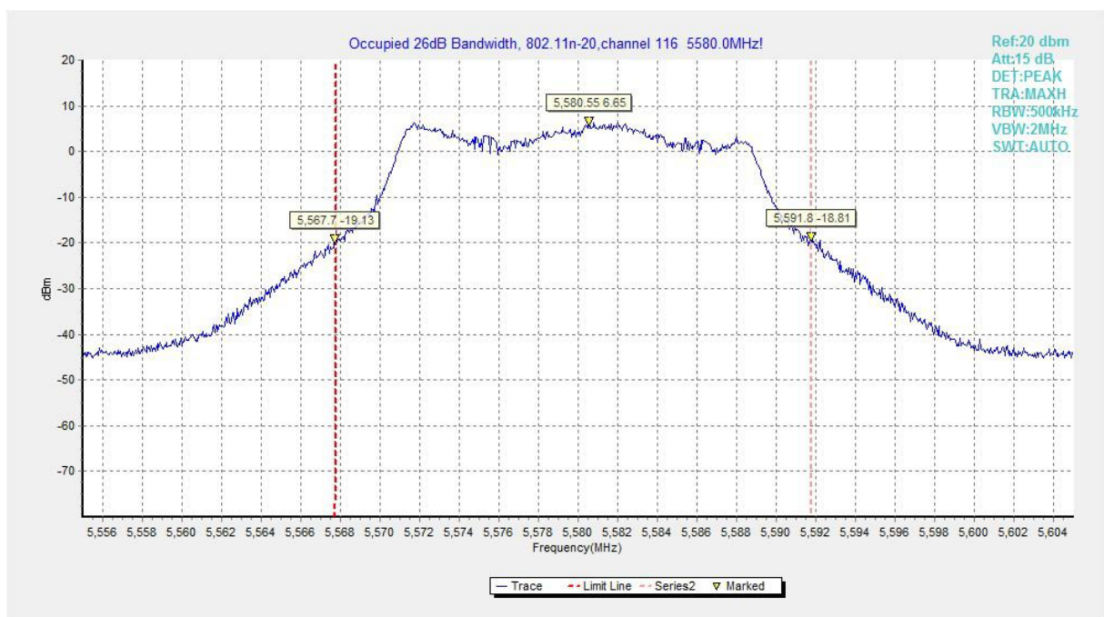
Fig.66 Occupied 26dB Bandwidth (802. 11n-HT20, 5580MHz)
