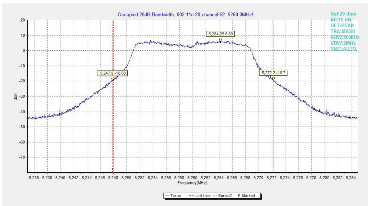
Fig.62 Occupied 26dB Bandwidth (802.11n-HT20, 5260MHz)
