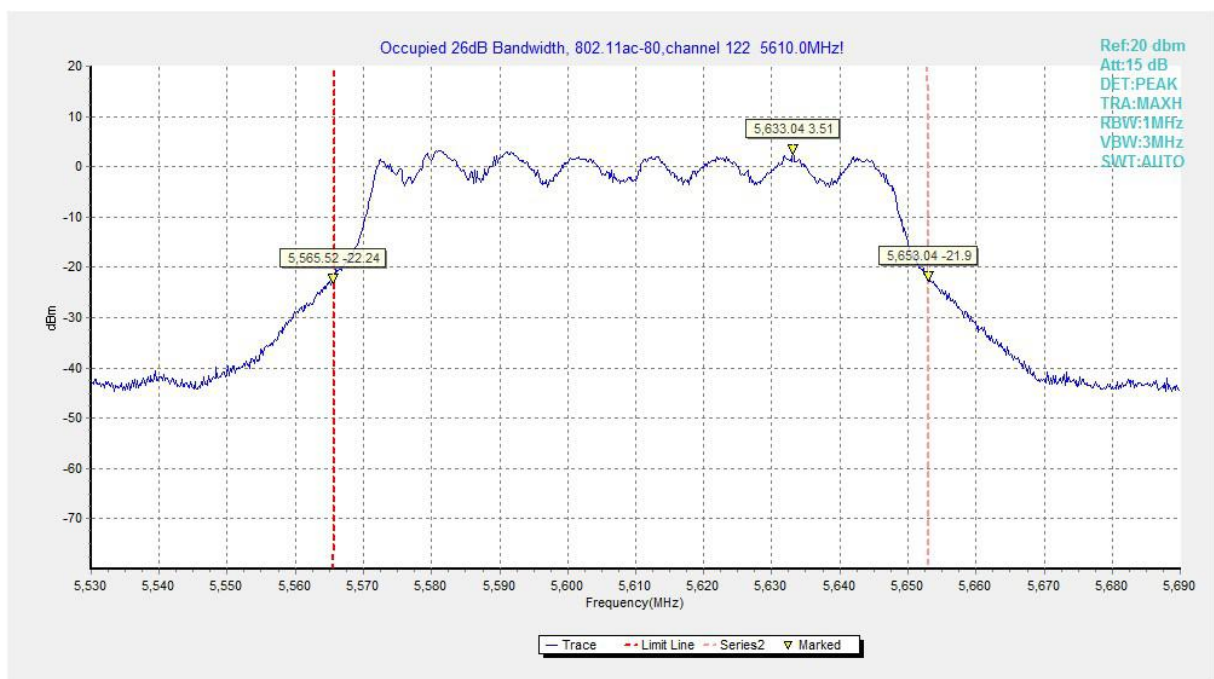
Fig.78 Occupied 26dB Bandwidth (802. 11ac-HT80, 5610MHz)
