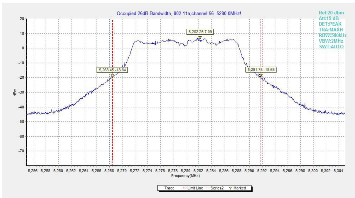
Fig.54 Occupied 26dB Bandwidth (802.11a, 5280MHz)
