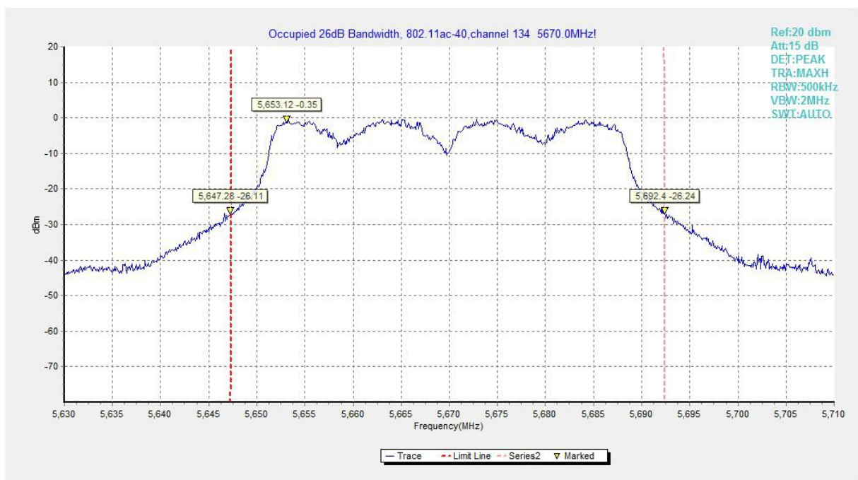
Fig.74 Occupied 26dB Bandwidth (802.11ac-HT40, 5670MHz)
