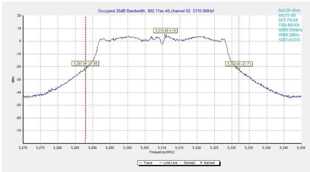
Fig.71 Occupied 26dB Bandwidth (802.11ac-HT40, 5310MHz)
