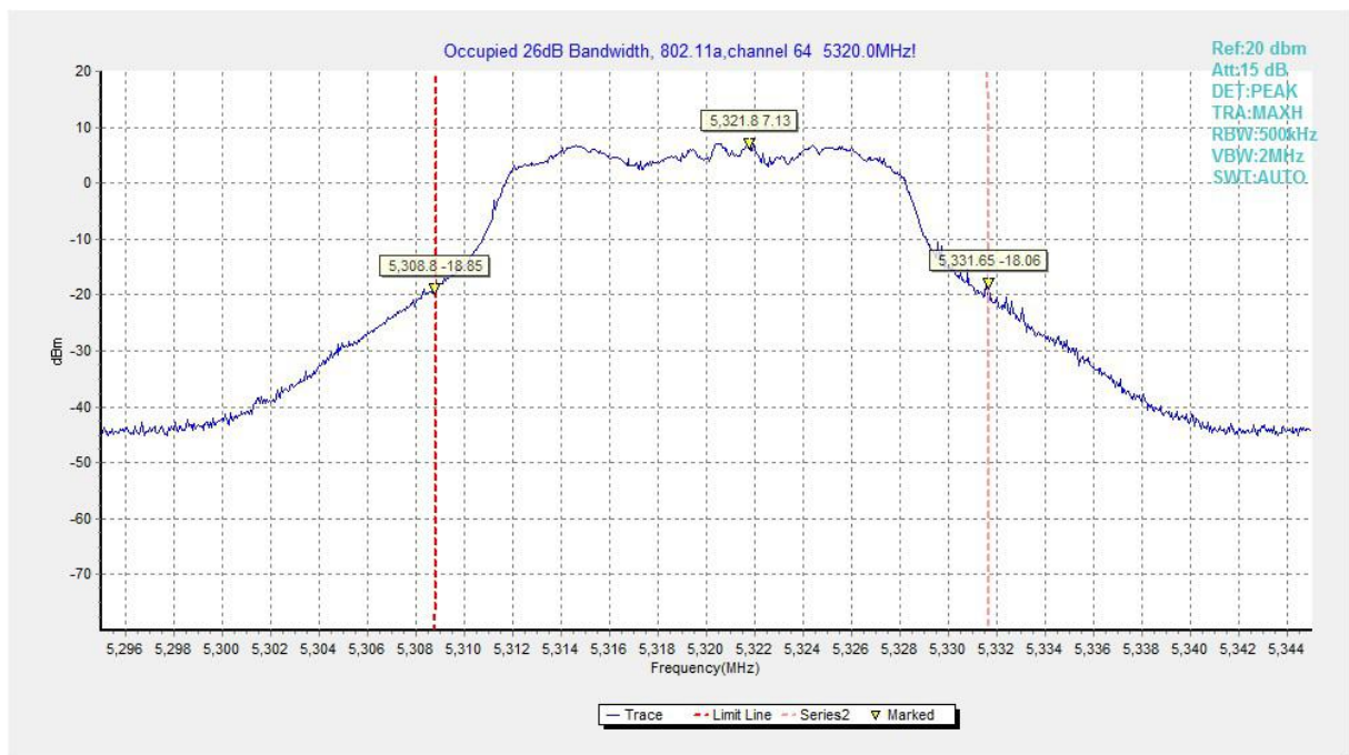
Fig.55 Occupied 26dB Bandwidth (802.11a, 5320MHz)
