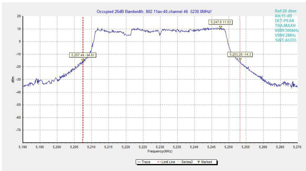
Fig.89 Occupied 26dB Bandwidth (802.11ax-HE40, 5230MHz)
