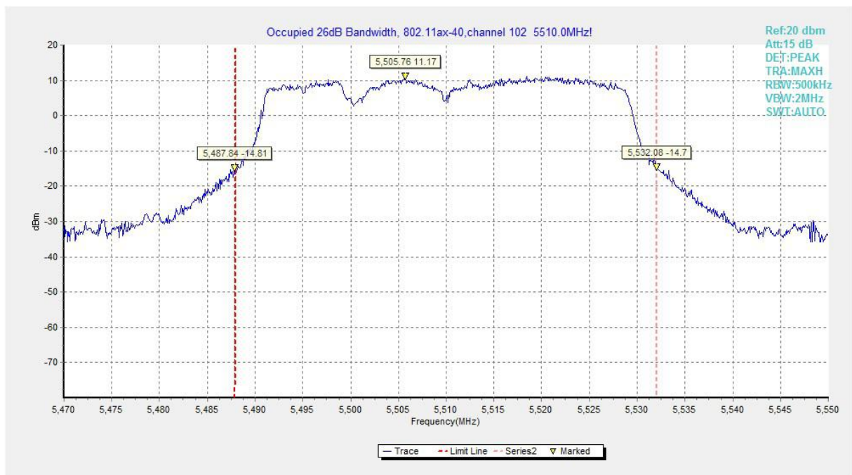
Fig.92 Occupied 26dB Bandwidth (802.11ax-HE40, 5510MHz)
