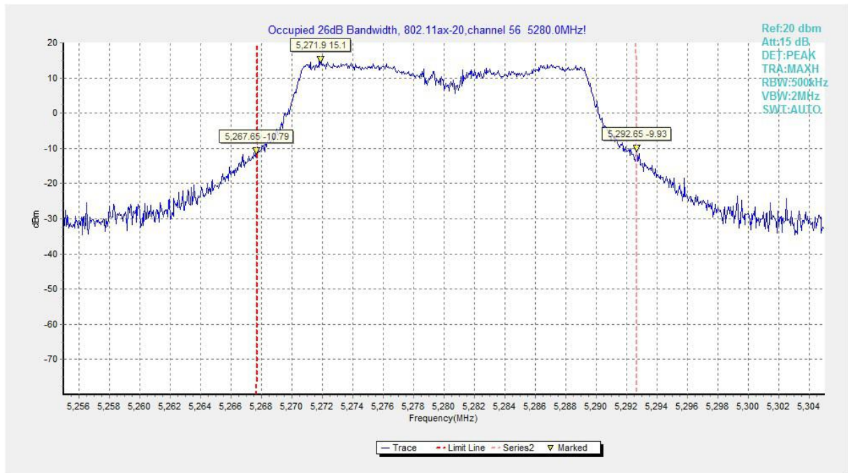
Fig.83 Occupied 26dB Bandwidth (802.11ax-HE20, 5280MHz)
