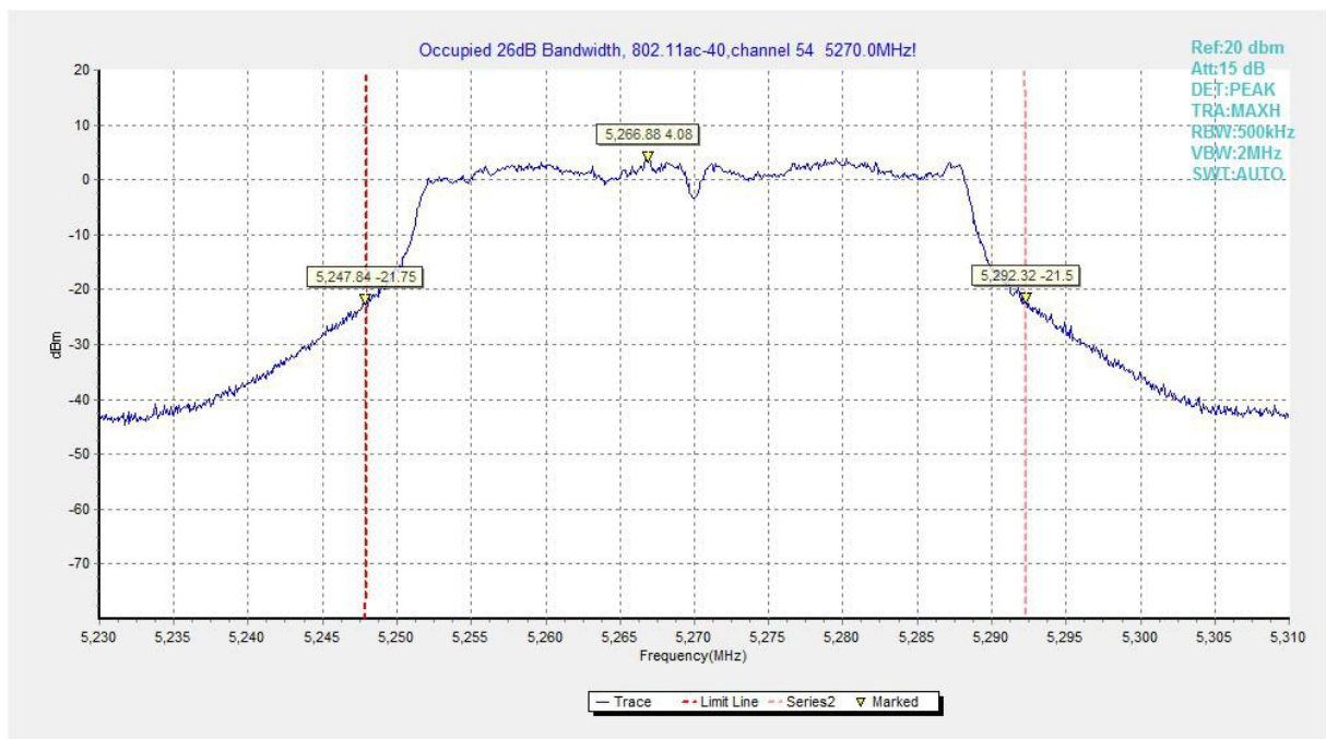
Fig.70 Occupied 26dB Bandwidth (802.11ac-HT40, 5270MHz)
