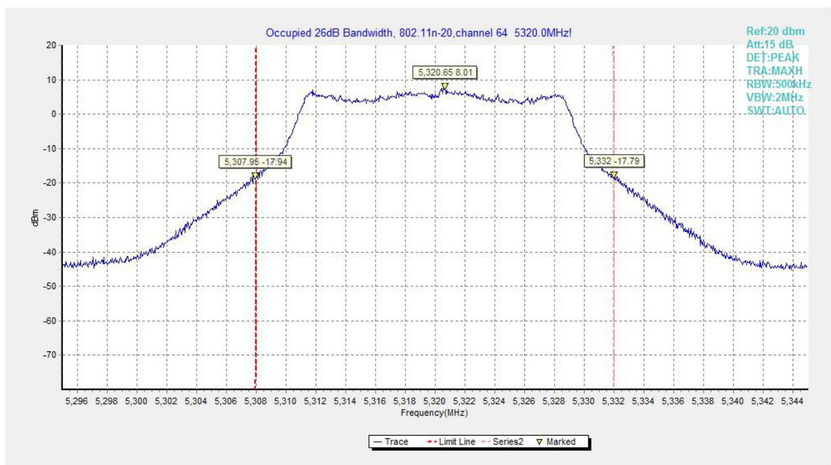
Fig.64 Occupied 26dB Bandwidth (802.11n-HT20, 5320MHz)
