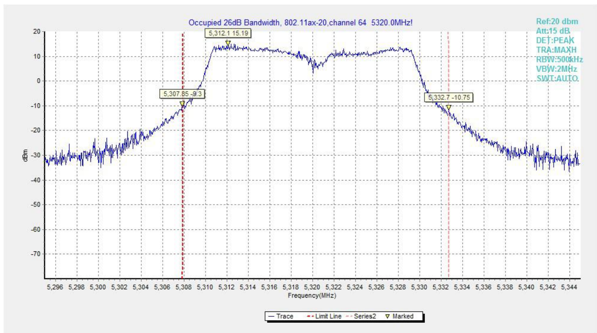
Fig.84 Occupied 26dB Bandwidth (802.11ax-HE20, 5320MHz)
