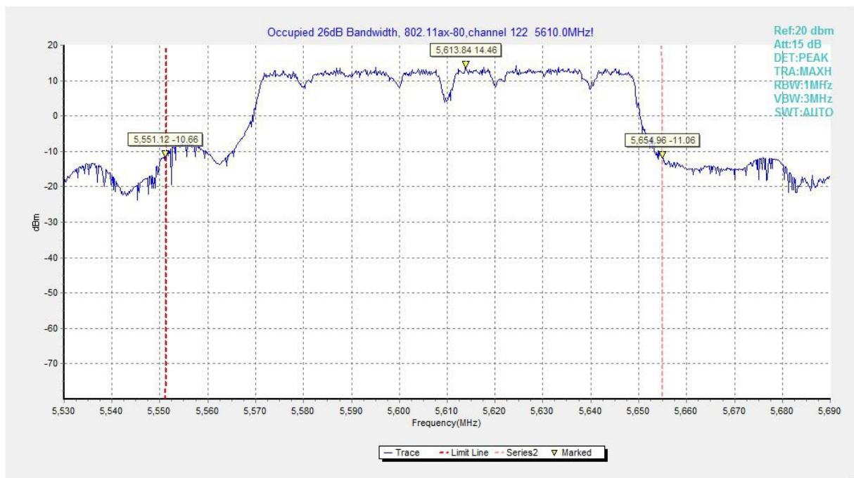
Fig.49 Occupied 26dB Bandwidth (802.11ax-HE80, 5610MHz)
