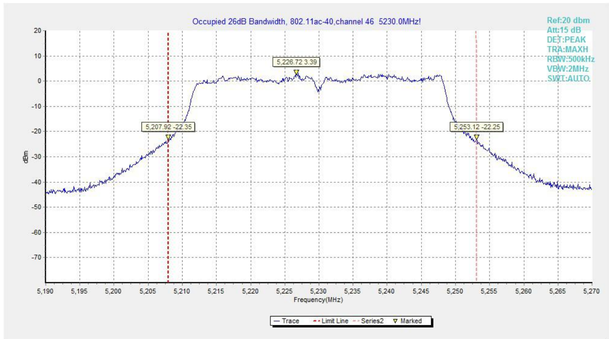
Fig.69 Occupied 26dB Bandwidth (802.11ac-HT40, 5230MHz)
