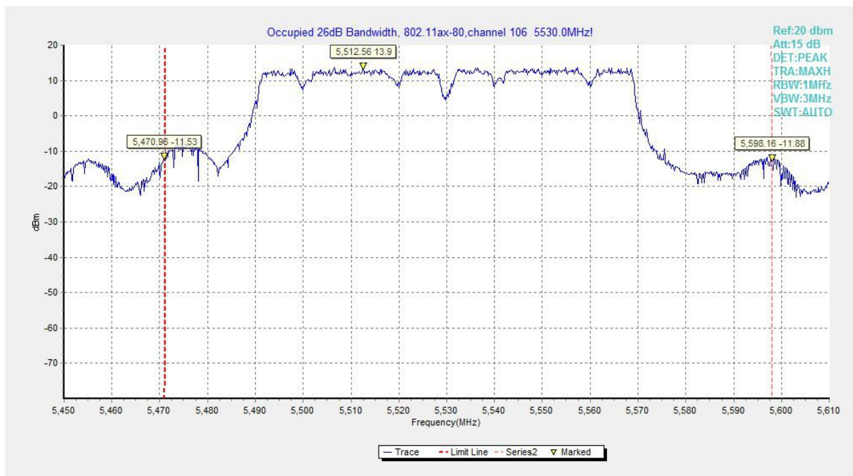
Fig.48 Occupied 26dB Bandwidth (802.11ax-HE80,5530MHz)
