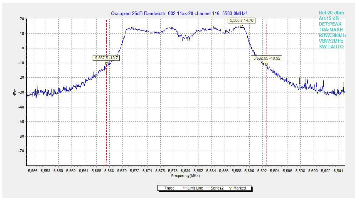
Fig.86 Occupied 26dB Bandwidth (802.11ax-HE20, 5580MHz)
