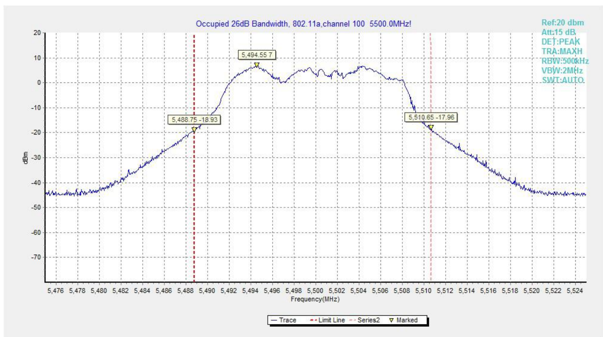
Fig.56 Occupied 26dB Bandwidth (802.11a, 5500MHz)
