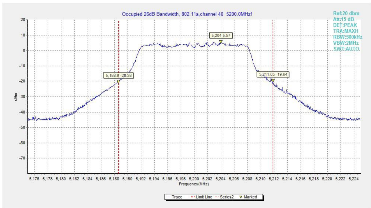
Fig.51 Occupied 26dB Bandwidth (802.11a, 5200MHz)
