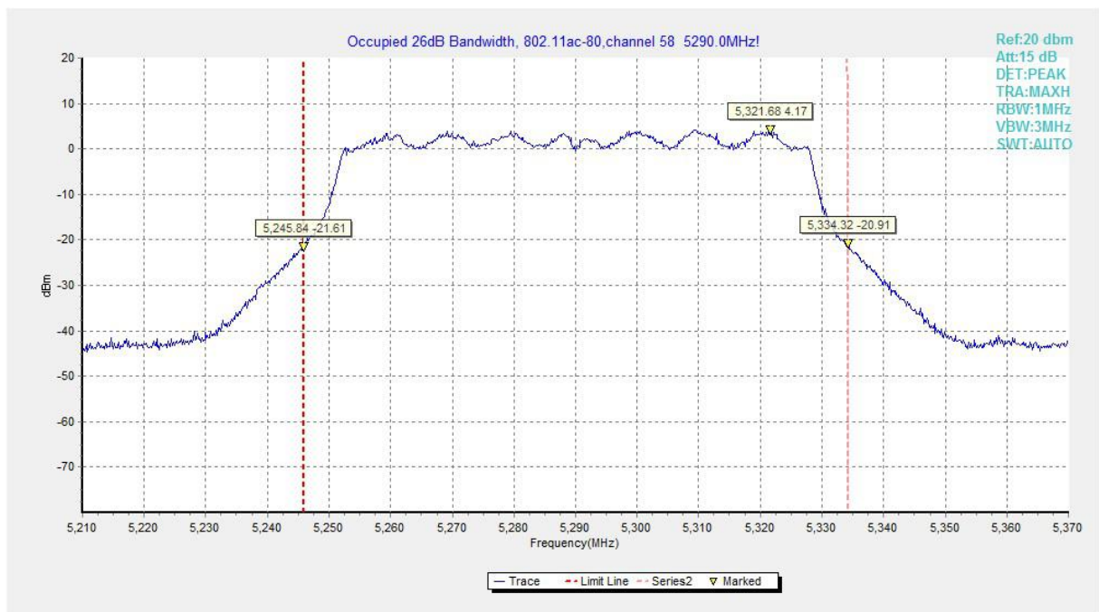
Fig.76 Occupied 26dB Bandwidth (802. 11ac-HT80, 5290MHz)
