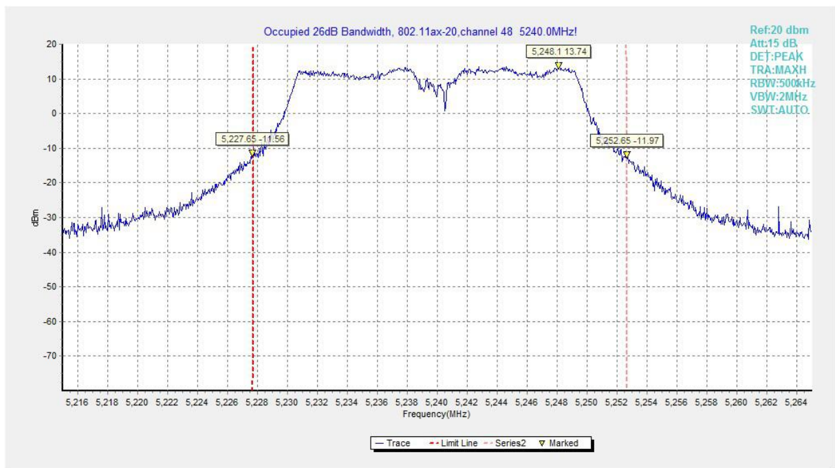
Fig.81 Occupied 26dB Bandwidth (802.11ax-HE20, 5240MHz)
