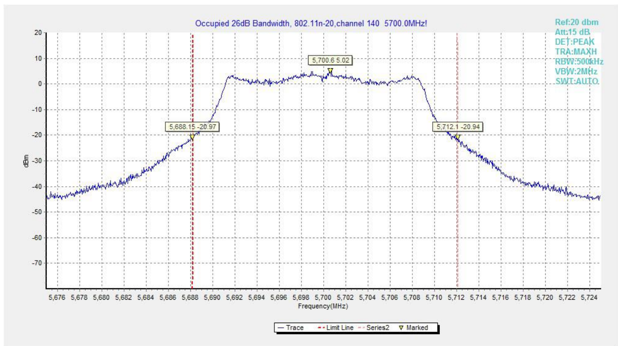
Fig.67 Occupied 26dB Bandwidth (802. 11n-HT20, 5700MHz)
