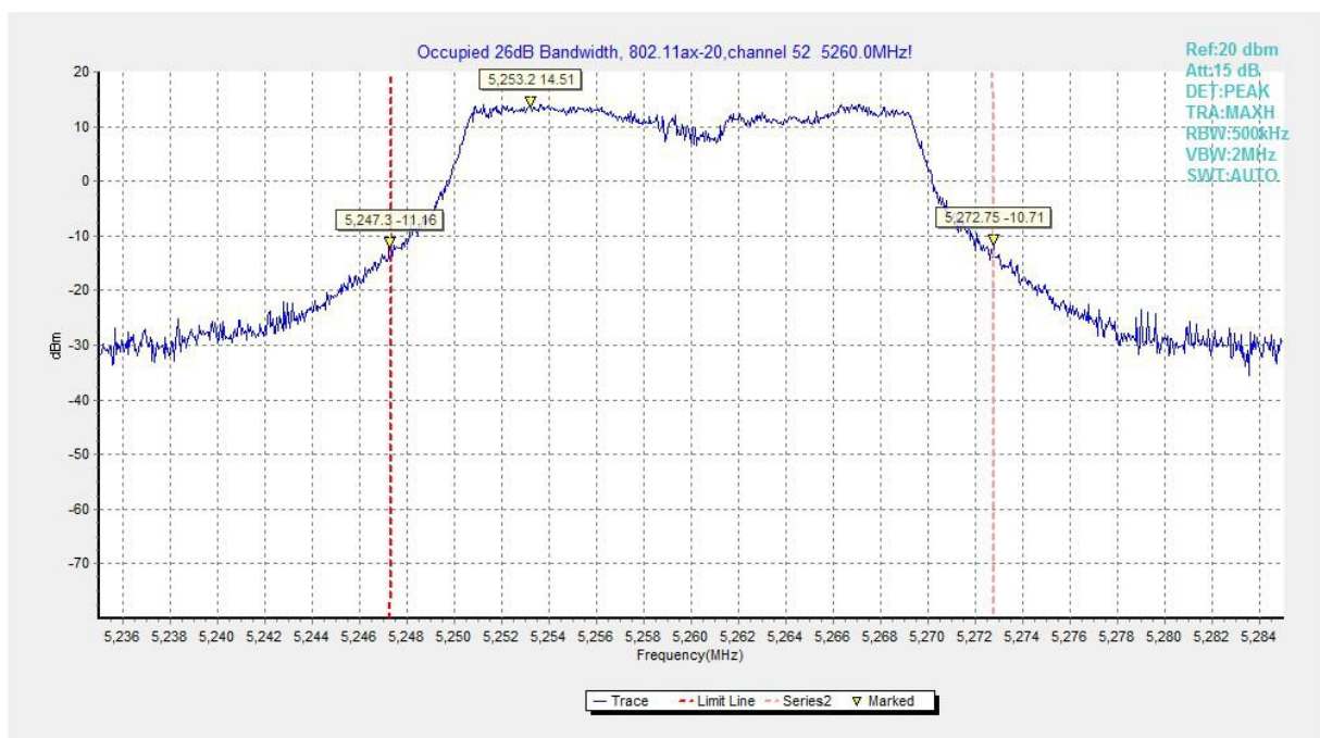
Fig.82 Occupied 26dB Bandwidth (802.11ax-HE20, 5260MHz)
