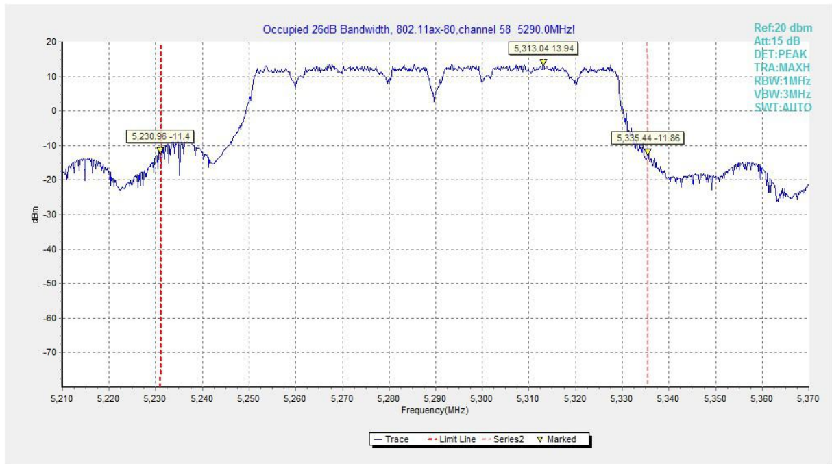
Fig.47 Occupied 26dB Bandwidth (802.11ax-HE80, 5290MHz)
