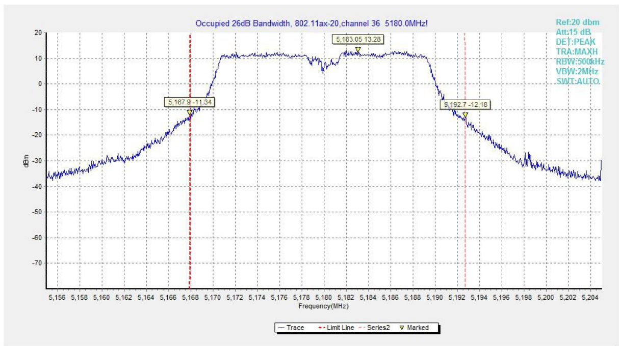
Fig.79 Occupied 26dB Bandwidth (802.11ax-HE20, 5180MHz)
