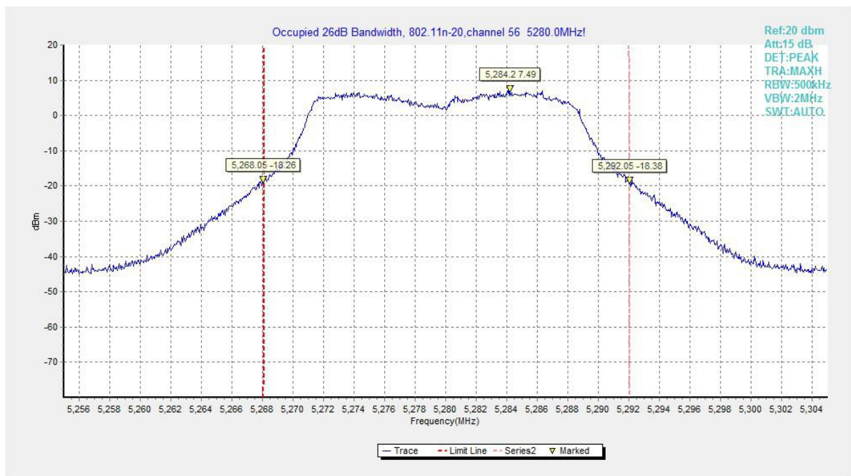
Fig.63 Occupied 26dB Bandwidth (802.11n-HT20, 5280MHz)
