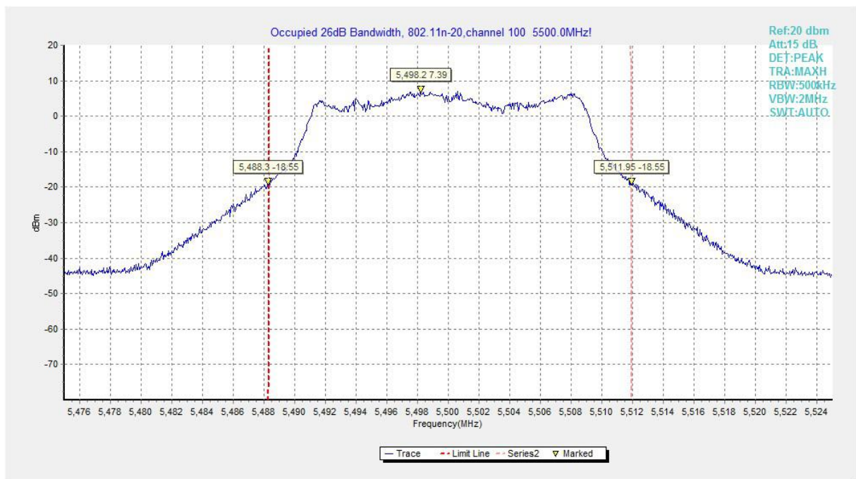
Fig.65 Occupied 26dB Bandwidth (802. 11n-HT20, 5500MHz)
