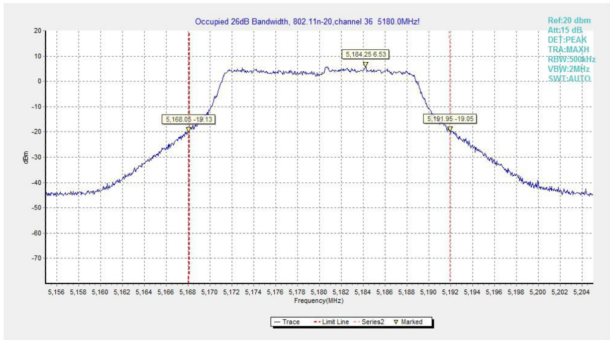
Fig.59 Occupied 26dB Bandwidth (802.11n-HT20, 5180MHz)
