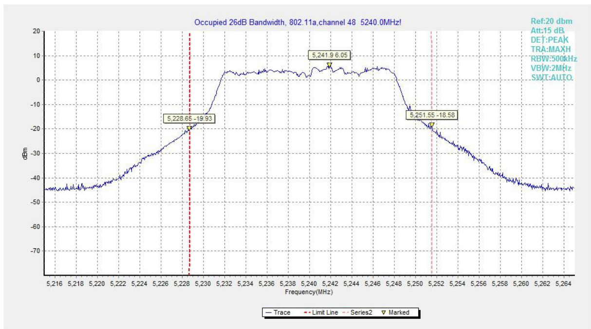
Fig.52 Occupied 26dB Bandwidth (802.11a, 5240MHz)
