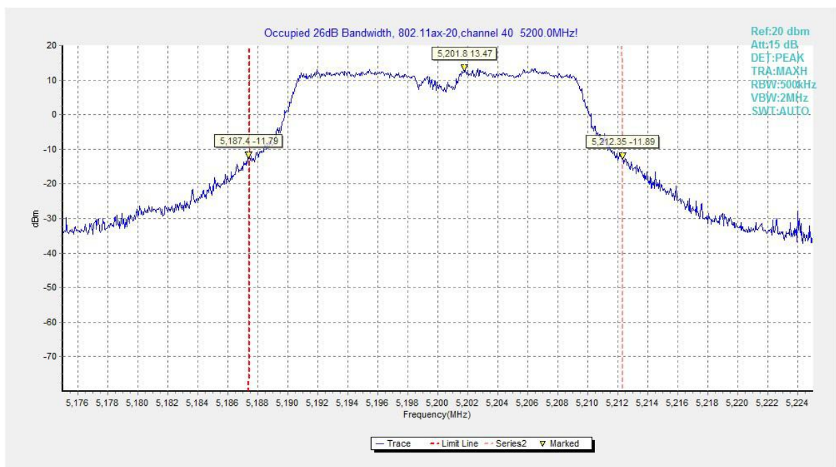
Fig.80 Occupied 26dB Bandwidth (802.11ax-HE20, 5200MHz)
