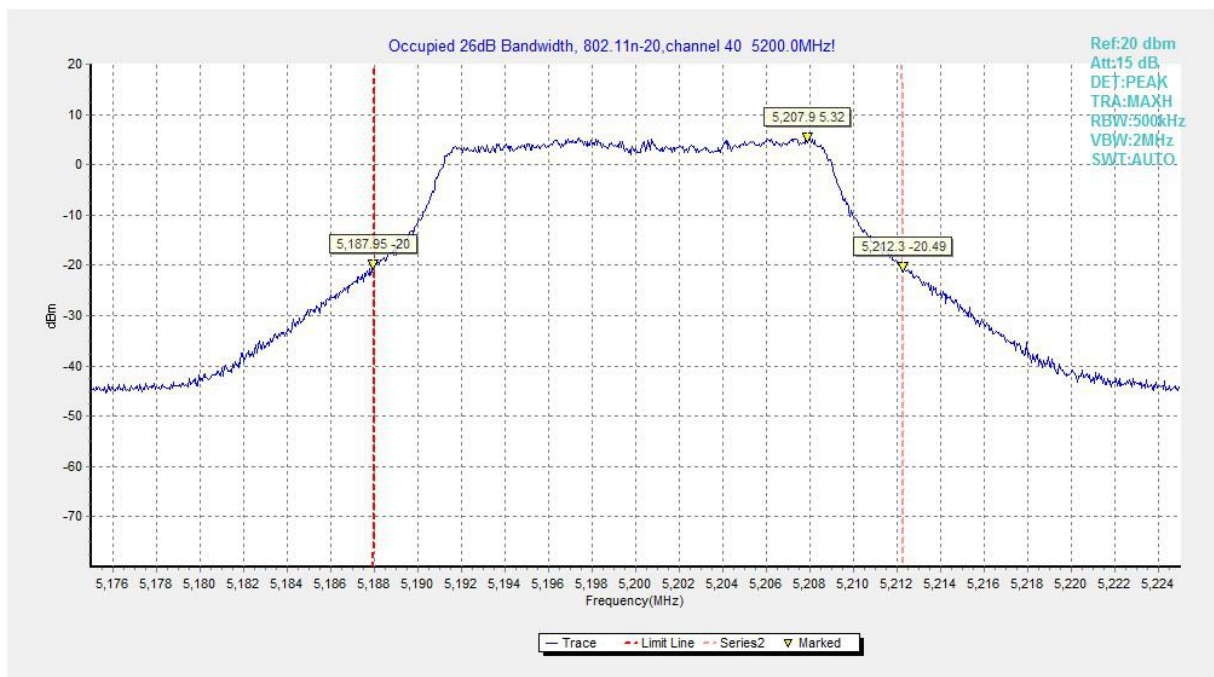
Fig.60 Occupied 26dB Bandwidth (802.11n-HT20, 5200MHz)
