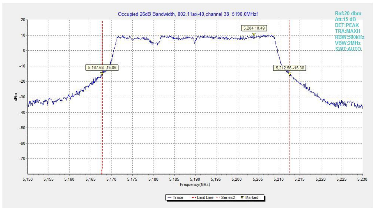
Fig.88 Occupied 26dB Bandwidth (802.11ax-HE40, 5190MHz)
