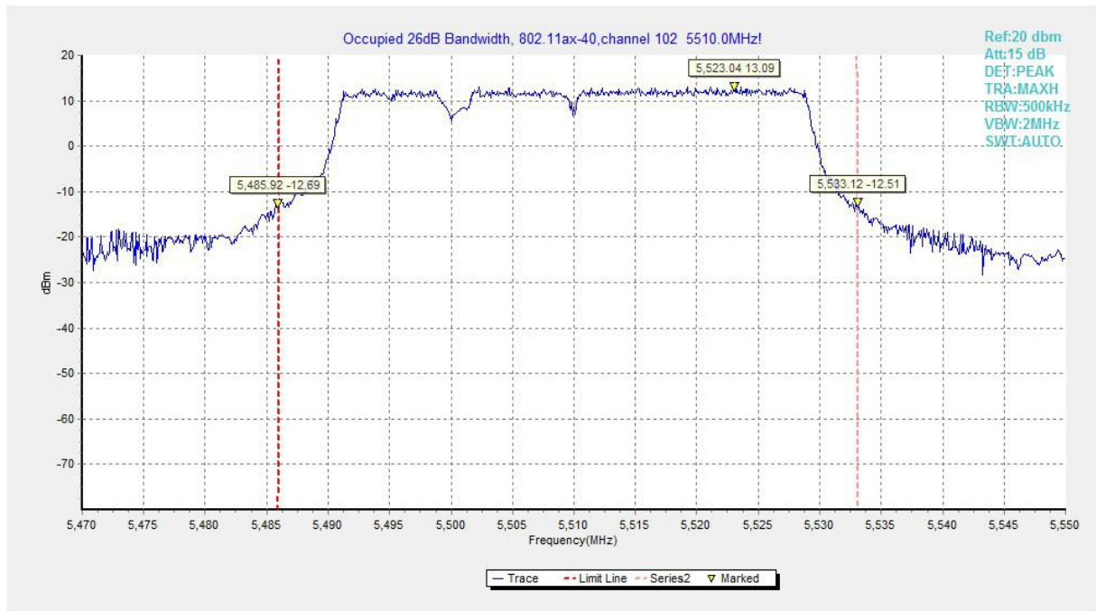
Fig.43 Occupied 26dB Bandwidth (802.11ax-HE40, 5510MHz)
