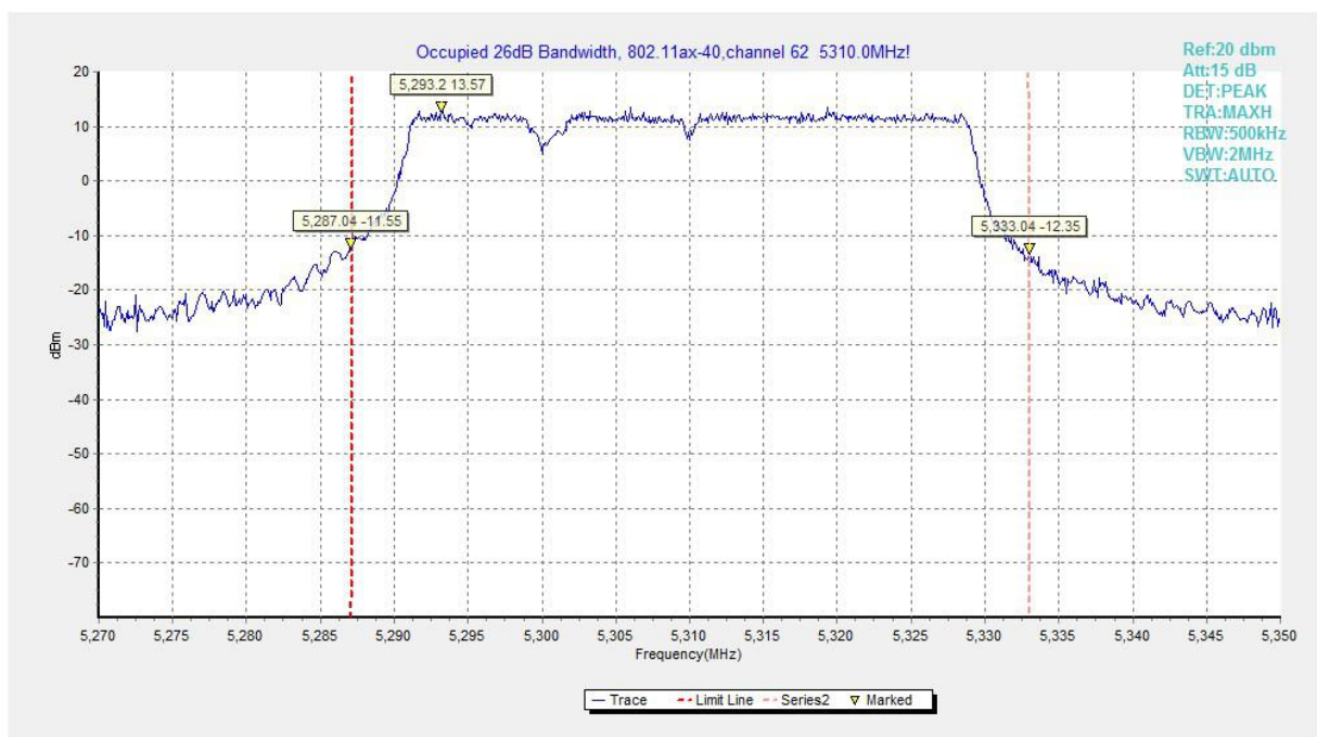
Fig.42 Occupied 26dB Bandwidth (802.11ax-HE40,5310MHz)
