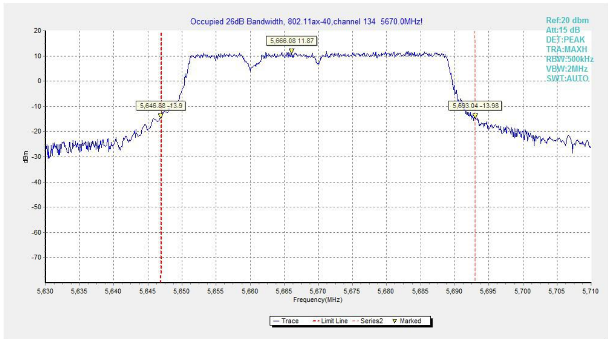
Fig.45 Occupied 26dB Bandwidth (802.11ax-HE40, 5670MHz)
