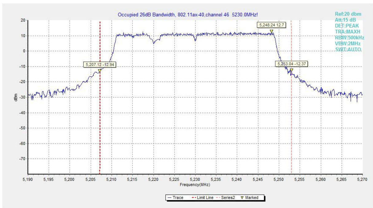
Fig.40 Occupied 26dB Bandwidth (802.11ax-HE40, 5230MHz)
