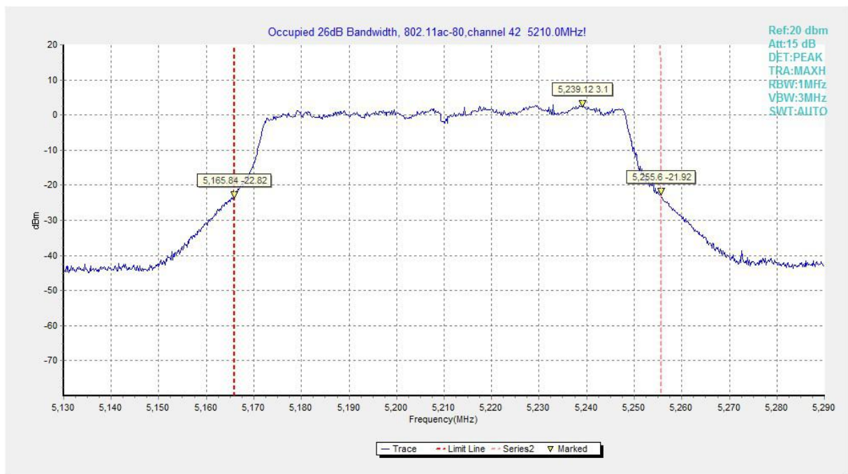
Fig.75 Occupied 26dB Bandwidth (802. 11ac-HT80, 5210MHz)
