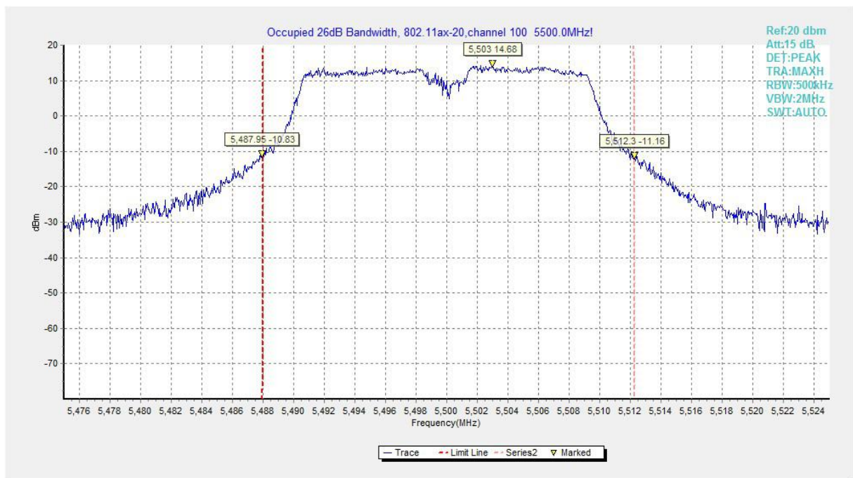
Fig.85 Occupied 26dB Bandwidth (802.11ax-HE20, 5500MHz)
