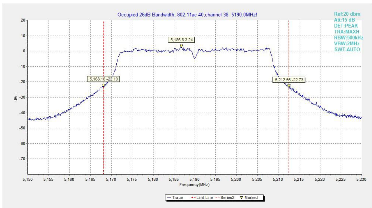
Fig.68 Occupied 26dB Bandwidth (802.11ac-HT40, 5190MHz)
