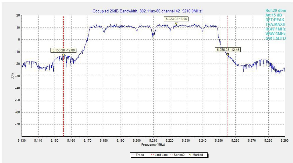
Fig.46 Occupied 26dB Bandwidth (802.11ax-HE80,5210MHz)
