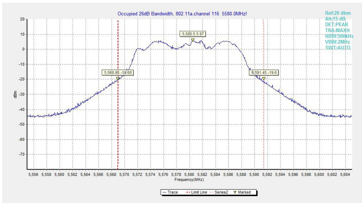
Fig.57 Occupied 26dB Bandwidth (802.11a, 5580MHz)
