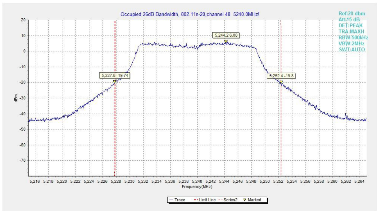
Fig.61 Occupied 26dB Bandwidth (802.11n-HT20, 5240MHz)
