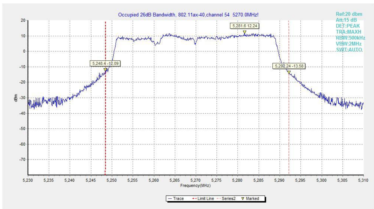
Fig.90 Occupied 26dB Bandwidth (802.11ax-HE40, 5270MHz)
