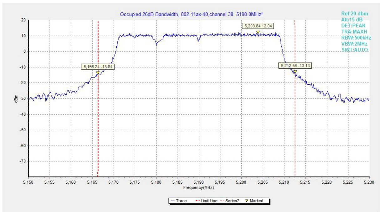
Fig.39 Occupied 26dB Bandwidth (802.11ax-HE40, 5190MHz)
