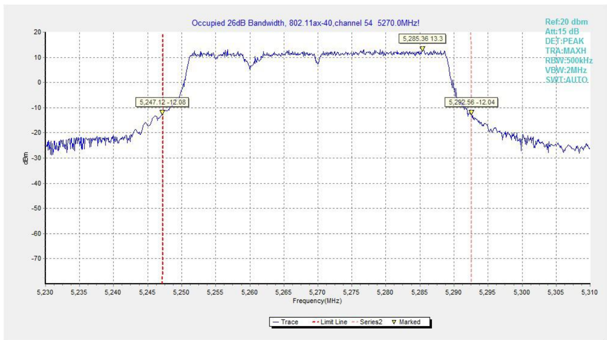
Fig.41 Occupied 26dB Bandwidth (802.11ax-HE40, 5270MHz)
