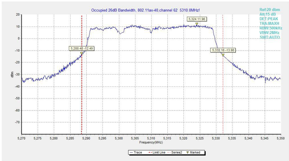
Fig.91 Occupied 26dB Bandwidth (802.11ax-HE40,5310MHz)
