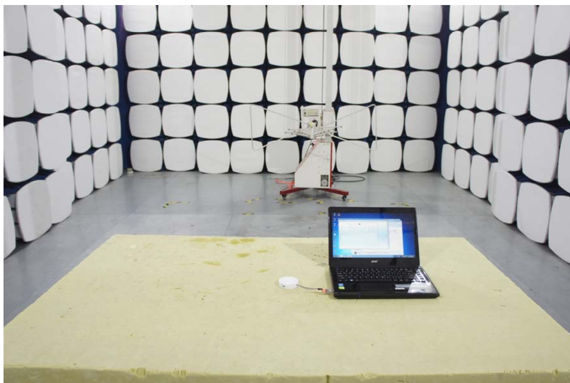
Radiated Setup photo (30M-1G)
