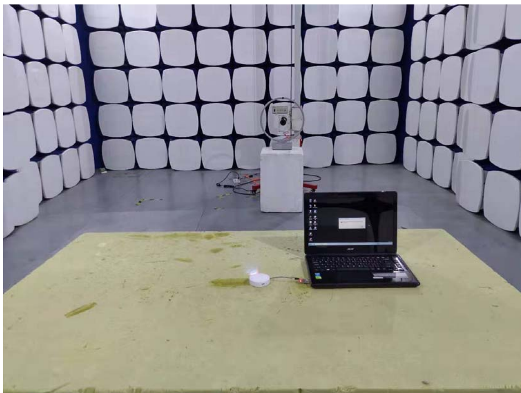
Radiated Setup photo (9k-30M)
