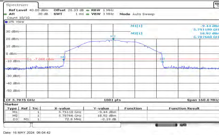
SRD 80M Ant1 5787.5
