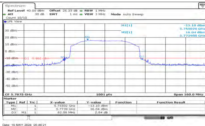
SRD 60M Ant1 5787.5
