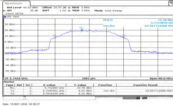
SRD 40M Ant0 5745.5
