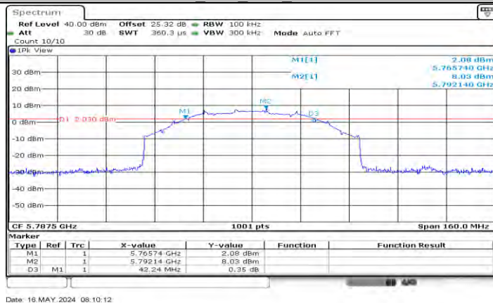
SRD 80M Ant0 5787.5
