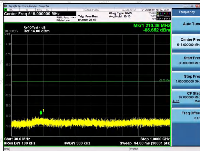
11N20MIMO-Ant1-2462-30~1000-PASS
