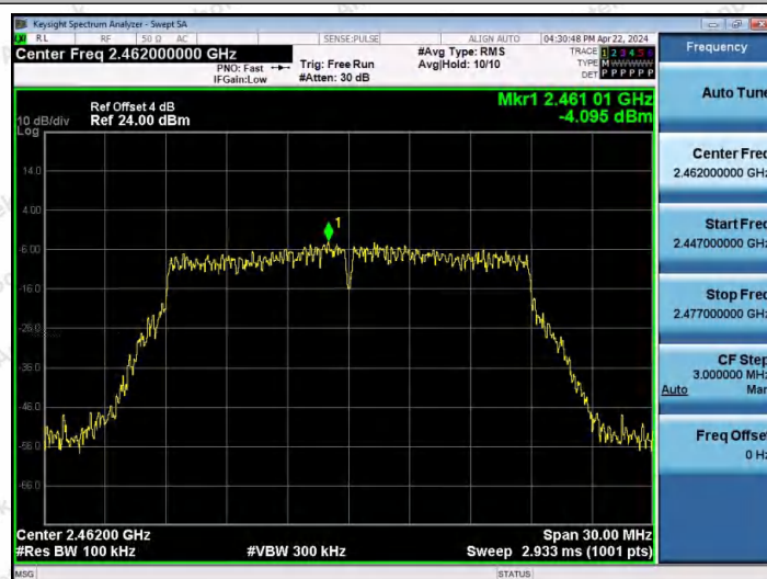
11N20MIMO-Ant2-2462-0~Reference-PASS
