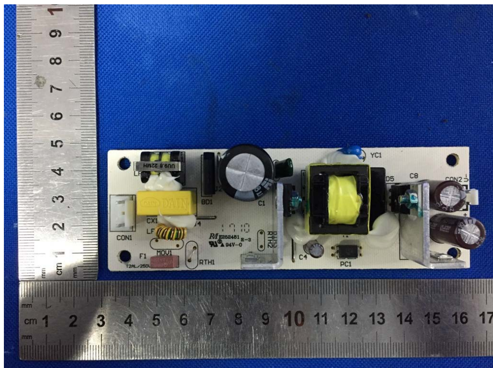
Built-in AC adapter: JFY40A-160250
