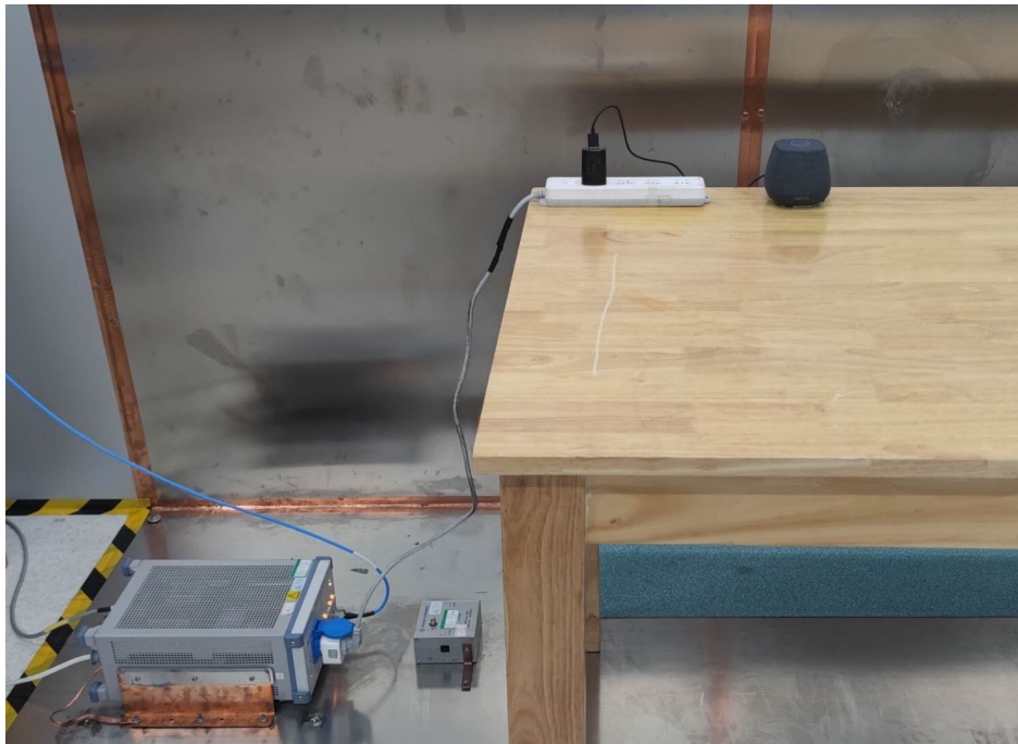
Photograph 3: Set-up for Conducted Emission on AC Mains
