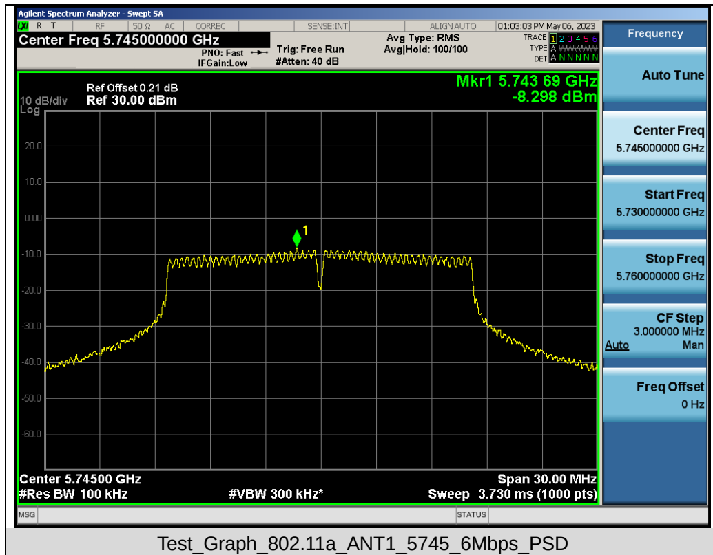
Test Graphs of Conducted Output Power Spectral Density for band 5.725-5.85 GHz-Ant 1
