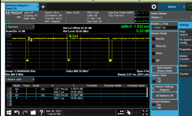
802.11ac-VHT40(T=5.390ms)
