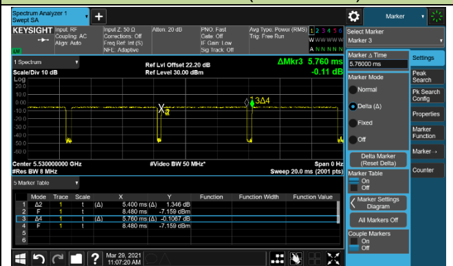
802.11ac-VHT80(T=5.400ms)
