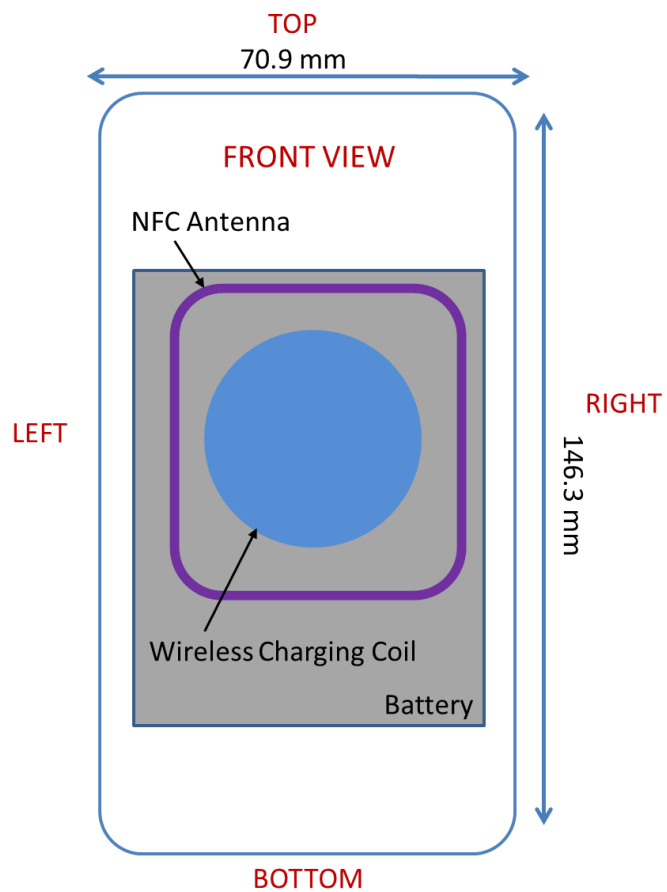
Figure K-2 NFC Antenna Locations
