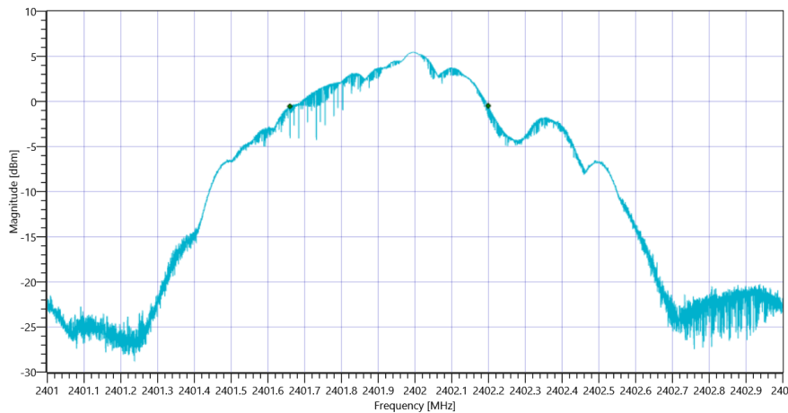
Plot_FCC Part 15.247 Maximum Peak Conducted Output Power DTS ~ BT LE 1 Msps DTS BW_02082021_143856.png
