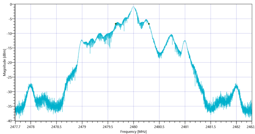
Plot_FCC Part 15.247 Maximum Peak Conducted Output Power DTS ~ BT LE 2 Msps DTS BW_02082021_163859.png
