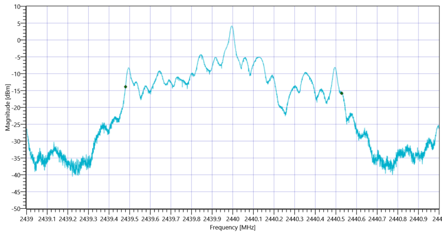
Plot_FCC Part 15.247 Bandwidth 99PCT-20dB ~ BT LE 1 Msps 99PCT_02082021_145320.png
