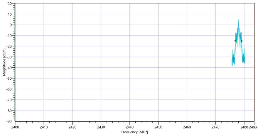
Plot_FCC Part 15.247 Bandwidth 99PCT-20dB ~ BT LE 2 Msps 20dB_02082021_171446.png
