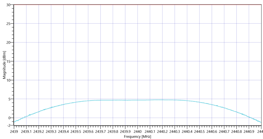
Plot_FCC Part 15.247 Maximum Peak Conducted Output Power DTS ~ BT LE 1 Msp_02082021_145126.png
