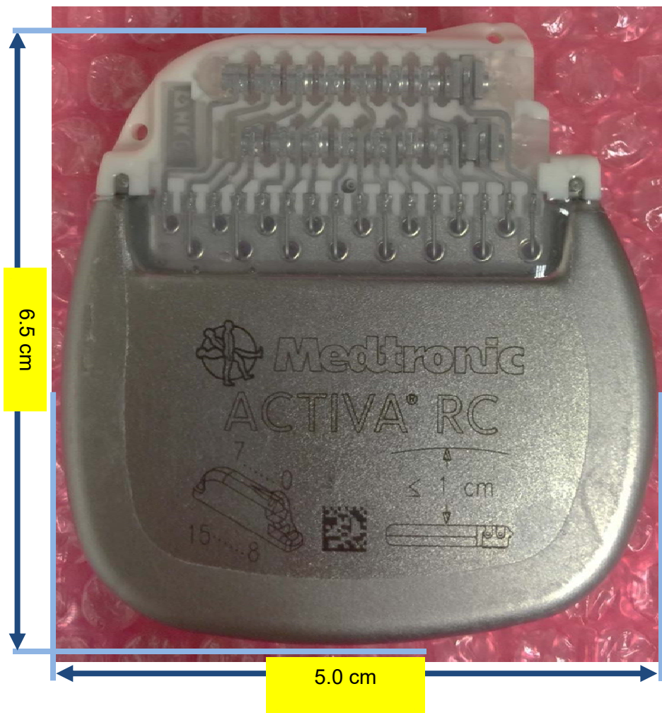
Figure 1: ACTIVA® RC, Model: 37612, Front View (with dimensions)
