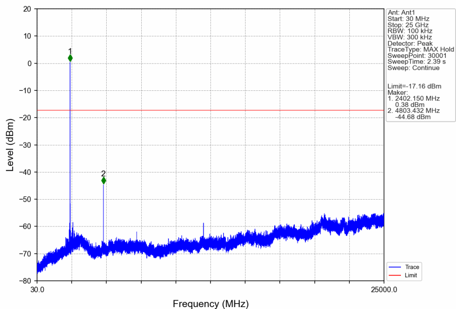
GFSK_LCH_2402MHz_Ant1_NTNV
