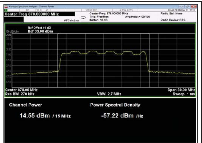
Figure 27: 16QAM 15MHz B.W.; 878.0MHz, 30kHz
