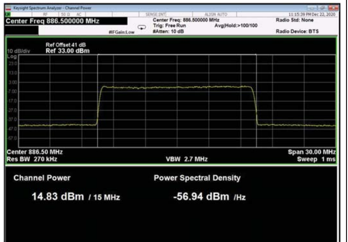
Figure 71: 64QAM 15MHz B.W.; 886.5MHz, 15kHz
