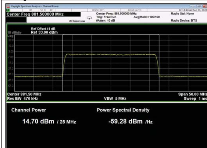
Figure 132: 256QAM 25MHz B.W.; 881.5MHz, 30kHz
