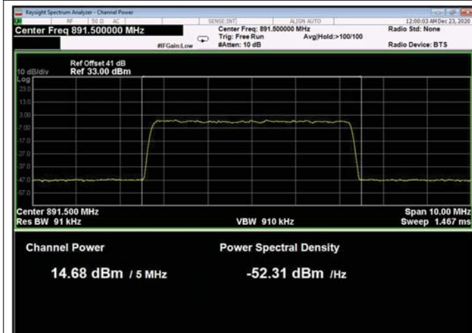
Figure 96: 256QAM 5MHz B.W.; 891.5MHz, 15kHz
