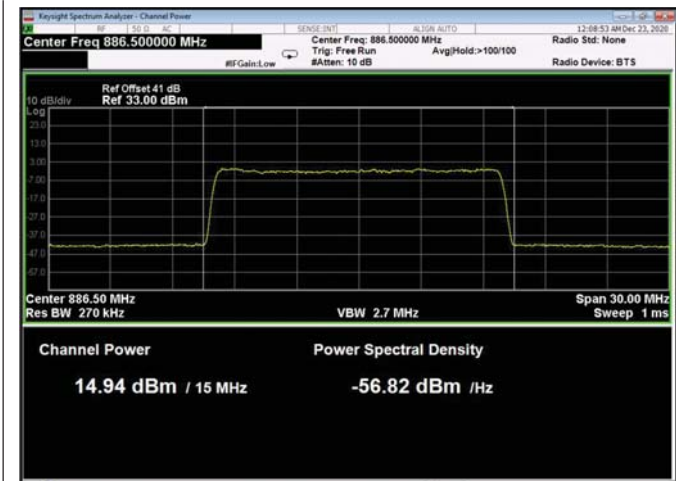
Figure 114: 256QAM 15MHz B.W.; 886.5MHz, 30kHz
