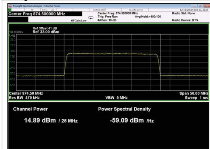
Figure 126: 256QAM 25MHz B.W.; 874.5MHz, 30kHz
