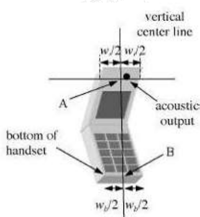
F-2. Handset vertical and horizontal reference lines-“clam-shell case”
