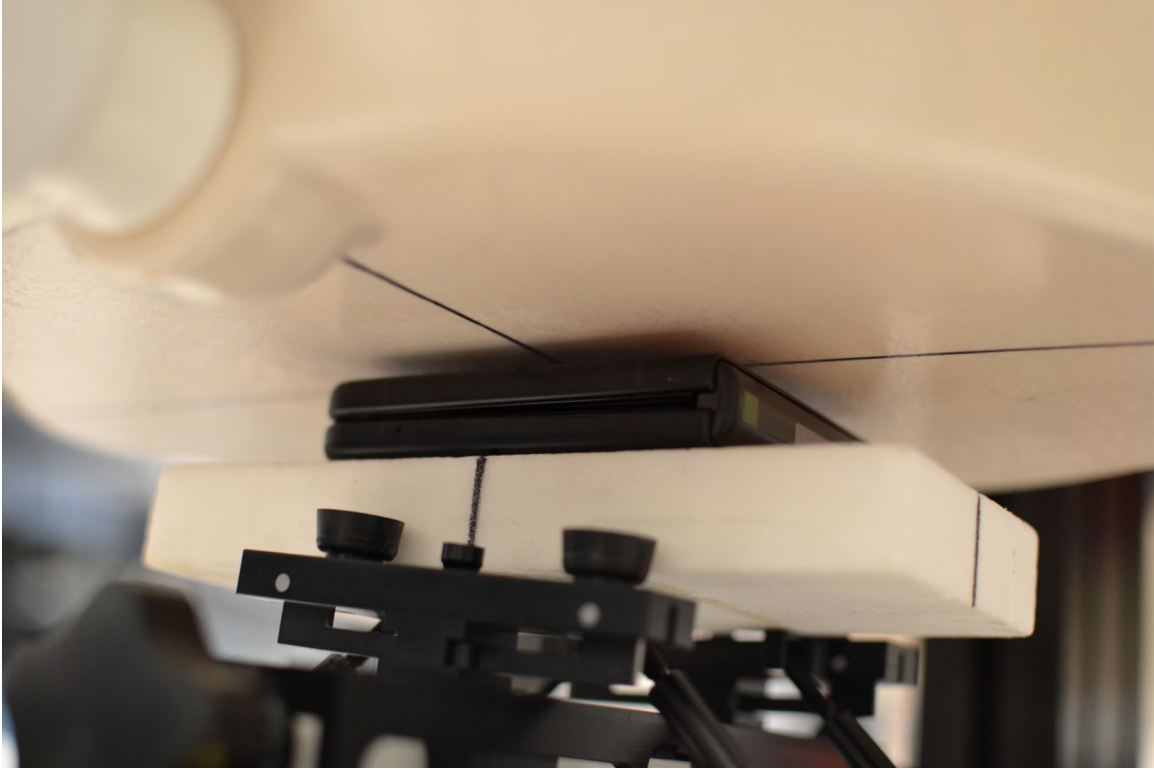
SAR Test Setup Photo 24 – Closed Hotspot, Front Side, 5 mm
