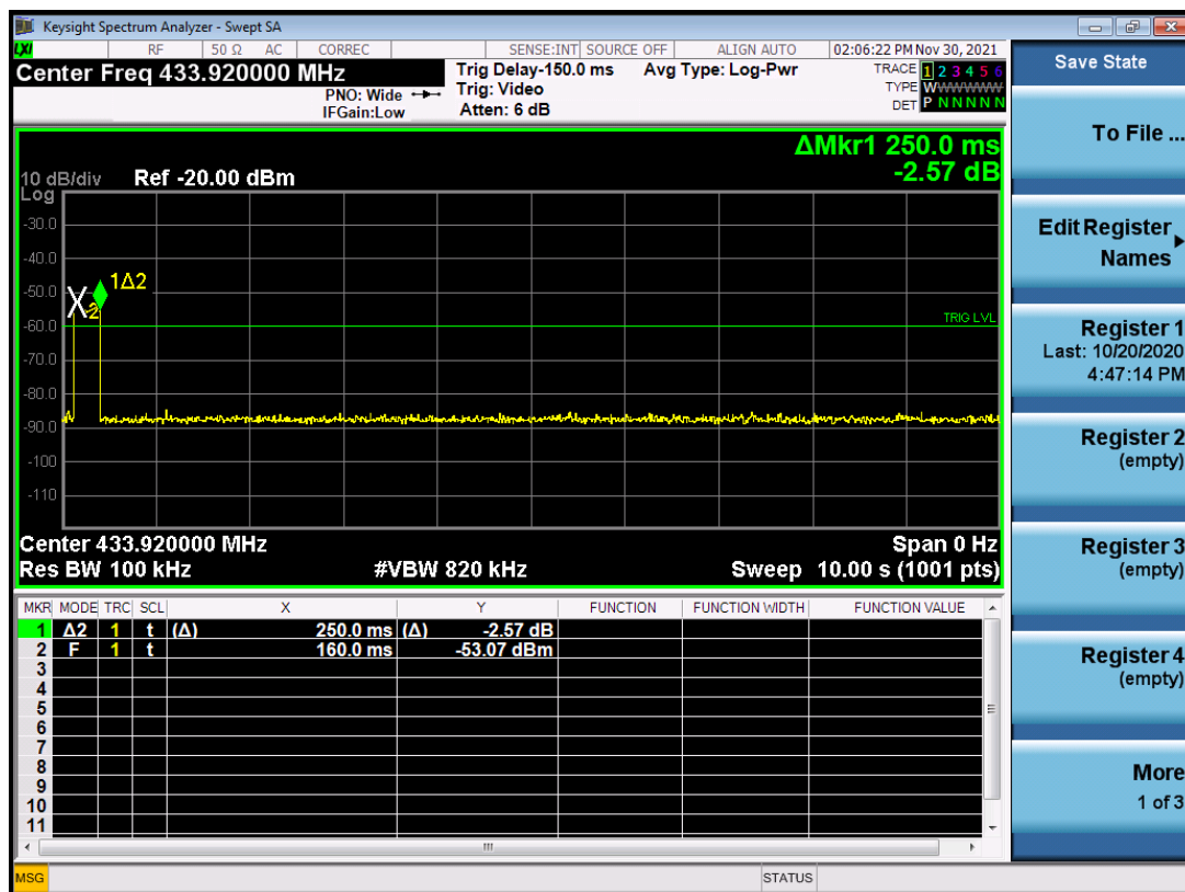
Figure 2: Deactivation Time
