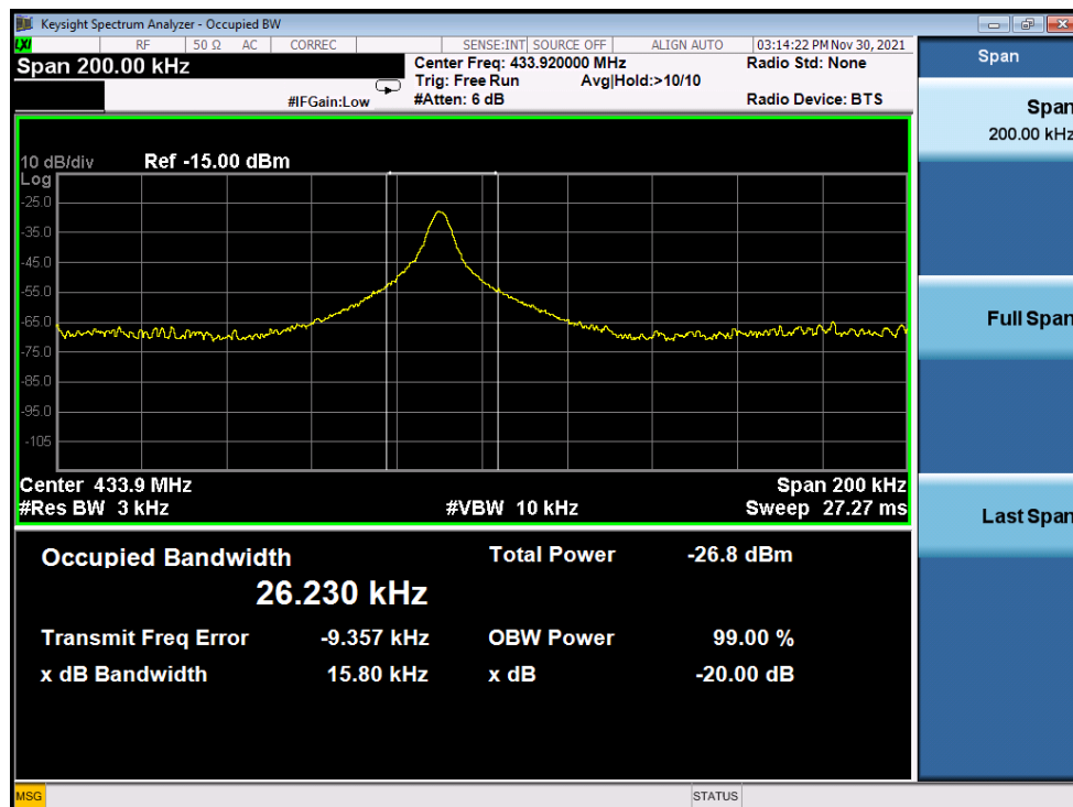
Figure 1: 20dB Bandwidth
