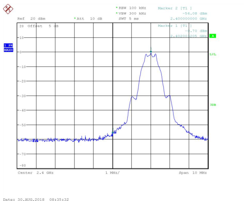
Fig.10 Frequency Band Edge: GFSK, Ch0
