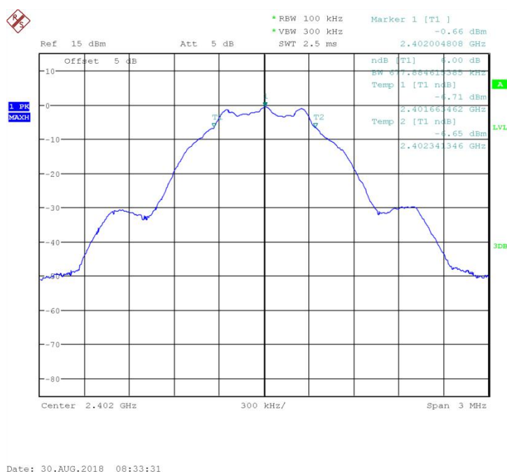
Fig.7 6dB Bandwidth: Ch0
