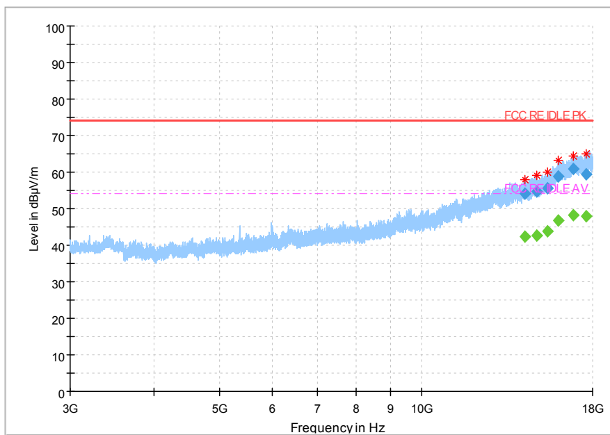
Fig.29 Radiated emission: Ch0, 3GHz~18GHz
