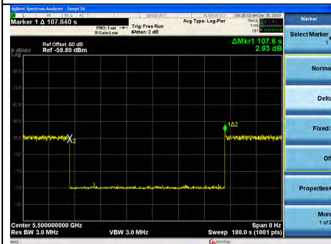
Initial CAC – HT20 – 5500MHz
