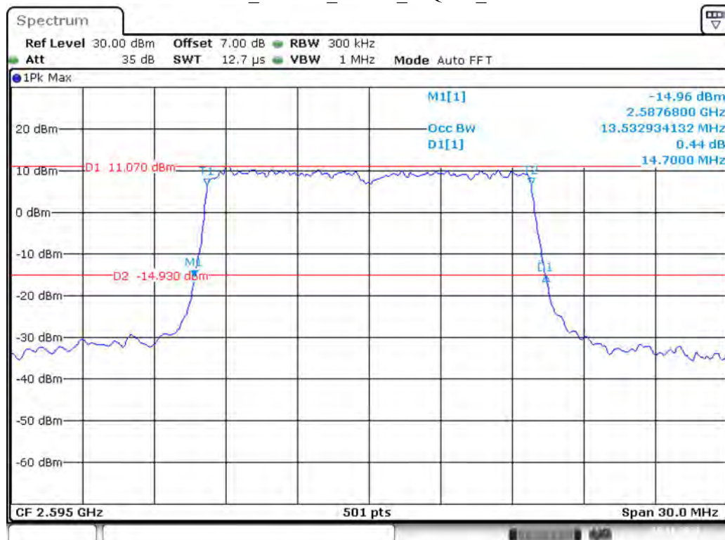
Band 41_15 MHz_Middle_16QAM_RB75#0
