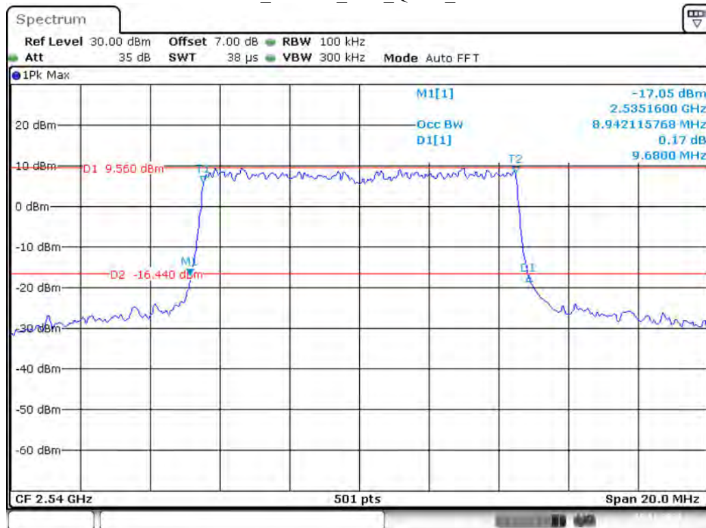
Band 41_10 MHz_Low_QPSK_RB50#0
