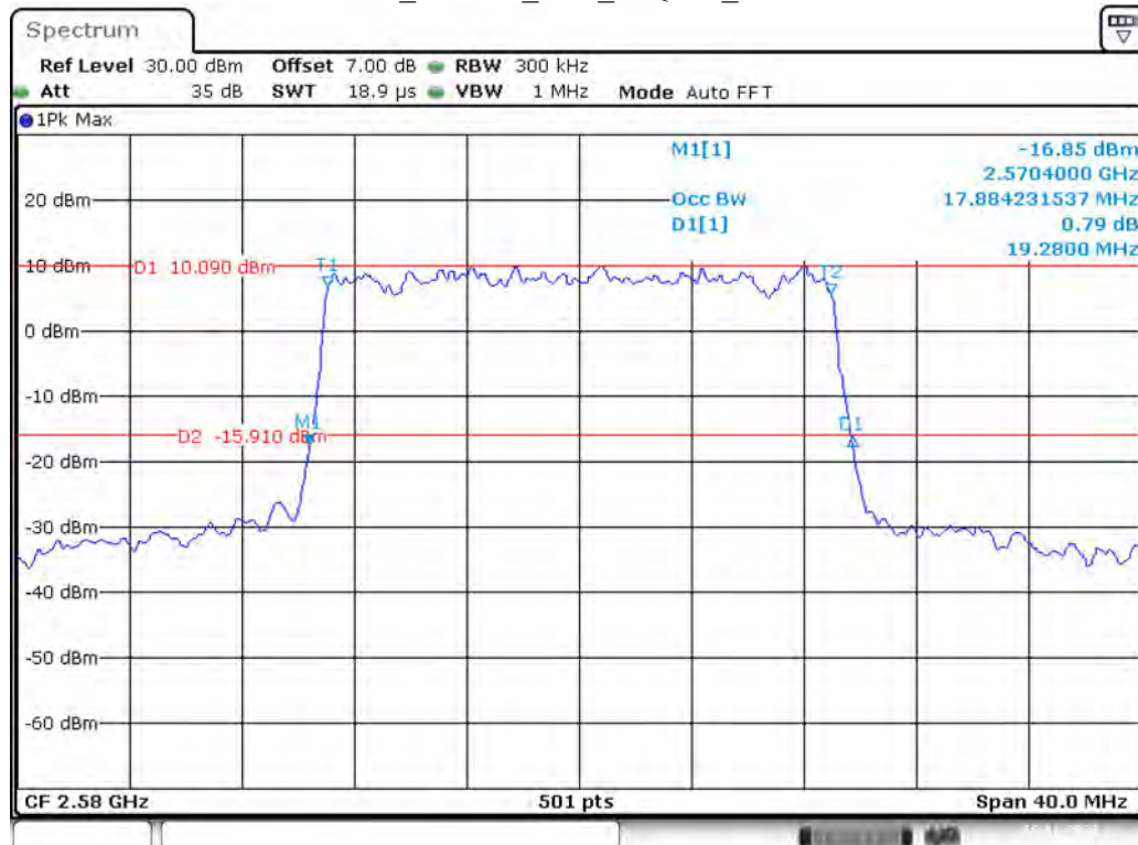
Band 38_20 MHz_Low_16QAM_RB100#0
