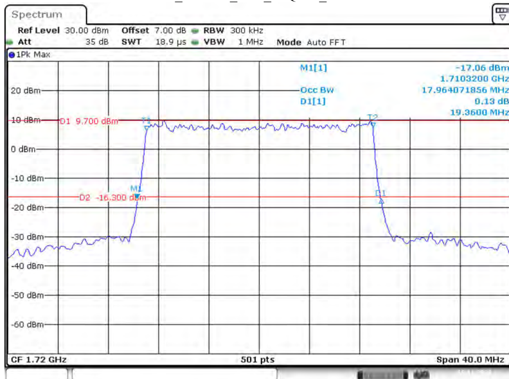
Band 4_20 MHz_Low_16QAM_RB100#0
