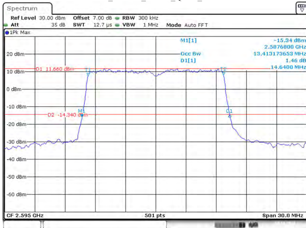
Band 41_15 MHz_Middle_QPSK_RB75#0
