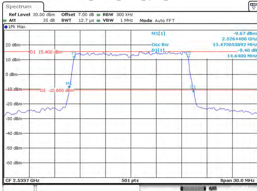
Band 7_15 MHz_Middle_QPSK_RB75#0
