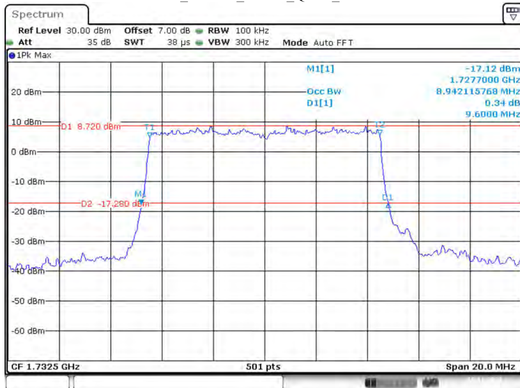
Band 4_10 MHz_Middle_QPSK_RB50#0
