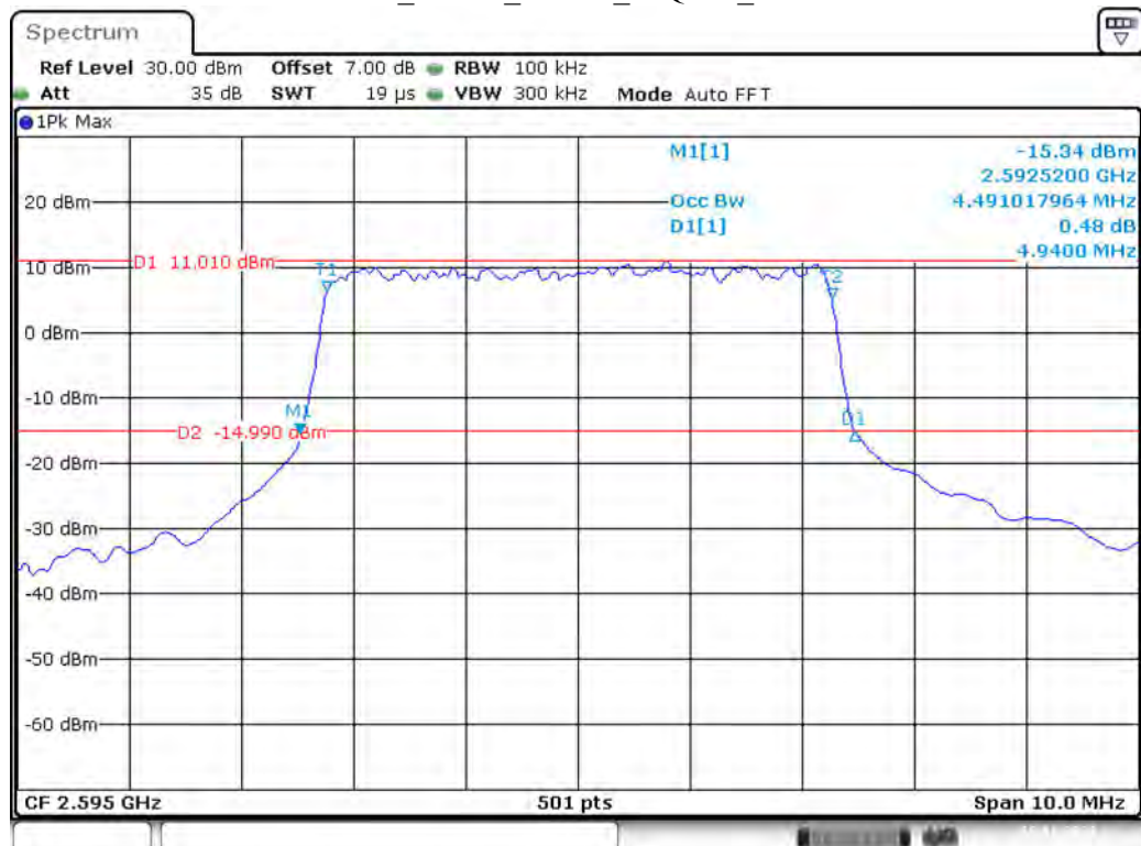
Band 38_5 MHz_Middle_16QAM_RB25#0
