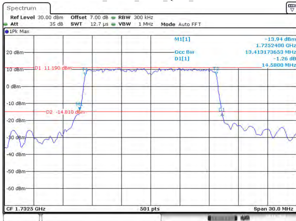
Band 4_15 MHz_Middle_QPSK_RB75#0
