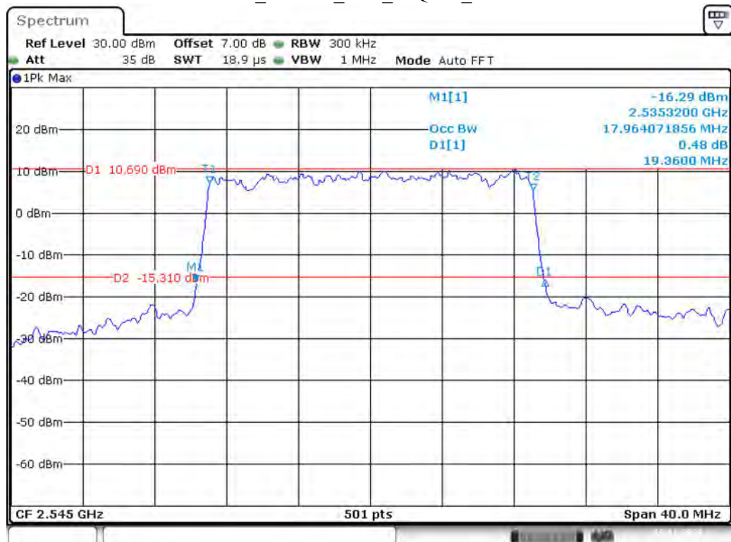
Band 41_20 MHz_Low_16QAM_RB100#0
