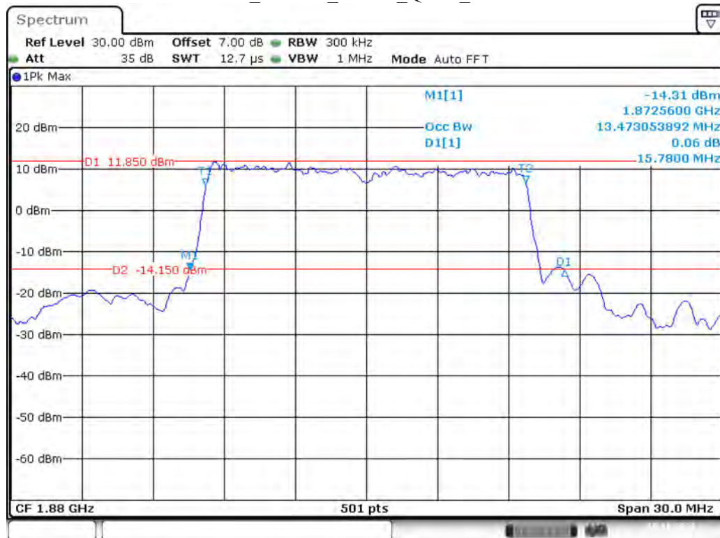
Band 2_15 MHz_Middle_QPSK_RB75#0
