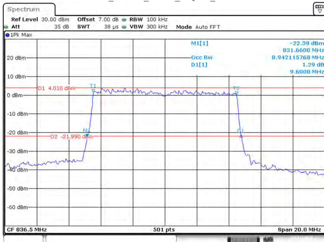
Band 5_10 MHz_Middle_16QAM_RB50#0
