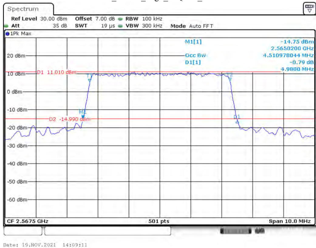
Band 7_5 MHz_High_16QAM_RB25#0
