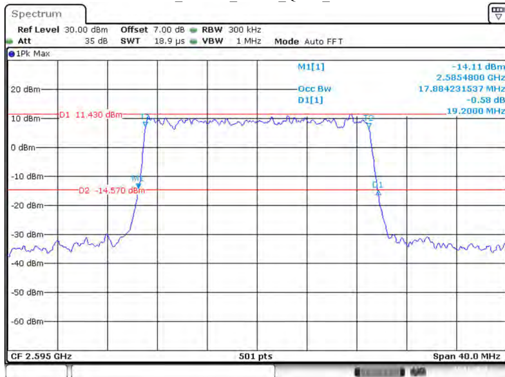
Band 38_20 MHz_Middle_QPSK_RB100#0
