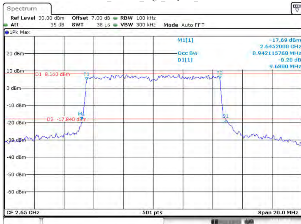
Band 41_10 MHz_High_16QAM_RB50#0
