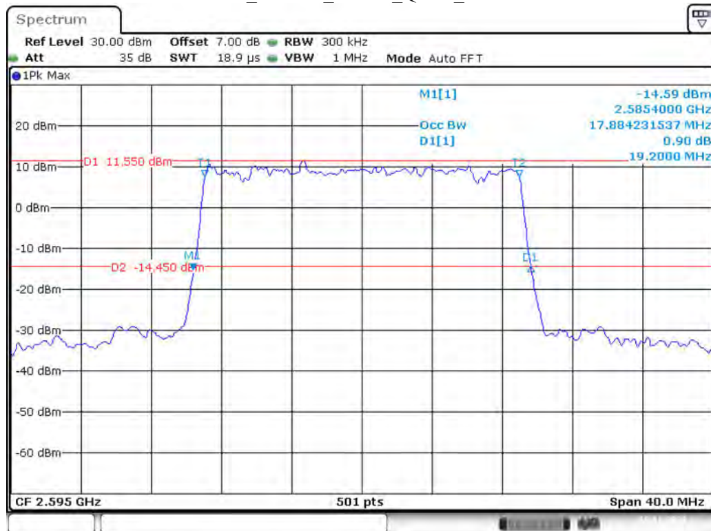
Band 41_20 MHz_Middle_QPSK_RB100#0
