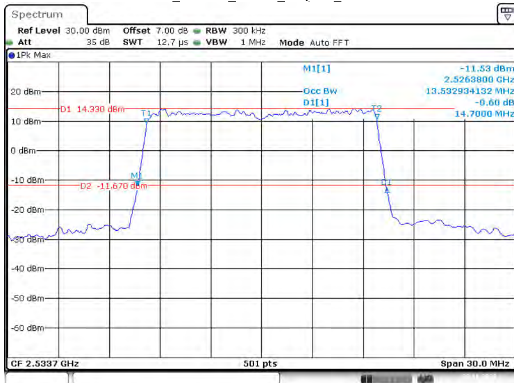
Band 7_15 MHz_Middle_16QAM_RB75#0
