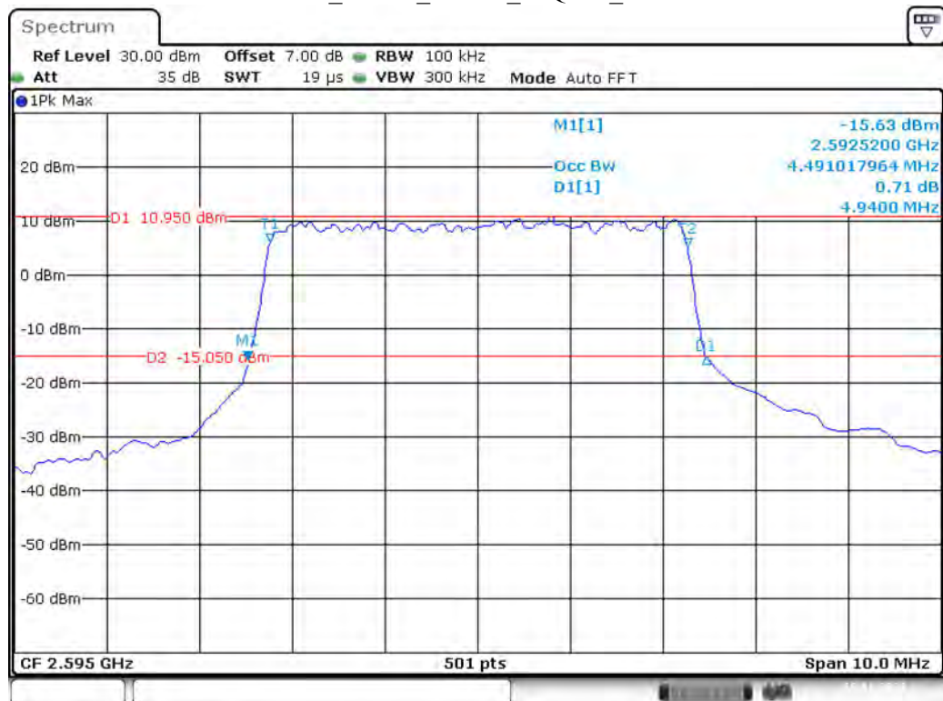
Band 41_5 MHz_Middle_16QAM_RB25#0
