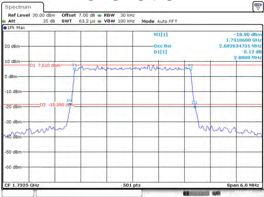
Band 4_3 MHz_Middle_16QAM_RB15#0
