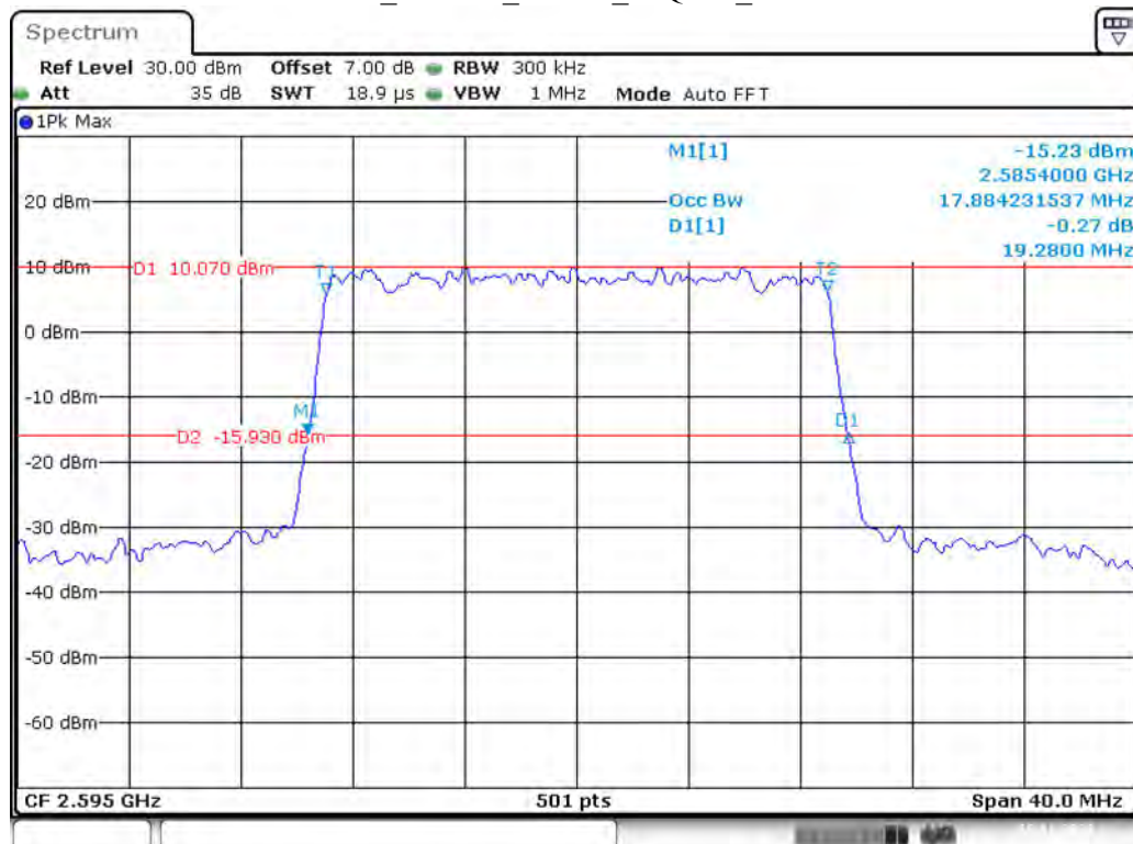
Band 38_20 MHz_Middle_16QAM_RB100#0
