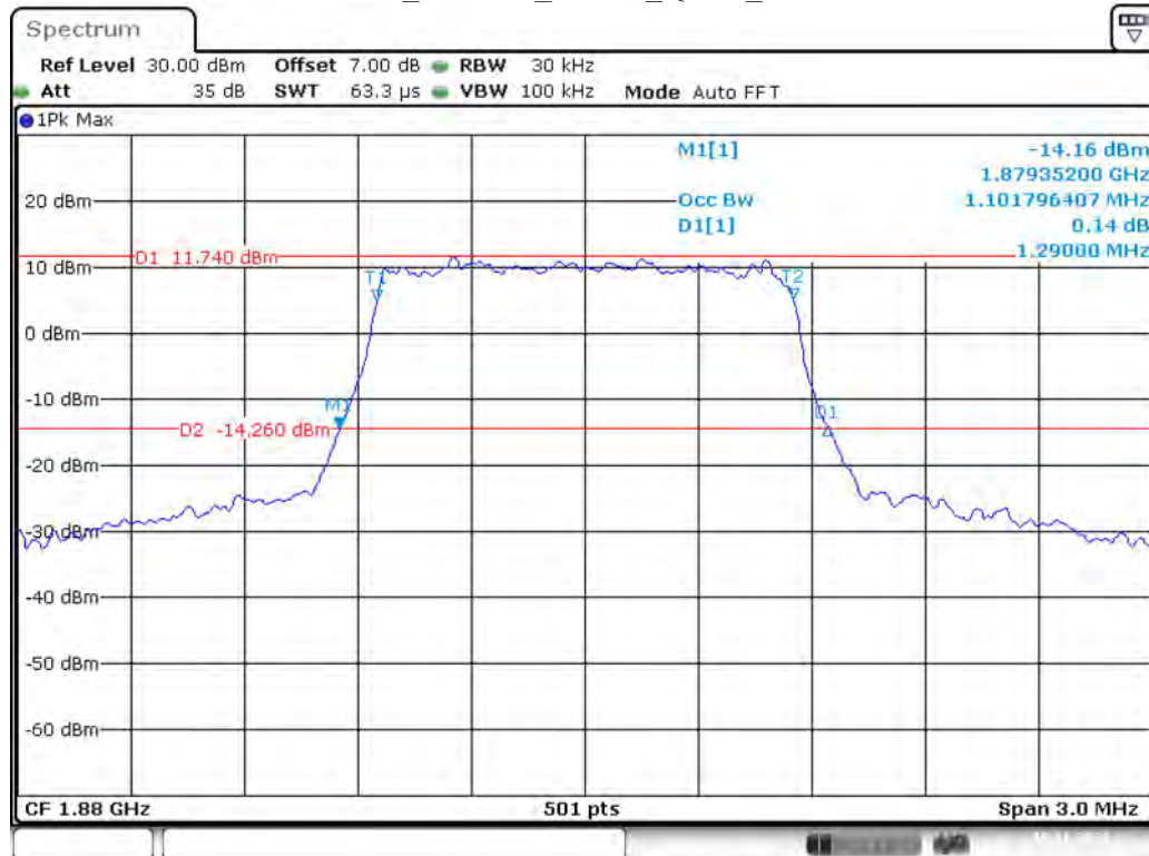
Band 2_1.4 MHz_Middle_QPSK_RB6#0
