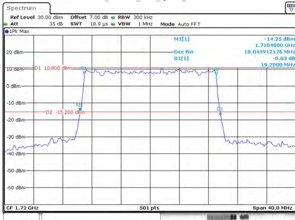
Band 4_20 MHz_Low_QPSK_RB100#0
