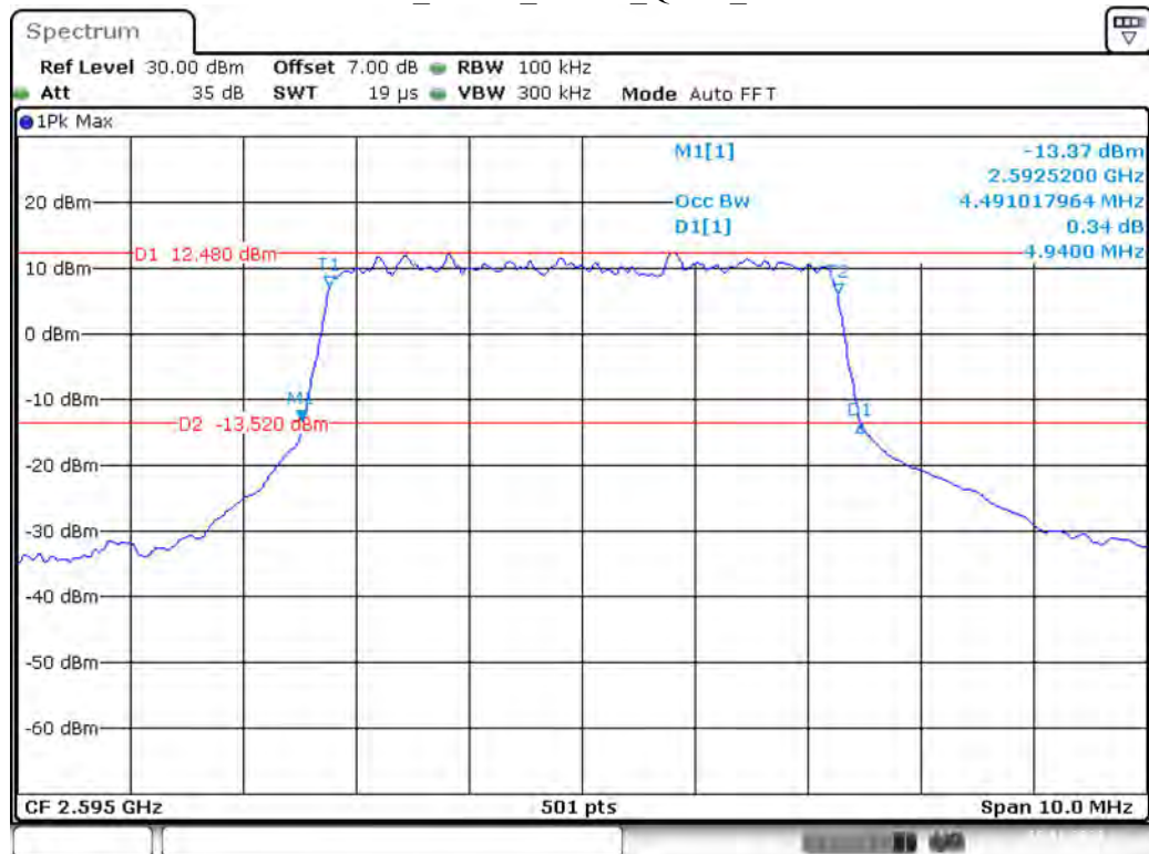
Band 38_5 MHz_Middle_QPSK_RB25#0
