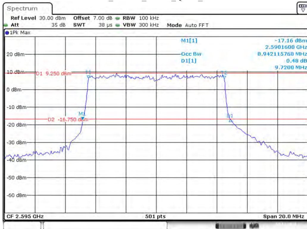
Band 38_10 MHz_Middle_QPSK_RB50#0
