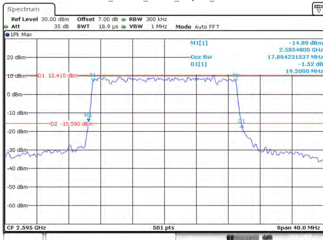
Band 41_20 MHz_Middle_16QAM_RB100#0
