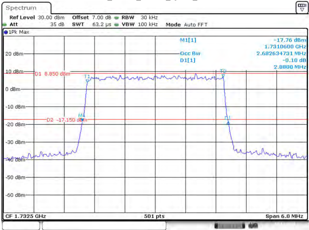
Band 4_3 MHz_Middle_QPSK_RB15#0
