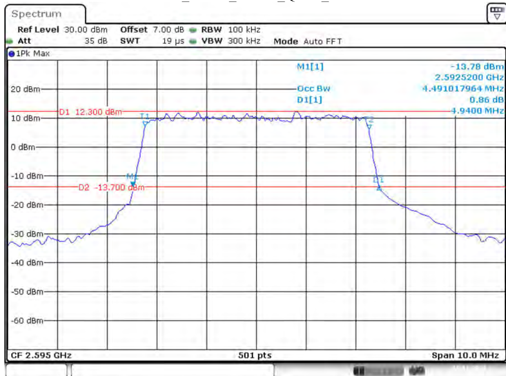
Band 41_5 MHz_Middle_QPSK_RB25#0
