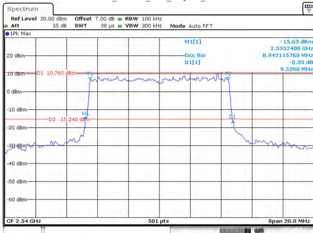
Band 41_10 MHz_Low_16QAM_RB50#0
