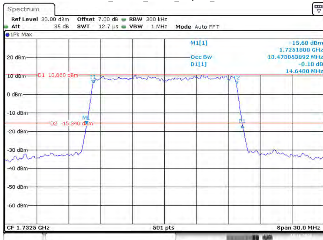
Band 4_15 MHz_Middle_16QAM_RB75#0
