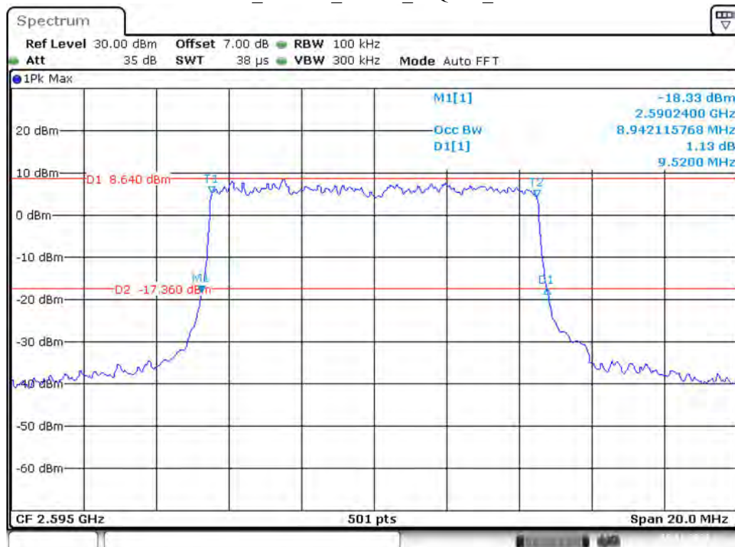
Band 38_10 MHz_Middle_16QAM_RB50#0
