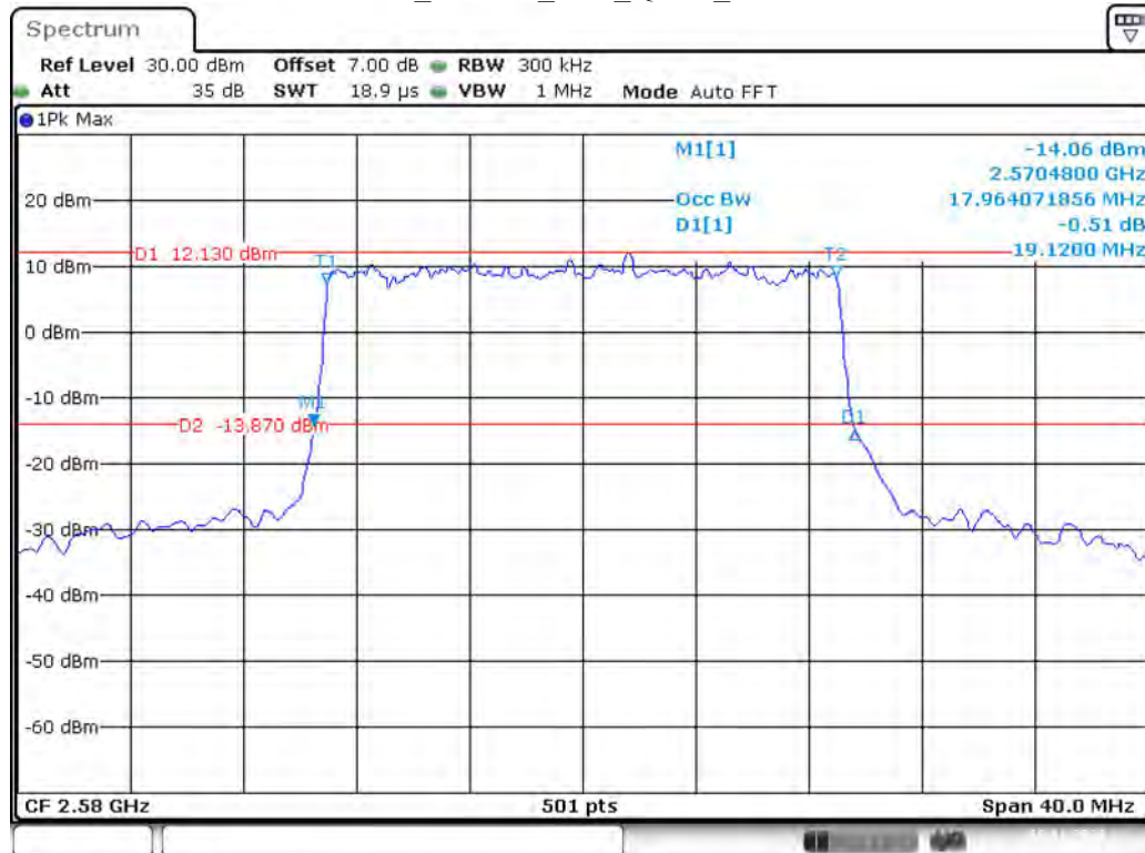
Band 38_20 MHz_Low_QPSK_RB100#0
