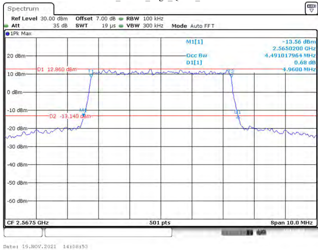
Band 7_5 MHz_High_QPSK_RB25#0
