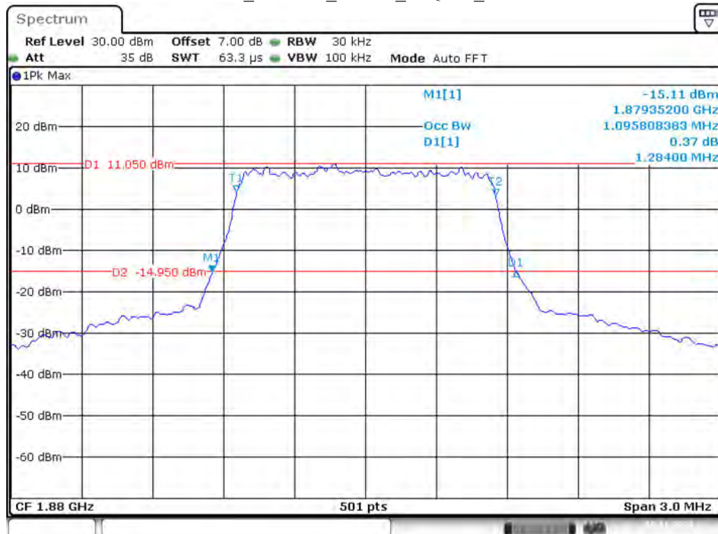
Band 2_1.4 MHz_Middle_16QAM_RB6#0
