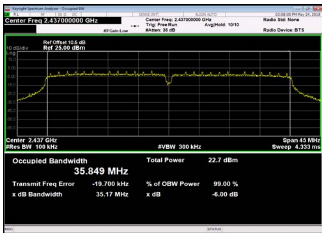
802.11n(HT40),2437MHz,
