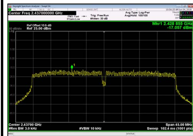
Power spectral density-802.11n(HT40) ,2437MHz,
