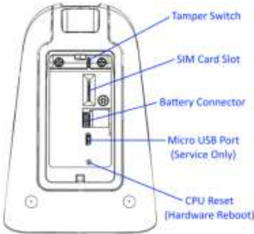
Smart Hub Lite (bottom view open) —
