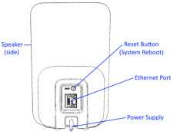
Smart Hub Lite (back view) —
